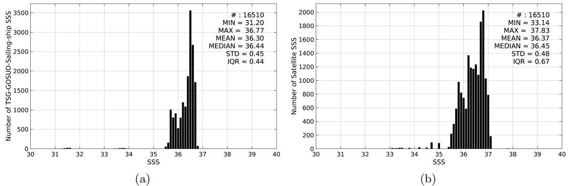
Figure 2: Histograms of SSS from TSG-GOSUD-Sailing-ship (a) and SMAP-L3-RSS-V2-MONTHLY-0.25DEG-40KM (b) considering all match-up pairs per bins of 0.1 over the Mid-Low Latitudes 45N-45S Pi-MEP region and for the full satellite product period.
