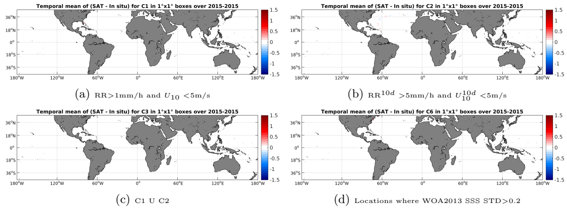
Figure 12: Temporal mean gridded over spatial boxes of size 1^\circ \times 1^\circ of \Delta SSS (SMAP-L3-RSS-V2-MONTHLY-0.25DEG-40KM - TSG-GOSUD-Sailing-ship) for 4 different subdatasets corresponding to: RR > 1\text{mm/h} and U_{10} < 5\text{m/s} (a), RR^{10d} > 5\text{mm/h} and U_{10}^{10d} < 5\text{m/s} (b), C1 U C2 (c), Locations where WOA2013 SSS STD > 0.2 (d).
