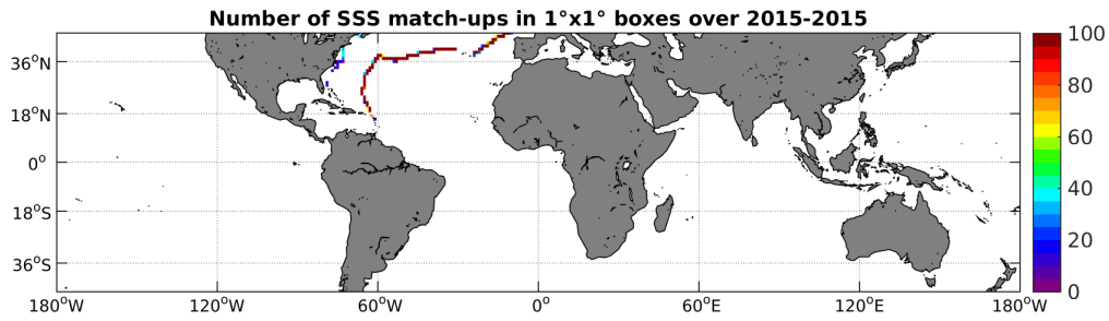
Figure 4: Number of SSS match-ups between TSG-GOSUD-Sailing-ship SSS and the SMAP-L3-RSS-V2-MONTHLY-0.25DEG-40KM SSS product for the Mid-Low Latitudes 45N-45S Pi-MEP region over 1°x1° boxes and for the full satellite product period.
