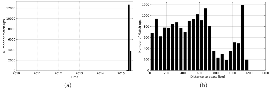
Figure 1: Number of match-ups between TSG-GOSUD-Sailing-ship and SMAP-L3-RSS-V2-MONTHLY-0.25DEG-40KM SSS as a function of time (a) and as function of the distance to coast (b) over the Mid-Low Latitudes 45N-45S Pi-MEP region and for the full satellite product period.
