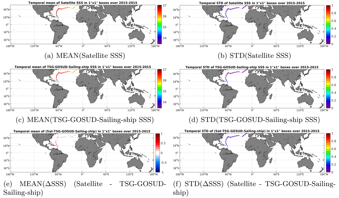
Figure 6: Temporal mean (left) and STD (right) of SSS from SMAP-L3-RSS-V2-MONTHLY-0.25DEG-40KM (top), TSG-GOSUD-Sailing-ship (middle), and of \Delta SSS (Satellite - TSG-GOSUD-Sailing-ship). Only match-up pairs are used to generate these maps.
