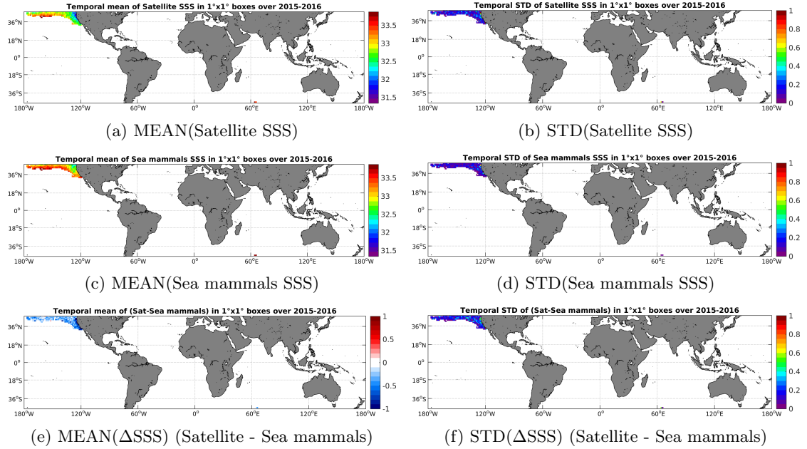
Figure 6: Temporal mean (left) and STD (right) of SSS from SMAP-L3-RSS-V2-MONTHLY-0.25DEG-40KM (top), Sea mammals (middle), and of \Delta SSS (Satellite - Sea mammals). Only match-up pairs are used to generate these maps.
