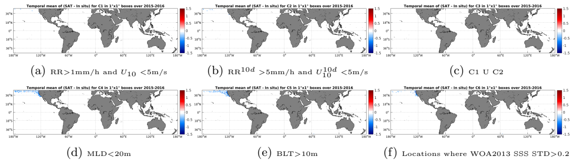
Figure 12: Temporal mean gridded over spatial boxes of size 1^\circ \times 1^\circ of \Delta SSS (SMAP-L3-RSS-V2-MONTHLY-0.25DEG-40KM - Sea mammals) for 6 different subdatasets corresponding to: RR > 1\text{mm/h} and U_{10} < 5\text{m/s} (a), RR^{10d} > 5\text{mm/h} and U_{10}^{10d} < 5\text{m/s} (b), C1 U C2 (c), MLD < 20\text{m} (d), BLT > 10\text{m} (e), Locations where WOA2013 SSS STD > 0.2 (f).
