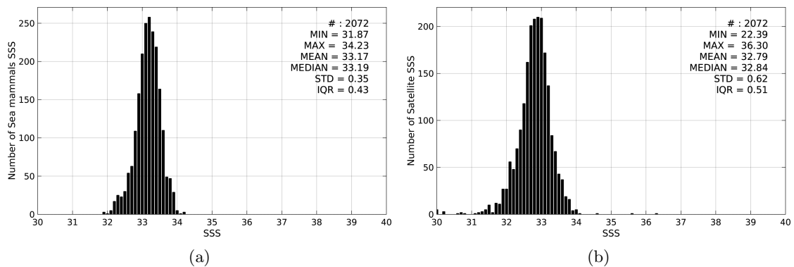
Figure 2: Histograms of SSS from Sea mammals (a) and SMAP-L3-RSS-V2-MONTHLY-0.25DEG-40KM (b) considering all match-up pairs per bins of 0.1 over the Mid-Low Latitudes 45N-45S Pi-MEP region and for the full satellite product period.
