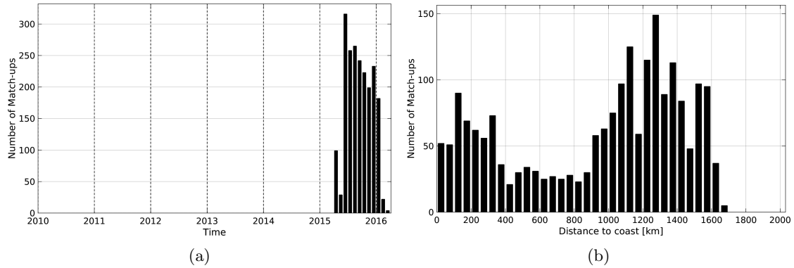
Figure 1: Number of match-ups between Sea mammals and SMAP-L3-RSS-V2-MONTHLY-0.25DEG-40KM SSS as a function of time (a) and as function of the distance to coast (b) over the Mid-Low Latitudes 45N-45S Pi-MEP region and for the full satellite product period.
