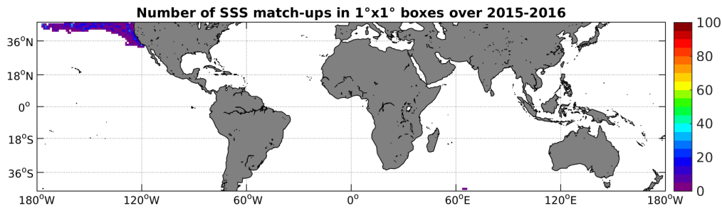
Figure 4: Number of SSS match-ups between Sea mammals SSS and the SMAP-L3-RSS-V2-MONTHLY-0.25DEG-40KM SSS product for the Mid-Low Latitudes 45N-45S Pi-MEP region over 1°x1° boxes and for the full satellite product period.
