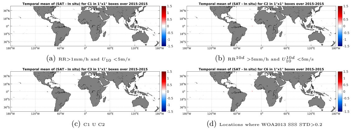
Figure 11: Temporal mean gridded over spatial boxes of size 1^\circ \times 1^\circ of \Delta SSS (SMAP-L3-RSS-V2-MONTHLY-0.25DEG-40KM - Surface drifters) for 4 different subdatasets corresponding to: RR > 1\text{mm/h} and U_{10} < 5\text{m/s} (a), RR^{10d} > 5\text{mm/h} and U_{10}^{10d} < 5\text{m/s} (b), C1 U C2 (c), Locations where WOA2013 SSS STD > 0.2 (d).
