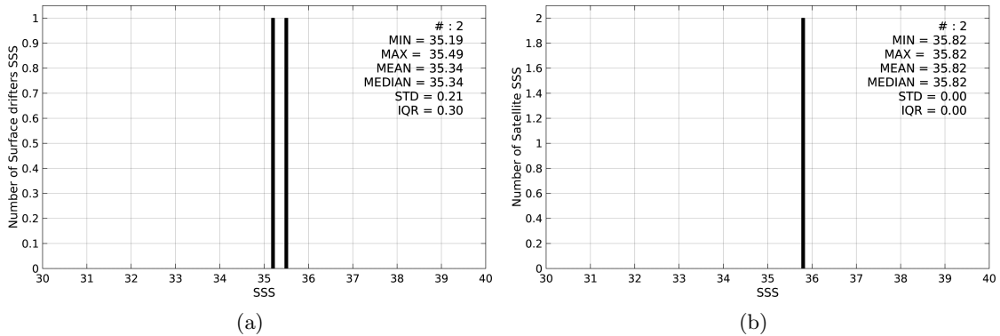
Figure 2: Histograms of SSS from Surface drifters (a) and SMAP-L3-RSS-V2-MONTHLY-0.25DEG-40KM (b) considering all match-up pairs per bins of 0.1 over the Mid-Low Latitudes 45N-45S Pi-MEP region and for the full satellite product period.
