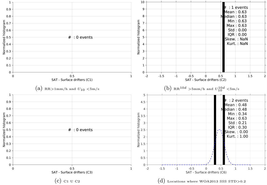
Figure 12: Normalized histogram of \Delta\text{SSS} (SMAP-L3-RSS-V2-MONTHLY-0.25DEG-40KM - Surface drifters) for 6 different subdatasets corresponding to: RR > 1\text{mm/h} and U_{10} < 5\text{m/s} (a), RR^{10d} > 5\text{mm/h} and U_{10}^{10d} < 5\text{m/s} (b), C1 U C2 (c), Locations where WOA2013 SSS STD > 0.2 (d).
