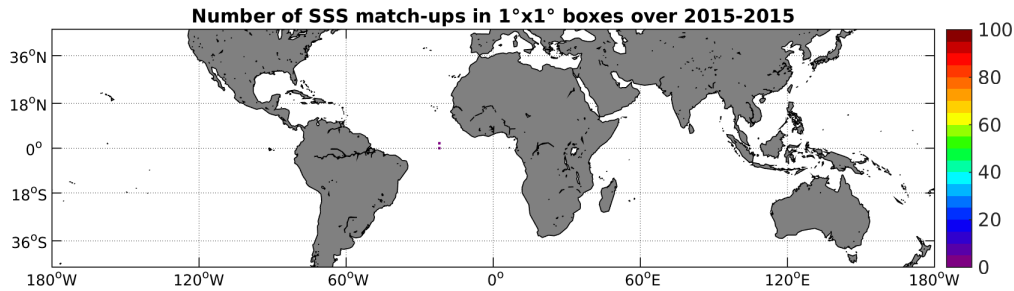
Figure 3: Number of SSS match-ups between Surface drifters SSS and the SMAP-L3-RSS-V2-MONTHLY-0.25DEG-40KM SSS product for the Mid-Low Latitudes 45N-45S Pi-MEP region over 1^\circ \times 1^\circ boxes and for the full satellite product period.
