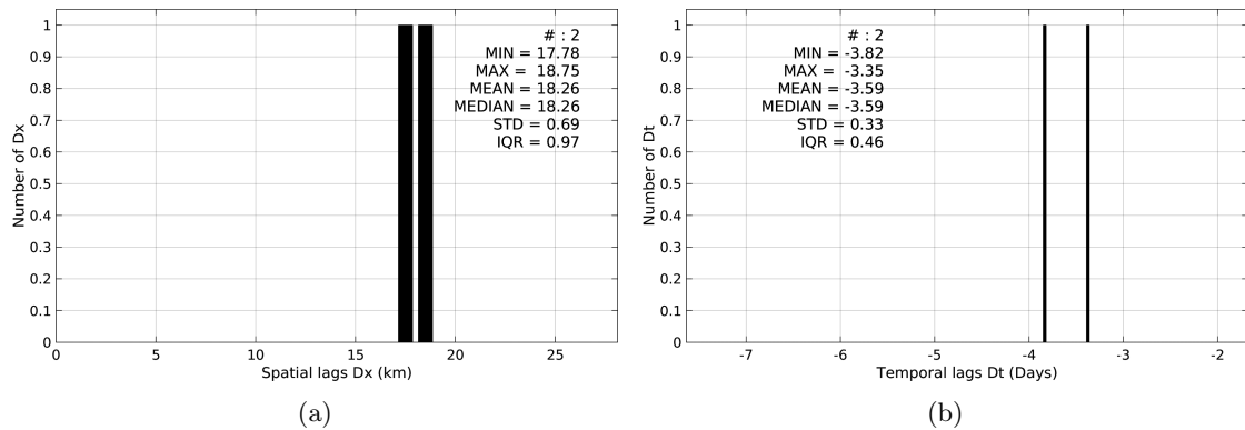
Figure 4: Histograms of the spatial (a) and temporal (b) lags between the time of the Surface drifters measurements and the date of the corresponding SMAP-L3-RSS-V2-MONTHLY-0.25DEG-40KM SSS product.
