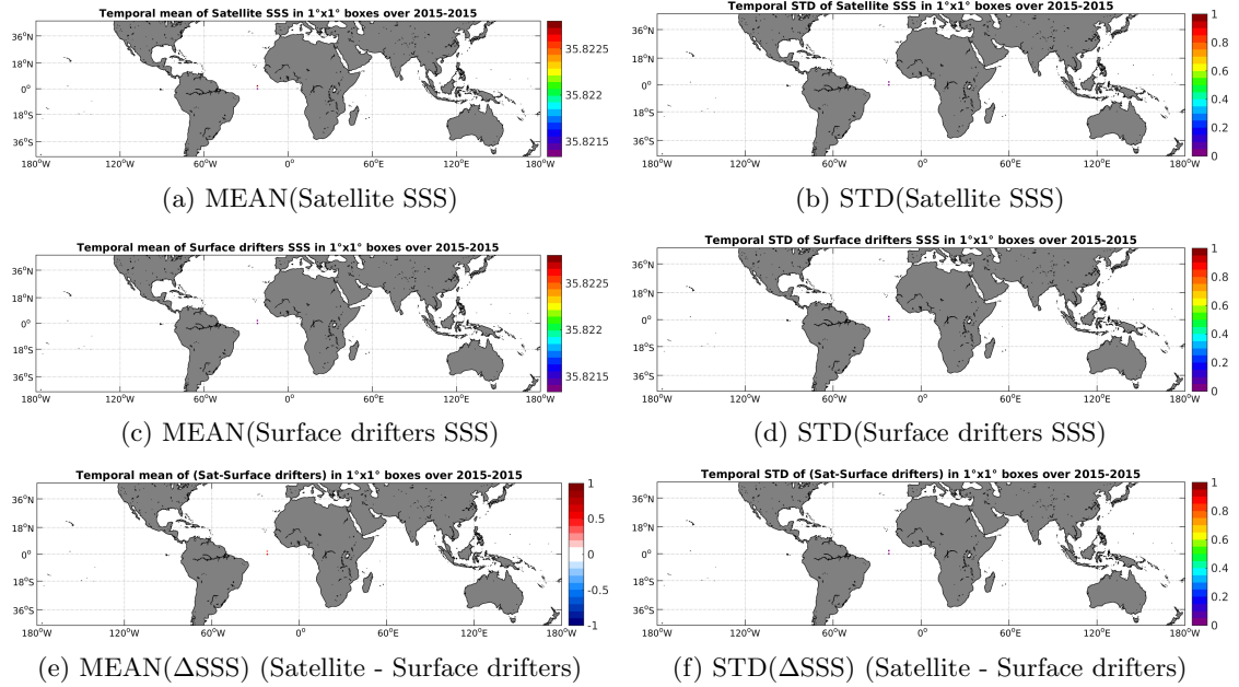
Figure 5: Temporal mean (left) and STD (right) of SSS from SMAP-L3-RSS-V2-MONTHLY-0.25DEG-40KM (top), Surface drifters (middle), and of \Delta SSS (Satellite - Surface drifters). Only match-up pairs are used to generate these maps.
