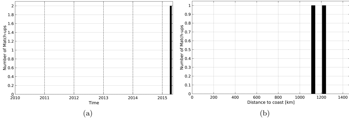
Figure 1: Number of match-ups between Surface drifters and SMAP-L3-RSS-V2-MONTHLY-0.25DEG-40KM SSS as a function of time (a) and as function of the distance to coast (b) over the Mid-Low Latitudes 45N-45S Pi-MEP region and for the full satellite product period.
