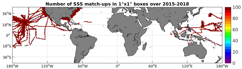
Figure 4: Number of SSS match-ups between TSG-SAMOS SSS and the SMAP-L3-RSS-V2-MONTHLY-70KM SSS product for the Mid-Low Latitudes 45N-45S Pi-MEP region over 1°x1° boxes and for the full satellite product period.
