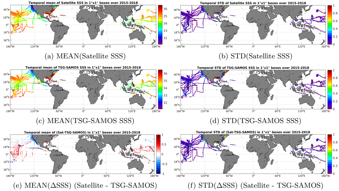
Figure 6: Temporal mean (left) and STD (right) of SSS from SMAP-L3-RSS-V2-MONTHLY-70KM (top), TSG-SAMOS (middle), and of \Delta SSS (Satellite - TSG-SAMOS). Only match-up pairs are used to generate these maps.
