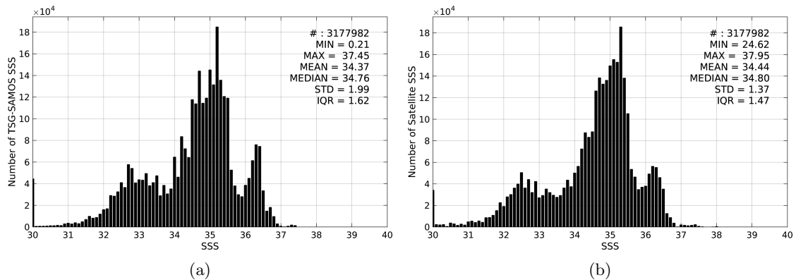
Figure 2: Histograms of SSS from TSG-SAMOS (a) and SMAP-L3-RSS-V2-MONTHLY-70KM (b) considering all match-up pairs per bins of 0.1 over the Mid-Low Latitudes 45N-45S Pi-MEP region and for the full satellite product period.
