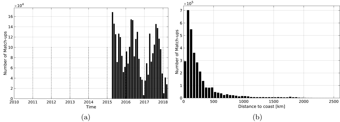
Figure 1: Number of match-ups between TSG-SAMOS and SMAP-L3-RSS-V2-MONTHLY-70KM SSS as a function of time (a) and as function of the distance to coast (b) over the Mid-Low Latitudes 45N-45S Pi-MEP region and for the full satellite product period.
