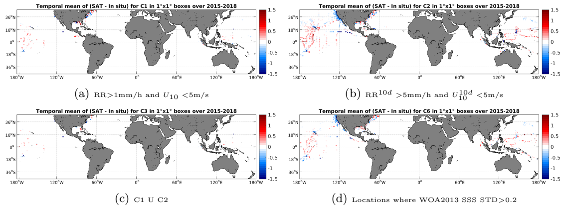
Figure 12: Temporal mean gridded over spatial boxes of size 1^\circ \times 1^\circ of \Delta SSS (SMAP-L3-RSS-V2-MONTHLY-70KM - TSG-SAMOS) for 4 different subdatasets corresponding to: RR > 1\text{mm/h} and U_{10} < 5\text{m/s} (a), RR^{10d} > 5\text{mm/h} and U_{10}^{10d} < 5\text{m/s} (b), C1 U C2 (c), Locations where WOA2013 SSS STD > 0.2 (d).
