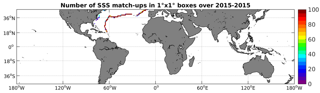
Figure 4: Number of SSS match-ups between TSG-GOSUD-Sailing-ship SSS and the SMAP-L3-RSS-V2-MONTHLY-70KM SSS product for the Mid-Low Latitudes 45N-45S Pi-MEP region over 1^\circ \times 1^\circ boxes and for the full satellite product period.
