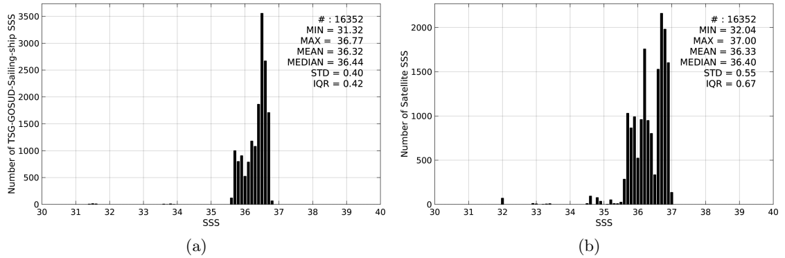
Figure 2: Histograms of SSS from TSG-GOSUD-Sailing-ship (a) and SMAP-L3-RSS-V2-MONTHLY-70KM (b) considering all match-up pairs per bins of 0.1 over the Mid-Low Latitudes 45N-45S Pi-MEP region and for the full satellite product period.
