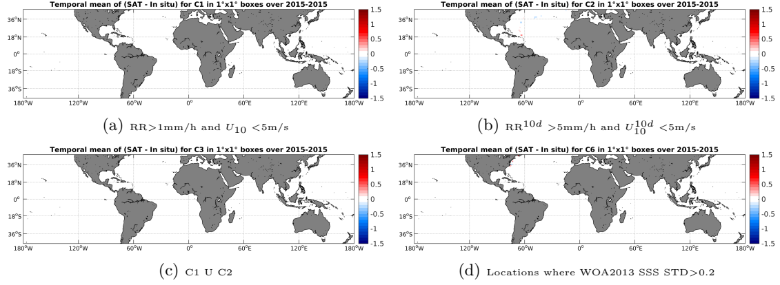
Figure 12: Temporal mean gridded over spatial boxes of size 1^\circ \times 1^\circ of \Delta SSS (SMAP-L3-RSS-V2-MONTHLY-70KM - TSG-GOSUD-Sailing-ship) for 4 different subdatasets corresponding to: RR > 1 mm/h and U_{10} < 5 m/s (a), RR^{10d} > 5 mm/h and U_{10}^{10d} < 5 m/s (b), C1 U C2 (c), Locations where WOA2013 SSS STD > 0.2 (d).
