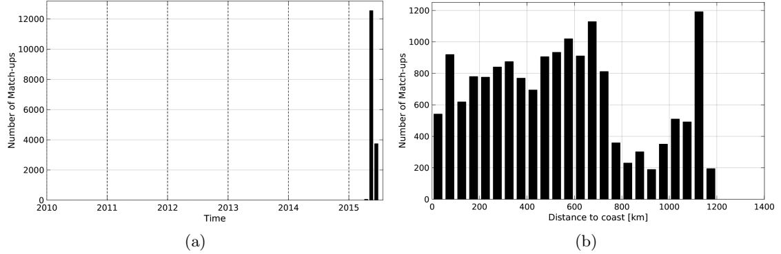
Figure 1: Number of match-ups between TSG-GOSUD-Sailing-ship and SMAP-L3-RSS-V2-MONTHLY-70KM SSS as a function of time (a) and as function of the distance to coast (b) over the Mid-Low Latitudes 45N-45S Pi-MEP region and for the full satellite product period.
