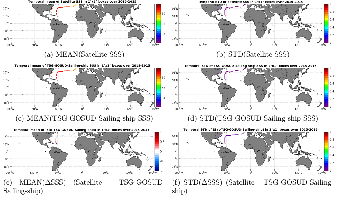
Figure 6: Temporal mean (left) and STD (right) of SSS from SMAP-L3-RSS-V2-MONTHLY-70KM (top), TSG-GOSUD-Sailing-ship (middle), and of \Delta SSS (Satellite - TSG-GOSUD-Sailing-ship). Only match-up pairs are used to generate these maps.
