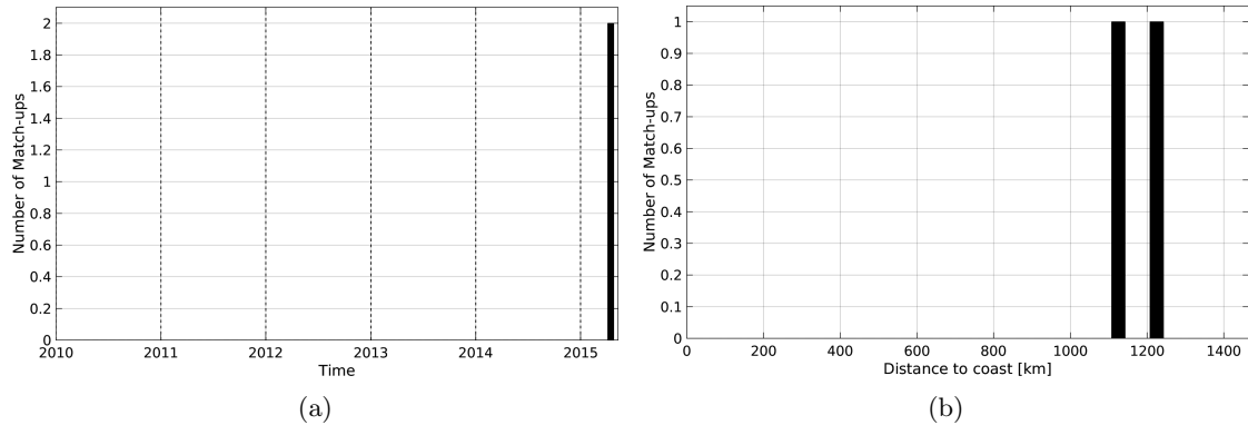
Figure 1: Number of match-ups between Surface drifters and SMAP-L3-RSS-V2-MONTHLY-70KM SSS as a function of time (a) and as function of the distance to coast (b) over the Mid-Low Latitudes 45N-45S Pi-MEP region and for the full satellite product period.
