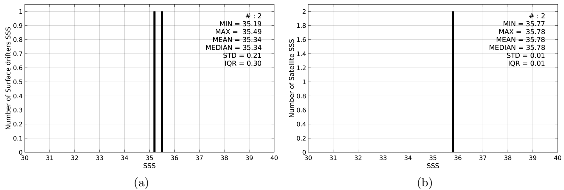
Figure 2: Histograms of SSS from Surface drifters (a) and SMAP-L3-RSS-V2-MONTHLY-70KM (b) considering all match-up pairs per bins of 0.1 over the Mid-Low Latitudes 45N-45S Pi-MEP region and for the full satellite product period.
