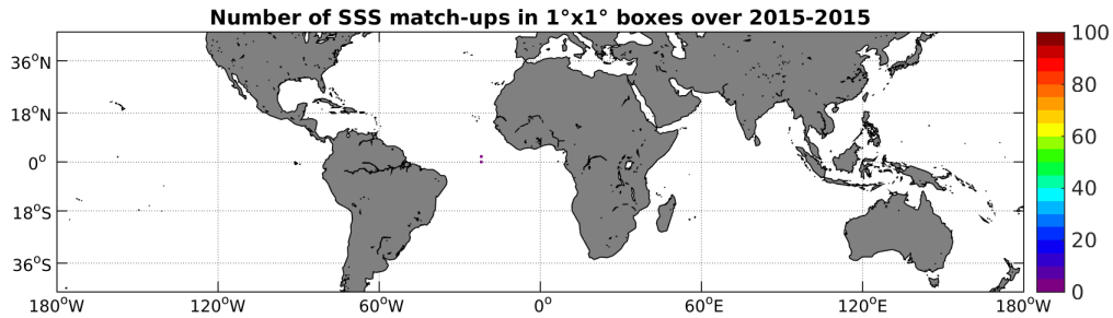
Figure 3: Number of SSS match-ups between Surface drifters SSS and the SMAP-L3-RSS-V2-MONTHLY-70KM SSS product for the Mid-Low Latitudes 45N-45S Pi-MEP region over 1^\circ \times 1^\circ boxes and for the full satellite product period.
