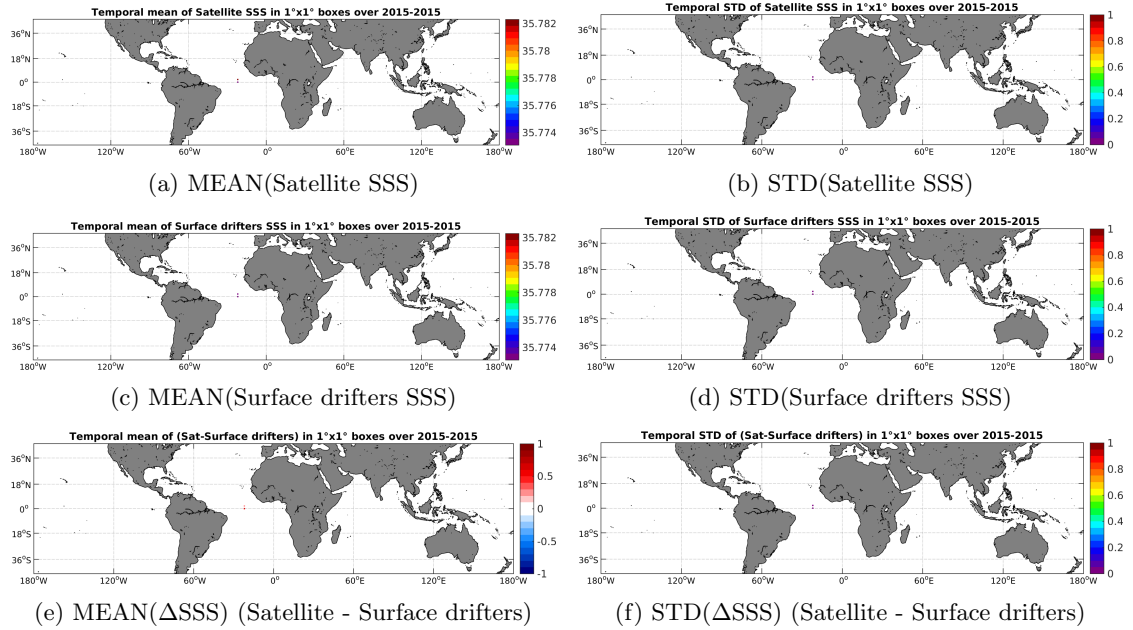
Figure 5: Temporal mean (left) and STD (right) of SSS from SMAP-L3-RSS-V2-MONTHLY-70KM (top), Surface drifters (middle), and of \Delta SSS (Satellite - Surface drifters). Only match-up pairs are used to generate these maps.
