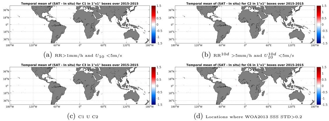
Figure 11: Temporal mean gridded over spatial boxes of size 1^\circ \times 1^\circ of \Delta SSS (SMAP-L3-RSS-V2-MONTHLY-70KM - Surface drifters) for 4 different subdatasets corresponding to: RR > 1\text{mm/h} and U_{10} < 5\text{m/s} (a), RR^{10d} > 5\text{mm/h} and U_{10}^{10d} < 5\text{m/s} (b), C1 U C2 (c), Locations where WOA2013 SSS STD > 0.2 (d).
