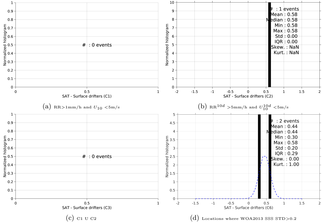
Figure 12: Normalized histogram of \Delta\text{SSS} (SMAP-L3-RSS-V2-MONTHLY-70KM - Surface drifters) for 6 different subdatasets corresponding to: RR > 1\text{mm/h} and U_{10} < 5\text{m/s} (a), RR^{10d} > 5\text{mm/h} and U_{10}^{10d} < 5\text{m/s} (b), C1 U C2 (c), Locations where WOA2013 SSS STD > 0.2 (d).
