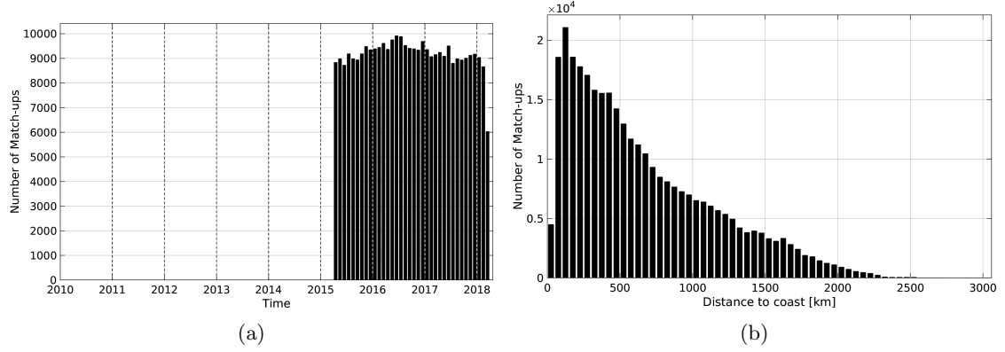
Figure 1: Number of match-ups between Argo and SMAP-L3-RSS-V2-MONTHLY-70KM SSS as a function of time (a) and as function of the distance to coast (b) over the Mid-Low Latitudes 45N-45S Pi-MEP region and for the full satellite product period.
