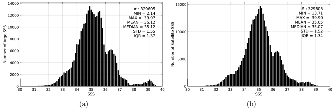
Figure 2: Histograms of SSS from Argo (a) and SMAP-L3-RSS-V2-MONTHLY-70KM (b) considering all match-up pairs per bins of 0.1 over the Mid-Low Latitudes 45N-45S Pi-MEP region and for the full satellite product period.
