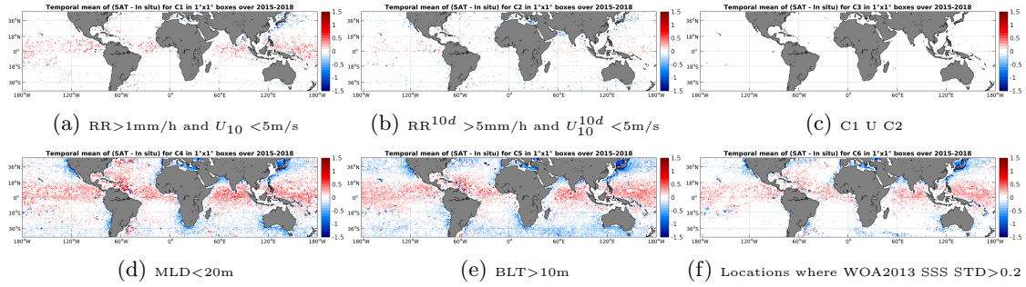
Figure 12: Temporal mean gridded over spatial boxes of size 1^\circ \times 1^\circ of \Delta SSS (SMAP-L3-RSS-V2-MONTHLY-70KM - Argo) for 6 different subdatasets corresponding to: RR>1mm/h and U_{10} < 5\text{m/s} (a), RR^{10d} > 5\text{mm/h} and U_{10}^{10d} < 5\text{m/s} (b), C1 U C2 (c), MLD<20m (d), BLT>10m (e), Locations where WOA2013 SSS STD>0.2 (f).
