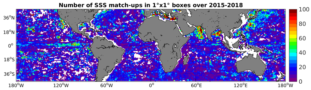
Figure 4: Number of SSS match-ups between Argo SSS and the SMAP-L3-RSS-V2-MONTHLY-70KM SSS product for the Mid-Low Latitudes 45N-45S Pi-MEP region over 1^\circ \times 1^\circ boxes and for the full satellite product period.
