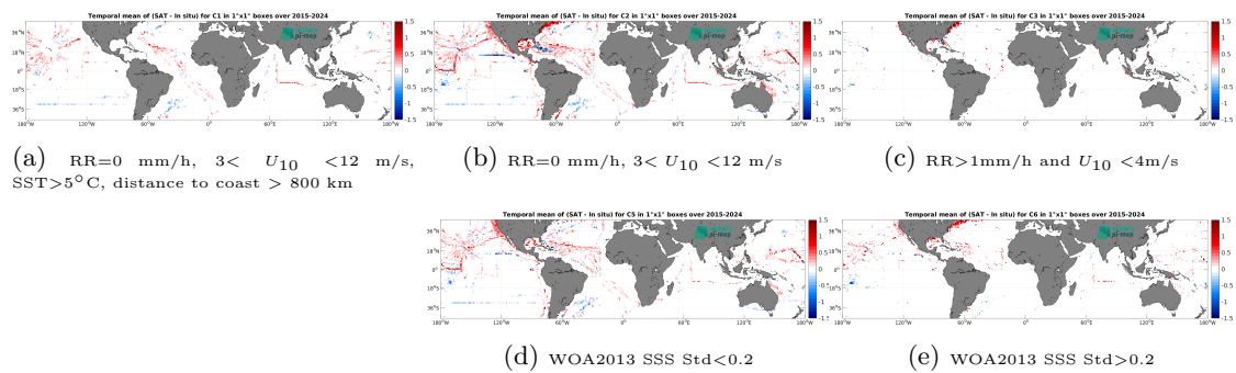
Figure 14: Temporal mean gridded over spatial boxes of size 1^\circ \times 1^\circ of \Delta SSS (SMAP SSS L3 v5.0 - 8-Day running (JPL) - TSG (SAMOS)) for 5 different subdatasets corresponding to: RR=0 mm/h, 3 < U_{10} < 12 m/s, SST > 5^\circ\text{C} , distance to coast > 800 km (a), RR=0 mm/h, 3 < U_{10} < 12 m/s (b), RR > 1 mm/h and U_{10} < 4 m/s (c), WOA2013 SSS Std < 0.2 (d), WOA2013 SSS Std > 0.2 (e).
