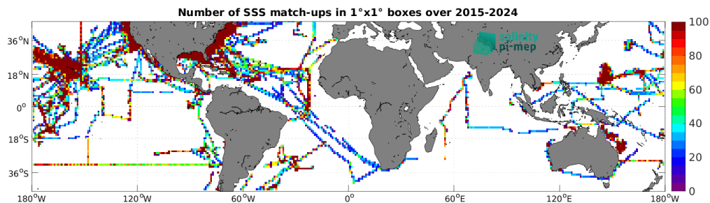
Figure 5: Number of SSS match-ups between TSG (SAMOS) SSS and the SMAP SSS L3 v5.0 - 8-Day running (JPL) SSS product for the Mid-Low Latitudes 45N-45S Pi-MEP region over 1^\circ \times 1^\circ boxes and for the full satellite product period.
