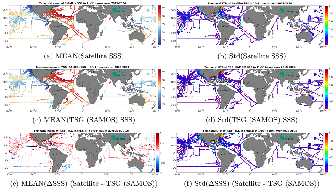
Figure 7: Temporal mean (left) and Std (right) of SSS from SMAP SSS L3 v5.0 - 8-Day running (JPL) (top), TSG (SAMOS) (middle), and of \Delta SSS (Satellite - TSG (SAMOS)). Only match-up pairs are used to generate these maps.
