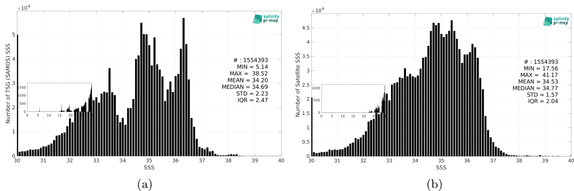
Figure 3: Histograms of SSS from TSG (SAMOS) (a) and SMAP SSS L3 v5.0 - 8-Day running (JPL) (b) considering all match-up pairs per bins of 0.1 over the Mid-Low Latitudes 45N-45S Pi-MEP region and for the full satellite product period.
