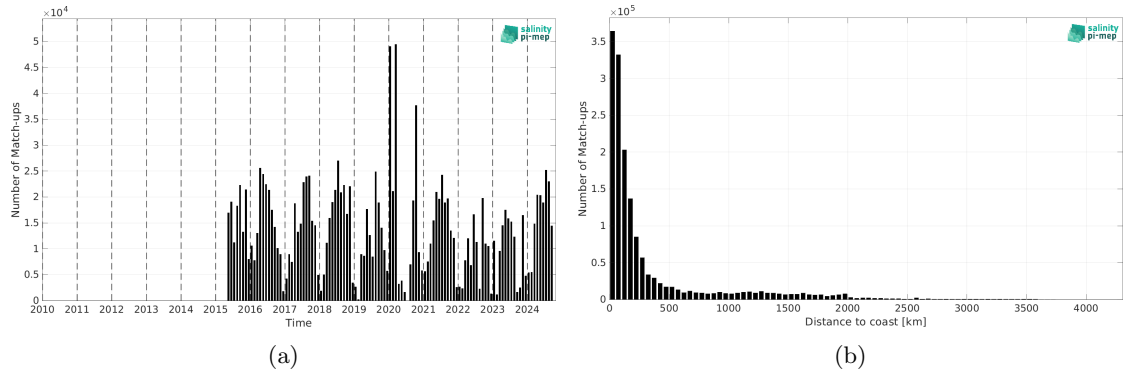
Figure 2: Number of match-ups between TSG (SAMOS) and SMAP SSS L3 v5.0 - 8-Day running (JPL) SSS as a function of time (a) and as function of the distance to coast (b) over the Mid-Low Latitudes 45N-45S Pi-MEP region and for the full satellite product period.
