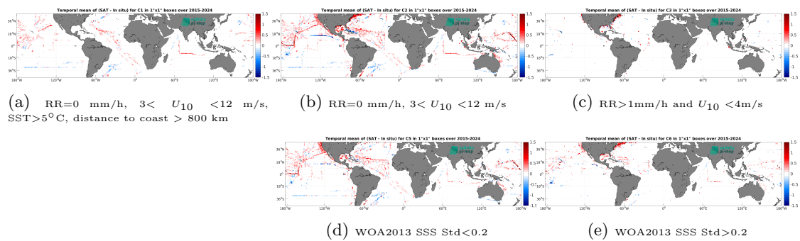
Figure 14: Temporal mean gridded over spatial boxes of size 1^\circ \times 1^\circ of \Delta\text{SSS} (SMAP SSS L3 v5.0 - 8-Day running (JPL) - TSG (SAMOS)) for 5 different subdatasets corresponding to:RR=0 mm/h, 3 < U_{10} < 12 m/s, SST >5^\circ\text{C} , distance to coast > 800 km (a), RR=0 mm/h, 3 < U_{10} < 12 m/s (b), RR >1 mm/h and U_{10} < 4 m/s (c), WOA2013 SSS Std <0.2 (d), WOA2013 SSS Std >0.2 (e).
