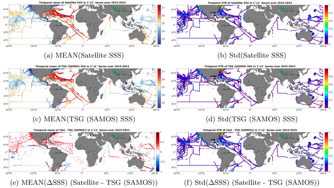
Figure 6: Temporal mean (left) and Std (right) of SSS from SMAP SSS L3 v5.0 - 8-Day running (JPL) (top), TSG (SAMOS) (middle), and of \Delta SSS (Satellite - TSG (SAMOS)). Only match-up pairs are used to generate these maps.
