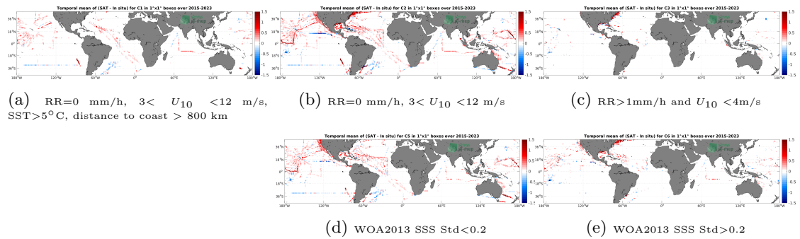
Figure 12: Temporal mean gridded over spatial boxes of size 1^\circ \times 1^\circ of \Delta SSS (SMAP SSS L3 v5.0 - 8-Day running (JPL) - TSG (SAMOS)) for 5 different subdatasets corresponding to:RR=0 mm/h, 3 < U_{10} < 12 m/s, SST >5^\circ C, distance to coast > 800 km (a), RR=0 mm/h, 3 < U_{10} < 12 m/s (b), RR >1 mm/h and U_{10} < 4 m/s (c), WOA2013 SSS Std <0.2 (d), WOA2013 SSS Std >0.2 (e).
