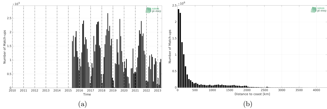
Figure 1: Number of match-ups between TSG (SAMOS) and SMAP SSS L3 v5.0 - 8-Day running (JPL) SSS as a function of time (a) and as function of the distance to coast (b) over the Mid-Low Latitudes 45N-45S Pi-MEP region and for the full satellite product period.
