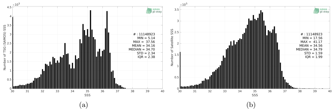
Figure 2: Histograms of SSS from TSG (SAMOS) (a) and SMAP SSS L3 v5.0 - 8-Day running (JPL) (b) considering all match-up pairs per bins of 0.1 over the Mid-Low Latitudes 45N-45S Pi-MEP region and for the full satellite product period.
