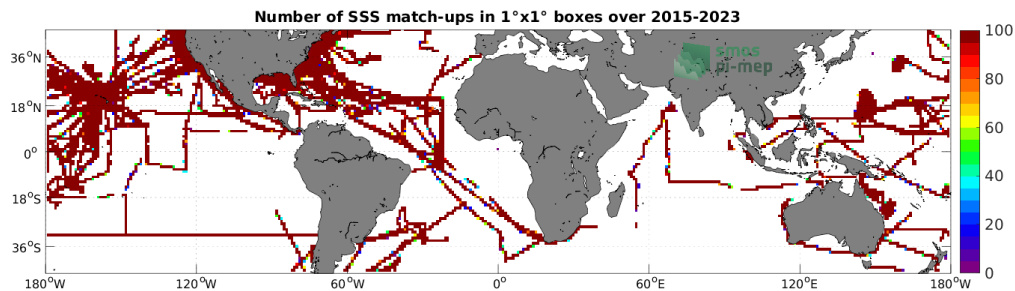
Figure 4: Number of SSS match-ups between TSG (SAMOS) SSS and the SMAP SSS L3 v5.0 - 8-Day running (JPL) SSS product for the Mid-Low Latitudes 45N-45S Pi-MEP region over 1^\circ \times 1^\circ boxes and for the full satellite product period.
