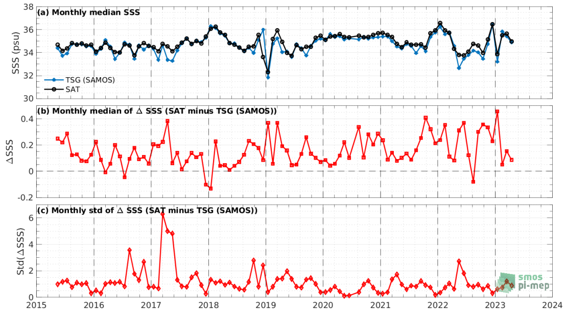
Figure 7: Time series of the monthly median SSS (top), median of \Delta\text{SSS} (Satellite - TSG (SAMOS)) and Std of \Delta\text{SSS} (Satellite - TSG (SAMOS)) over the Mid-Low Latitudes 45N-45S Pi-MEP region considering all match-ups collected by the Pi-MEP.
