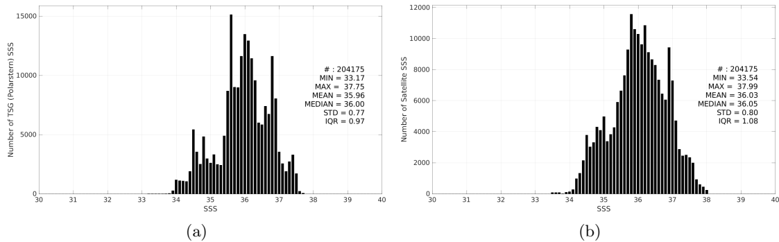
Figure 3: Histograms of SSS from TSG (Polarstern) (a) and SMAP SSS L3 v5.0 - 8-Day running (JPL) (b) considering all match-up pairs per bins of 0.1 over the Mid-Low Latitudes 45N-45S Pi-MEP region and for the full satellite product period.
