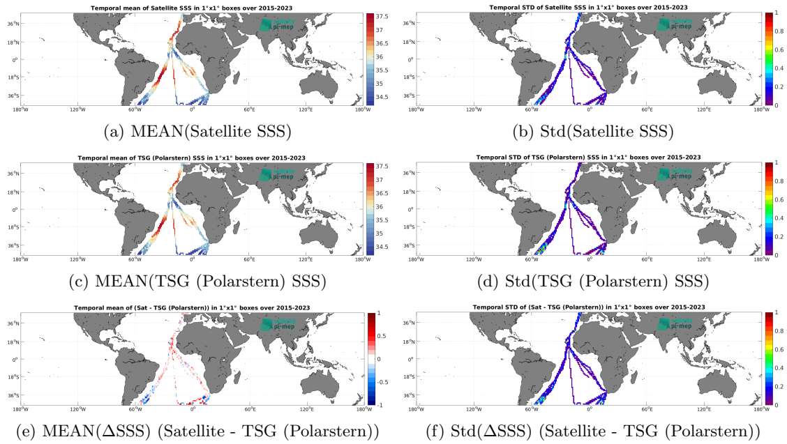
Figure 7: Temporal mean (left) and Std (right) of SSS from SMAP SSS L3 v5.0 - 8-Day running (JPL) (top), TSG (Polarstern) (middle), and of \Delta SSS (Satellite - TSG (Polarstern)). Only match-up pairs are used to generate these maps.
