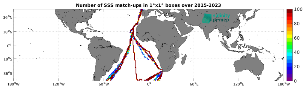
Figure 5: Number of SSS match-ups between TSG (Polarstern) SSS and the SMAP SSS L3 v5.0 - 8-Day running (JPL) SSS product for the Mid-Low Latitudes 45N-45S Pi-MEP region over 1^\circ \times 1^\circ boxes and for the full satellite product period.
