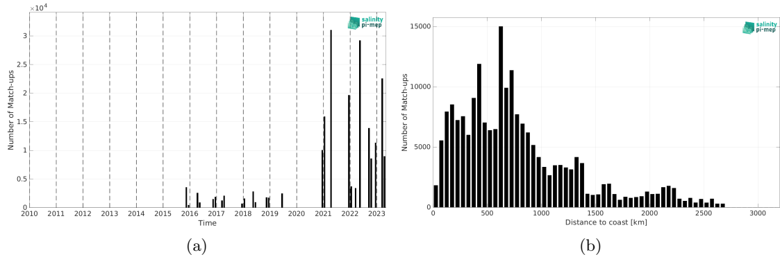
Figure 2: Number of match-ups between TSG (Polarstern) and SMAP SSS L3 v5.0 - 8-Day running (JPL) SSS as a function of time (a) and as function of the distance to coast (b) over the Mid-Low Latitudes 45N-45S Pi-MEP region and for the full satellite product period.
