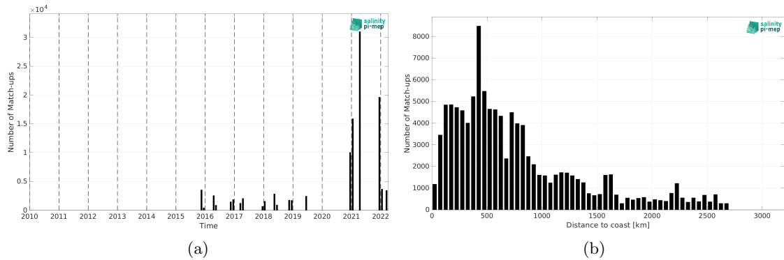
Figure 1: Number of match-ups between TSG (Polarstern) and SMAP SSS L3 v5.0 - 8-Day running (JPL) SSS as a function of time (a) and as function of the distance to coast (b) over the Mid-Low Latitudes 45N-45S Pi-MEP region and for the full satellite product period.
