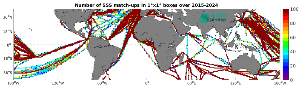
Figure 5: Number of SSS match-ups between TSG (LEGOS-DM) SSS and the SMAP SSS L3 v5.0 - 8-Day running (JPL) SSS product for the Mid-Low Latitudes 45N-45S Pi-MEP region over 1^\circ \times 1^\circ boxes and for the full satellite product period.
