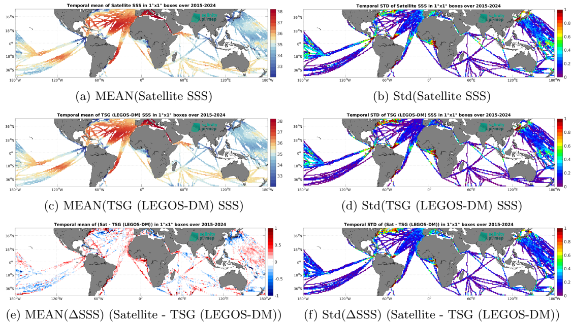
Figure 7: Temporal mean (left) and Std (right) of SSS from SMAP SSS L3 v5.0 - 8-Day running (JPL) (top), TSG (LEGOS-DM) (middle), and of \Delta SSS (Satellite - TSG (LEGOS-DM)). Only match-up pairs are used to generate these maps.
