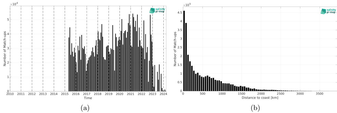
Figure 2: Number of match-ups between TSG (LEGOS-DM) and SMAP SSS L3 v5.0 - 8-Day running (JPL) SSS as a function of time (a) and as function of the distance to coast (b) over the Mid-Low Latitudes 45N-45S Pi-MEP region and for the full satellite product period.
