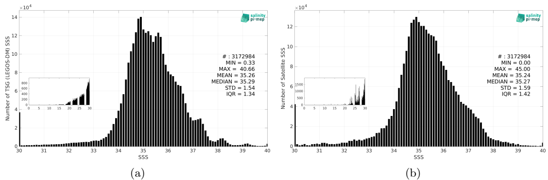
Figure 3: Histograms of SSS from TSG (LEGOS-DM) (a) and SMAP SSS L3 v5.0 - 8-Day running (JPL) (b) considering all match-up pairs per bins of 0.1 over the Mid-Low Latitudes 45N-45S Pi-MEP region and for the full satellite product period.
