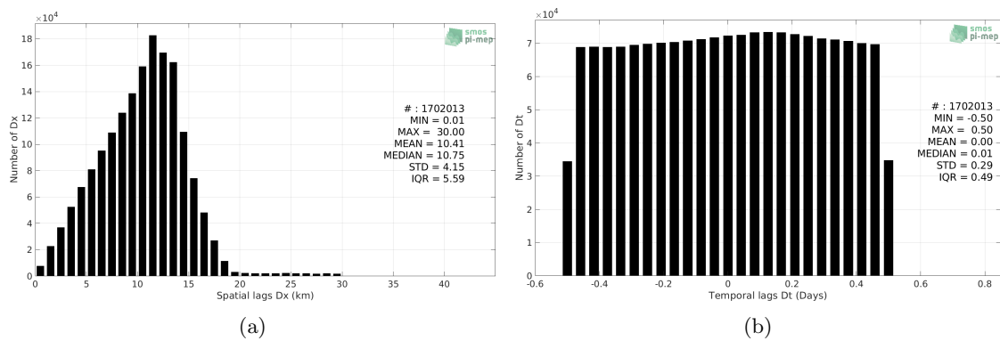
Figure 5: Histograms of the spatial (a) and temporal (b) lags between the location/time of the TSG (LEGOS-DM) measurement and the date of the corresponding SMAP SSS L3 v5.0 - 8-Day running (JPL) SSS pixel.
