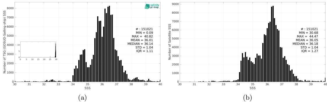
Figure 3: Histograms of SSS from TSG (GOSUD-Sailing-ship) (a) and SMAP SSS L3 v5.0 - 8-Day running (JPL) (b) considering all match-up pairs per bins of 0.1 over the Mid-Low Latitudes 45N-45S Pi-MEP region and for the full satellite product period.
