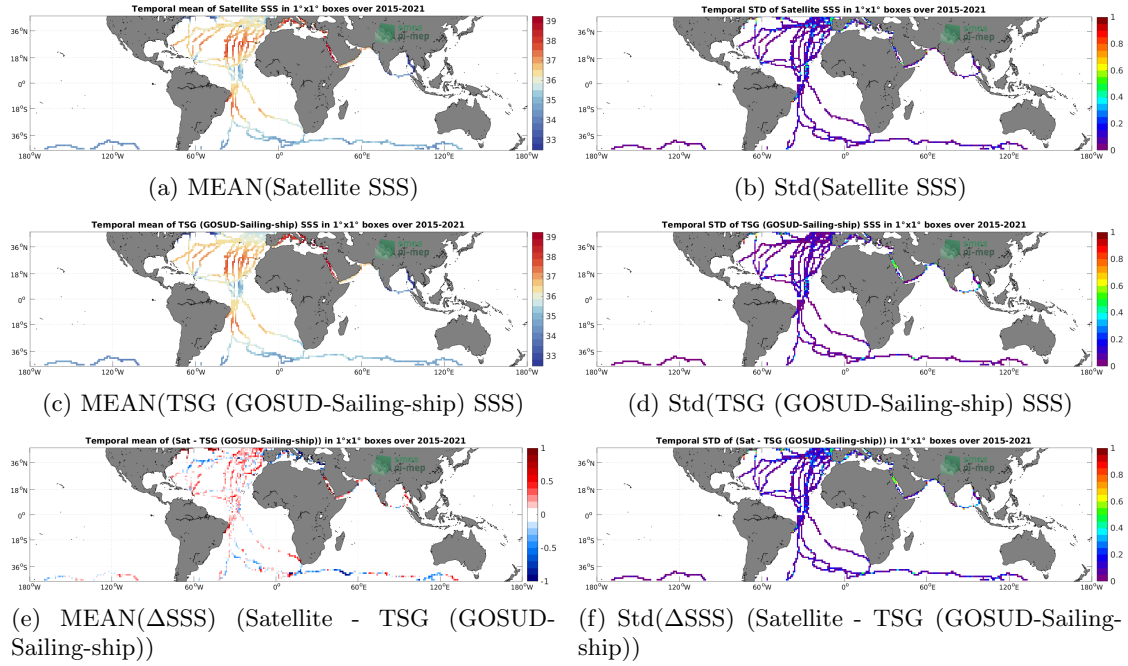
Figure 6: Temporal mean (left) and Std (right) of SSS from SMAP SSS L3 v5.0 - 8-Day running (JPL) (top), TSG (GOSUD-Sailing-ship) (middle), and of \Delta SSS (Satellite - TSG (GOSUD-Sailing-ship)). Only match-up pairs are used to generate these maps.
