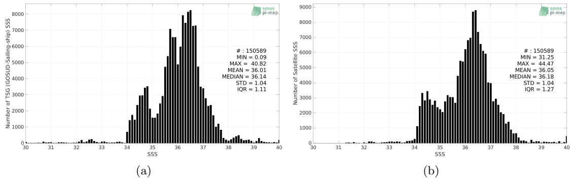
Figure 2: Histograms of SSS from TSG (GOSUD-Sailing-ship) (a) and SMAP SSS L3 v5.0 - 8-Day running (JPL) (b) considering all match-up pairs per bins of 0.1 over the Mid-Low Latitudes 45N-45S Pi-MEP region and for the full satellite product period.
