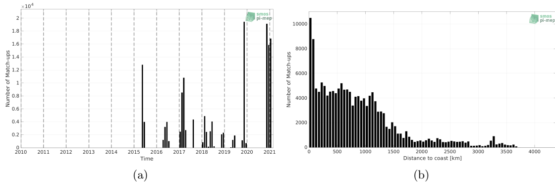
Figure 1: Number of match-ups between TSG (GOSUD-Sailing-ship) and SMAP SSS L3 v5.0 - 8-Day running (JPL) SSS as a function of time (a) and as function of the distance to coast (b) over the Mid-Low Latitudes 45N-45S Pi-MEP region and for the full satellite product period.
