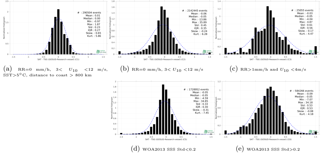
Figure 13: Normalized histogram of \Delta\text{SSS} (SMAP SSS L3 v5.0 - 8-Day running (JPL) - TSG (GOSUD-Research-vessel)) for 5 different subdatasets corresponding to: RR=0 mm/h, 3 < U_{10} < 12 m/s, SST > 5^\circ\text{C} , distance to coast > 800 km (a), RR=0 mm/h, 3 < U_{10} < 12 m/s (b), RR > 1\text{mm/h} and U_{10} < 4\text{m/s} (c), WOA2013 SSS Std < 0.2 (d), WOA2013 SSS Std > 0.2 (e).
