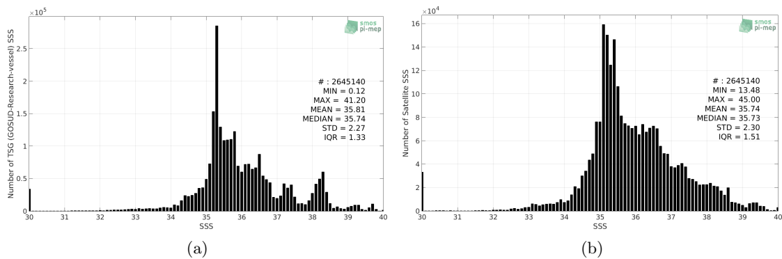
Figure 2: Histograms of SSS from TSG (GOSUD-Research-vessel) (a) and SMAP SSS L3 v5.0 - 8-Day running (JPL) (b) considering all match-up pairs per bins of 0.1 over the Mid-Low Latitudes 45N-45S Pi-MEP region and for the full satellite product period.
