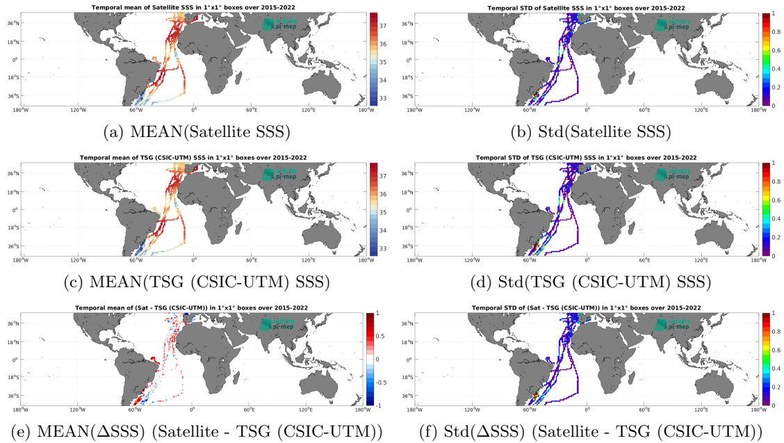
Figure 7: Temporal mean (left) and Std (right) of SSS from SMAP SSS L3 v5.0 - 8-Day running (JPL) (top), TSG (CSIC-UTM) (middle), and of \Delta SSS (Satellite - TSG (CSIC-UTM)). Only match-up pairs are used to generate these maps.
