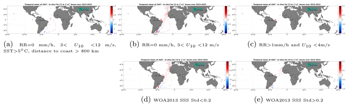
Figure 14: Temporal mean gridded over spatial boxes of size 1^\circ \times 1^\circ of \Delta SSS (SMAP SSS L3 v5.0 - 8-Day running (JPL) - TSG (CSIC-UTM)) for 5 different subdatasets corresponding to: RR=0 mm/h, 3 < U_{10} < 12 m/s, SST > 5°C, distance to coast > 800 km (a), RR=0 mm/h, 3 < U_{10} < 12 m/s (b), RR > 1mm/h and U_{10} < 4 m/s (c), WOA2013 SSS Std < 0.2 (d), WOA2013 SSS Std > 0.2 (e).
