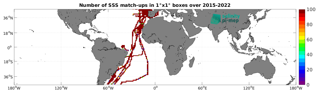
Figure 5: Number of SSS match-ups between TSG (CSIC-UTM) SSS and the SMAP SSS L3 v5.0 - 8-Day running (JPL) SSS product for the Mid-Low Latitudes 45N-45S Pi-MEP region over 1^\circ \times 1^\circ boxes and for the full satellite product period.
