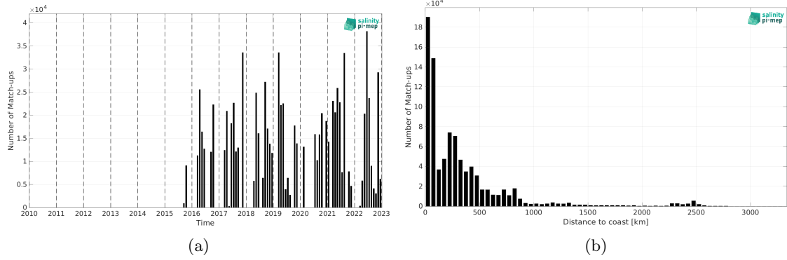
Figure 2: Number of match-ups between TSG (CSIC-UTM) and SMAP SSS L3 v5.0 - 8-Day running (JPL) SSS as a function of time (a) and as function of the distance to coast (b) over the Mid-Low Latitudes 45N-45S Pi-MEP region and for the full satellite product period.
