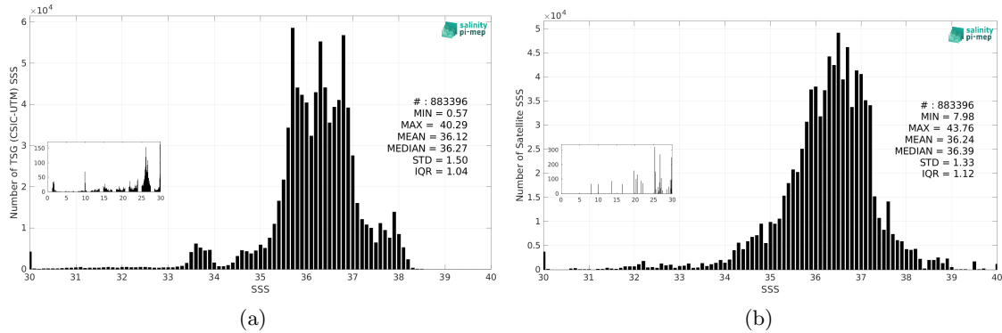
Figure 3: Histograms of SSS from TSG (CSIC-UTM) (a) and SMAP SSS L3 v5.0 - 8-Day running (JPL) (b) considering all match-up pairs per bins of 0.1 over the Mid-Low Latitudes 45N-45S Pi-MEP region and for the full satellite product period.
