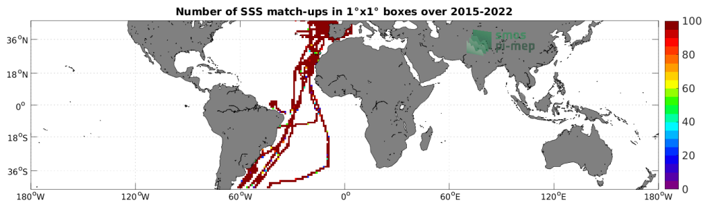
Figure 4: Number of SSS match-ups between TSG (CSIC-UTM) SSS and the SMAP SSS L3 v5.0 - 8-Day running (JPL) SSS product for the Mid-Low Latitudes 45N-45S Pi-MEP region over 1^\circ \times 1^\circ boxes and for the full satellite product period.
