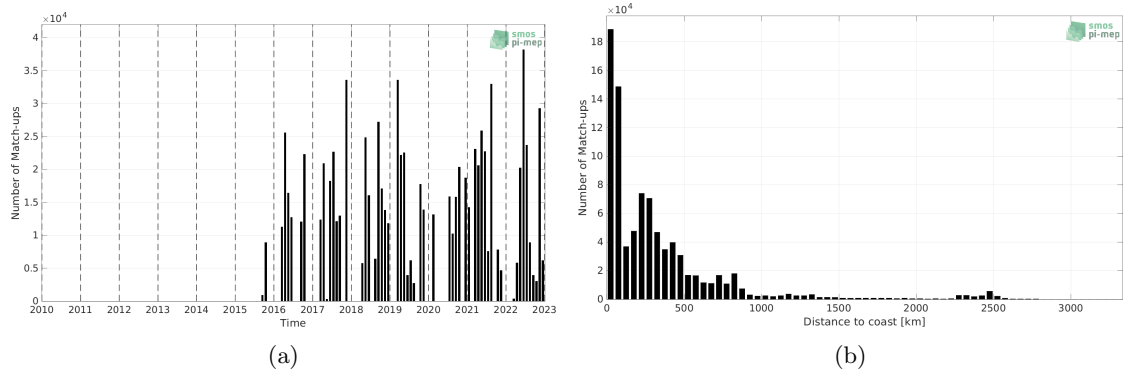
Figure 1: Number of match-ups between TSG (CSIC-UTM) and SMAP SSS L3 v5.0 - 8-Day running (JPL) SSS as a function of time (a) and as function of the distance to coast (b) over the Mid-Low Latitudes 45N-45S Pi-MEP region and for the full satellite product period.
