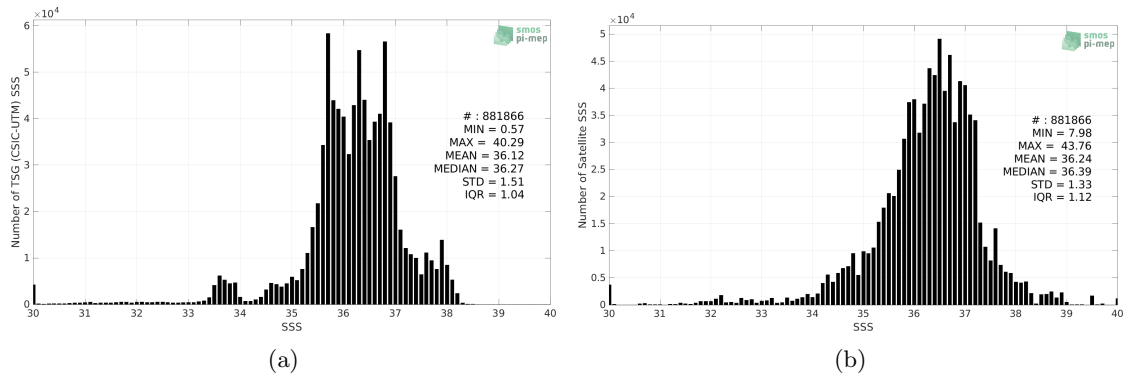
Figure 2: Histograms of SSS from TSG (CSIC-UTM) (a) and SMAP SSS L3 v5.0 - 8-Day running (JPL) (b) considering all match-up pairs per bins of 0.1 over the Mid-Low Latitudes 45N-45S Pi-MEP region and for the full satellite product period.
