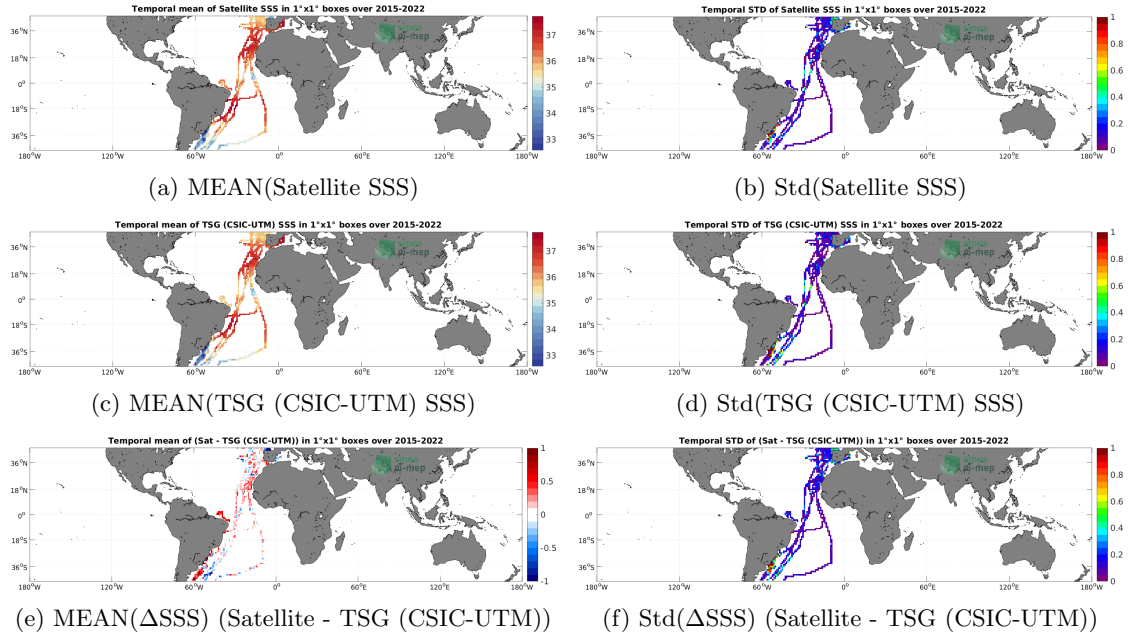
Figure 6: Temporal mean (left) and Std (right) of SSS from SMAP SSS L3 v5.0 - 8-Day running (JPL) (top), TSG (CSIC-UTM) (middle), and of \Delta SSS (Satellite - TSG (CSIC-UTM)). Only match-up pairs are used to generate these maps.
