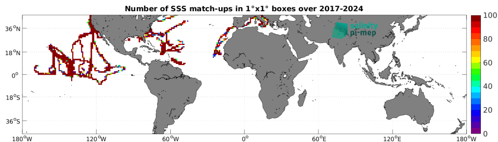
Figure 5: Number of SSS match-ups between Saildrone SSS and the SMAP SSS L3 v5.0 - 8-Day running (JPL) SSS product for the Mid-Low Latitudes 45N-45S Pi-MEP region over 1^\circ \times 1^\circ boxes and for the full satellite product period.
