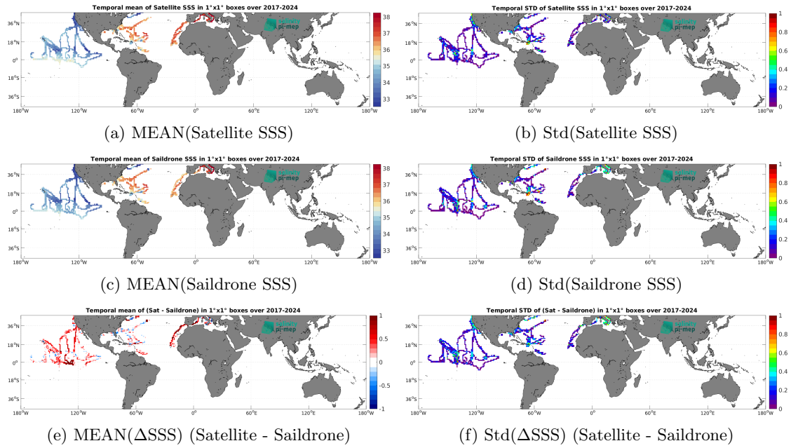
Figure 7: Temporal mean (left) and Std (right) of SSS from SMAP SSS L3 v5.0 - 8-Day running (JPL) (top), Saildrone (middle), and of \Delta SSS (Satellite - Saildrone). Only match-up pairs are used to generate these maps.
