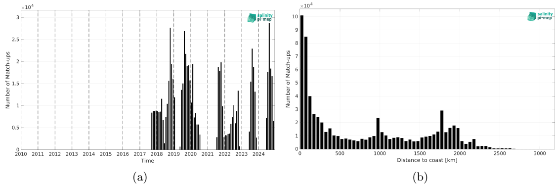
Figure 2: Number of match-ups between Sairdrone and SMAP SSS L3 v5.0 - 8-Day running (JPL) SSS as a function of time (a) and as function of the distance to coast (b) over the Mid-Low Latitudes 45N-45S Pi-MEP region and for the full satellite product period.
