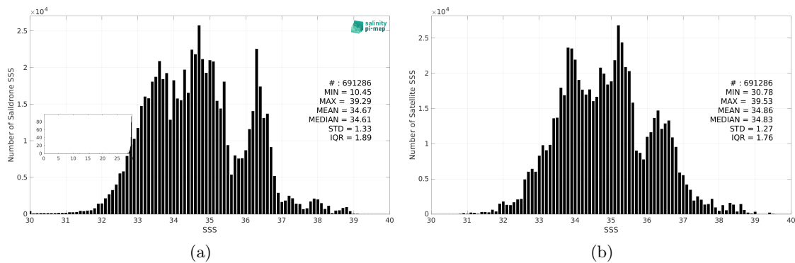
Figure 3: Histograms of SSS from Sairdrone (a) and SMAP SSS L3 v5.0 - 8-Day running (JPL) (b) considering all match-up pairs per bins of 0.1 over the Mid-Low Latitudes 45N-45S Pi-MEP region and for the full satellite product period.
