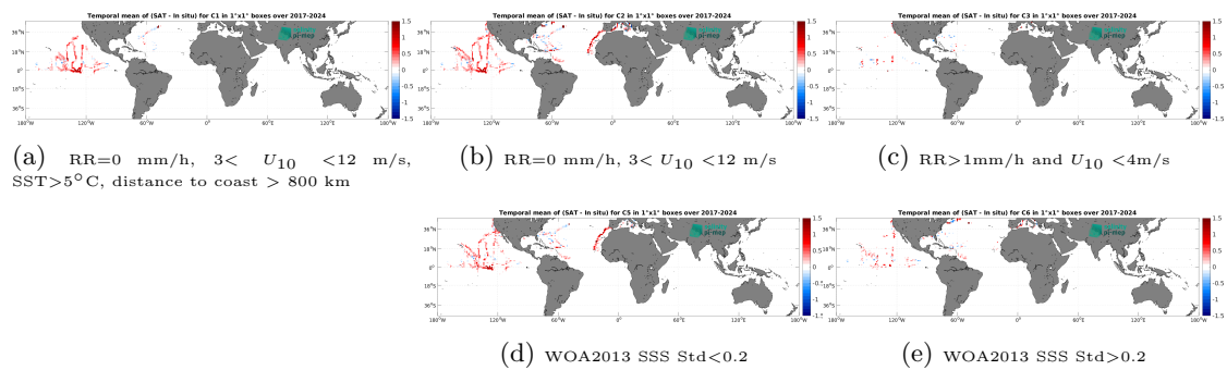
Figure 14: Temporal mean gridded over spatial boxes of size 1^\circ \times 1^\circ of \Delta\text{SSS} (SMAP SSS L3 v5.0 - 8-Day running (JPL) - Saildrone) for 5 different subdatasets corresponding to: RR=0 mm/h, 3 < U_{10} < 12 m/s, SST > 5°C, distance to coast > 800 km (a), RR=0 mm/h, 3 < U_{10} < 12 m/s (b), RR > 1mm/h and U_{10} < 4 m/s (c), WOA2013 SSS Std < 0.2 (d), WOA2013 SSS Std > 0.2 (e).
