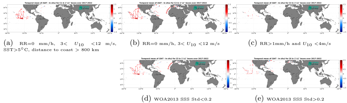
Figure 12: Temporal mean gridded over spatial boxes of size 1^\circ \times 1^\circ of \Delta\text{SSS} (SMAP SSS L3 v5.0 - 8-Day running (JPL) - Saildrone) for 5 different subdatasets corresponding to:RR=0 mm/h, 3 < U_{10} < 12 m/s, SST >5^\circ\text{C} , distance to coast > 800 km (a), RR=0 mm/h, 3 < U_{10} < 12 m/s (b), RR >1 mm/h and U_{10} < 4 m/s (c), WOA2013 SSS Std <0.2 (d), WOA2013 SSS Std >0.2 (e).
