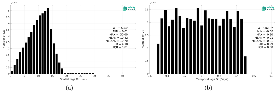
Figure 5: Histograms of the spatial (a) and temporal (b) lags between the location/time of the Sailability measurement and the date of the corresponding SMAP SSS L3 v5.0 - 8-Day running (JPL) SSS pixel.
