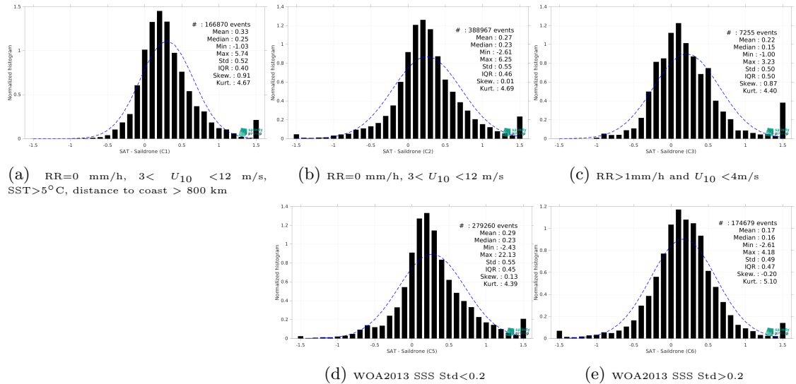
Figure 13: Normalized histogram of \Delta\text{SSS} (SMAP SSS L3 v5.0 - 8-Day running (JPL) - Saildrone) for 5 different subdatasets corresponding to: RR=0 mm/h, 3 < U_{10} < 12 m/s, SST >5^\circ\text{C} , distance to coast > 800 km (a), RR=0 mm/h, 3 < U_{10} < 12 m/s (b), RR >1 mm/h and U_{10} < 4 m/s (c), WOA2013 SSS Std <0.2 (d), WOA2013 SSS Std >0.2 (e).
