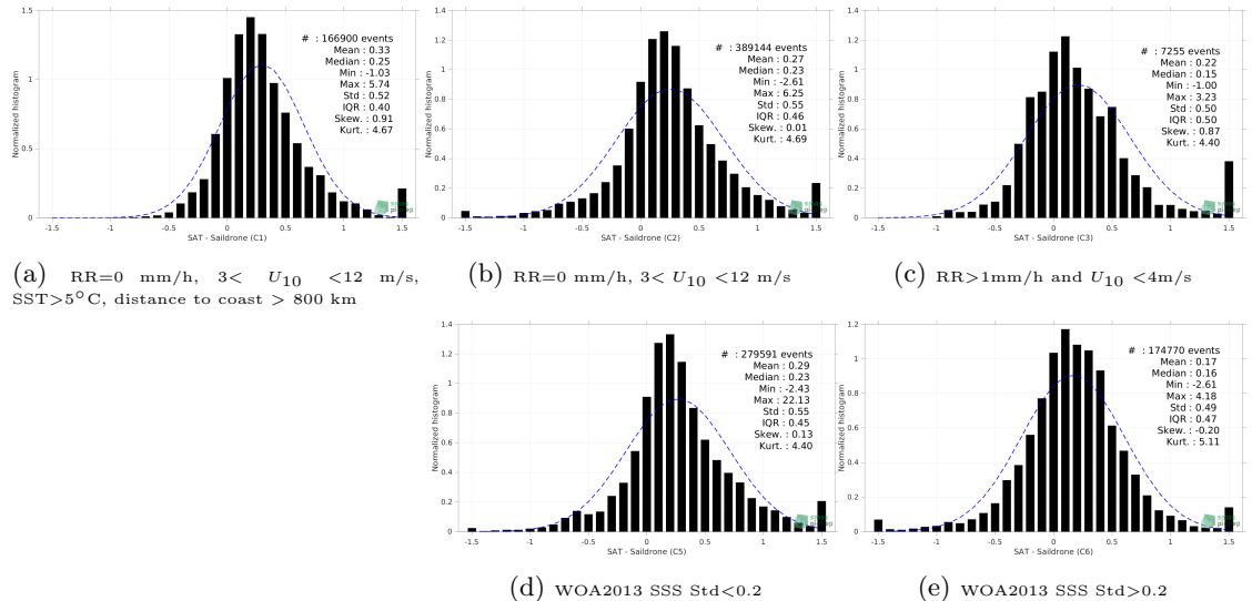
Figure 13: Normalized histogram of \Delta SSS (SMAP SSS L3 v5.0 - 8-Day running (JPL) - Saildrone) for 5 different subdatasets corresponding to: RR=0 mm/h, 3 < U_{10} < 12 m/s, SST>5°C, distance to coast > 800 km (a), RR=0 mm/h, 3 < U_{10} < 12 m/s (b), RR>1mm/h and U_{10} < 4 m/s (c), WOA2013 SSS Std<0.2 (d), WOA2013 SSS Std>0.2 (e).
