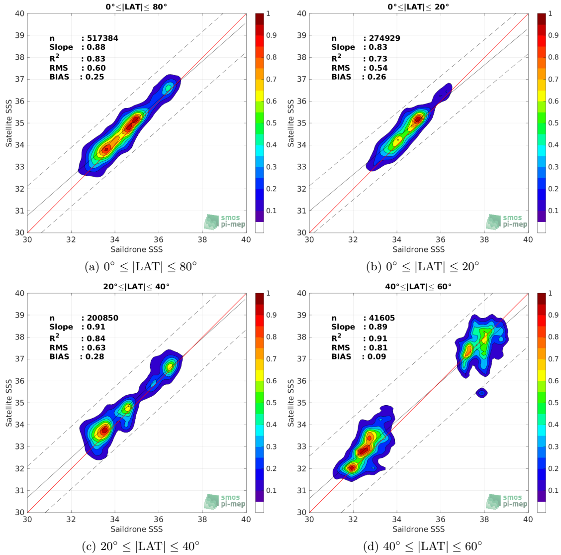
Figure 9: Contour maps of the concentration of SMAP SSS L3 v5.0 - 8-Day running (JPL) SSS (y-axis) versus Saildrone SSS (x-axis) at match-up pairs for different latitude bands. For each plot, the red line shows x=y . The black thin and dashed lines indicate a linear fit through the data cloud and the \pm 95\% confidence levels, respectively. The number match-up pairs n , the slope and R^2 coefficient of the linear fit, the root mean square (RMS) and the mean bias between satellite and in situ data are indicated for each latitude band in each plots.
