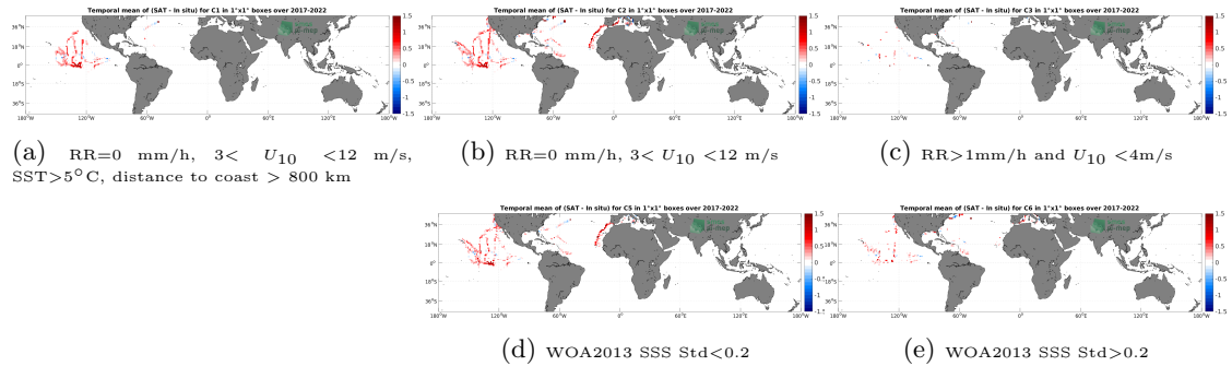
Figure 12: Temporal mean gridded over spatial boxes of size 1^\circ \times 1^\circ of \Delta SSS (SMAP SSS L3 v5.0 - 8-Day running (JPL) - Saildrone) for 5 different subdatasets corresponding to:RR=0 mm/h, 3 < U_{10} < 12 m/s, SST>5°C, distance to coast > 800 km (a), RR=0 mm/h, 3 < U_{10} < 12 m/s (b), RR>1mm/h and U_{10} < 4 m/s (c), WOA2013 SSS Std<0.2 (d), WOA2013 SSS Std>0.2 (e).
