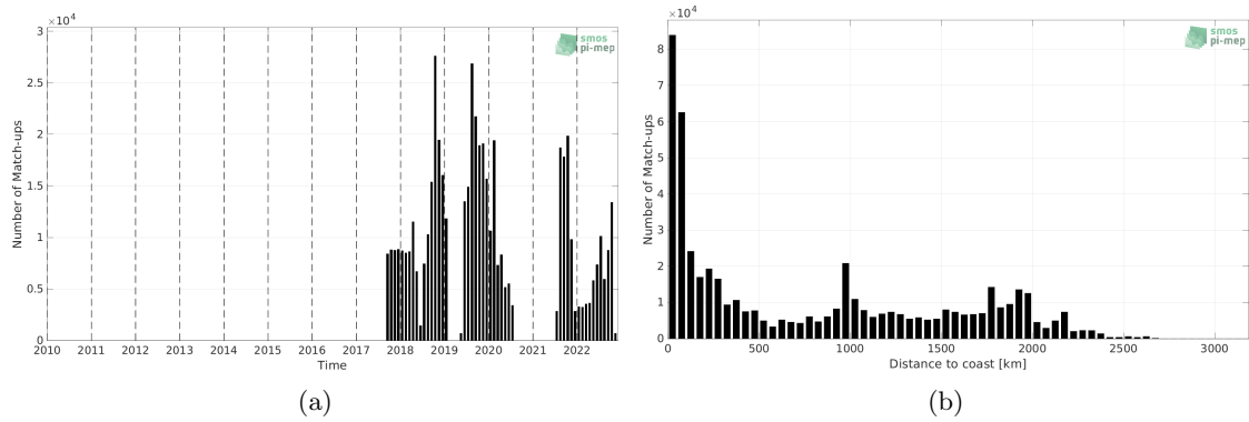
Figure 1: Number of match-ups between Sairdrone and SMAP SSS L3 v5.0 - 8-Day running (JPL) SSS as a function of time (a) and as function of the distance to coast (b) over the Mid-Low Latitudes 45N-45S Pi-MEP region and for the full satellite product period.
