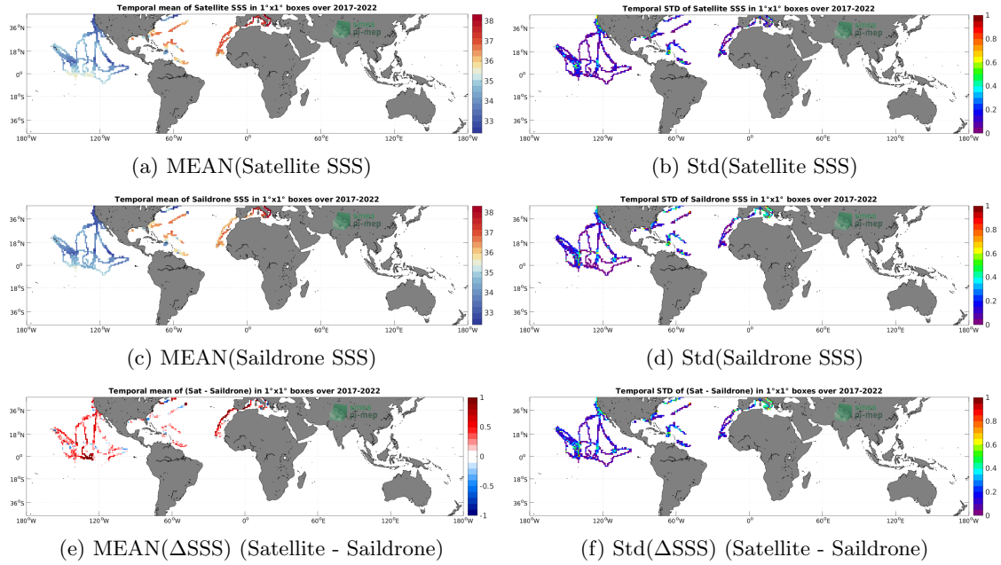
Figure 6: Temporal mean (left) and Std (right) of SSS from SMAP SSS L3 v5.0 - 8-Day running (JPL) (top), Saildrone (middle), and of \Delta SSS (Satellite - Saildrone). Only match-up pairs are used to generate these maps.
