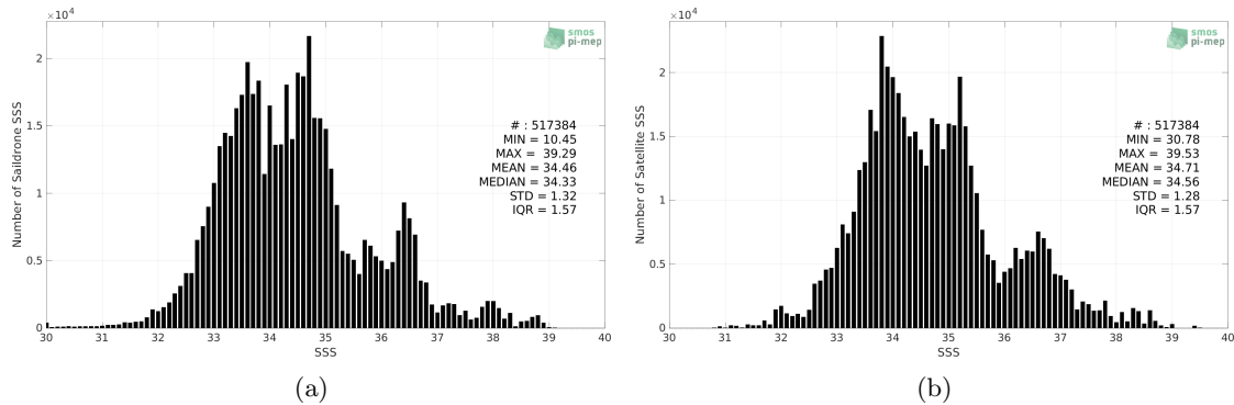
Figure 2: Histograms of SSS from Sairdrone (a) and SMAP SSS L3 v5.0 - 8-Day running (JPL) (b) considering all match-up pairs per bins of 0.1 over the Mid-Low Latitudes 45N-45S Pi-MEP region and for the full satellite product period.
