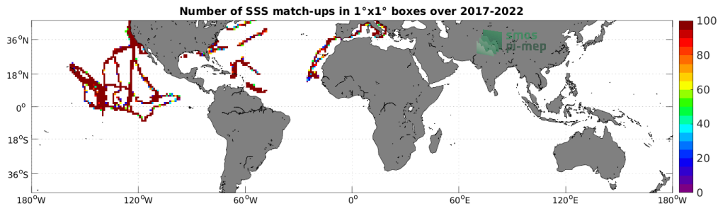
Figure 4: Number of SSS match-ups between Saildrone SSS and the SMAP SSS L3 v5.0 - 8-Day running (JPL) SSS product for the Mid-Low Latitudes 45N-45S Pi-MEP region over 1^\circ \times 1^\circ boxes and for the full satellite product period.
