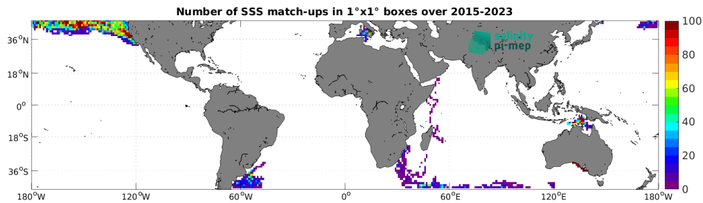
Figure 5: Number of SSS match-ups between Marine mammals SSS and the SMAP SSS L3 v5.0 - 8-Day running (JPL) SSS product for the Mid-Low Latitudes 45N-45S Pi-MEP region over 1^\circ \times 1^\circ boxes and for the full satellite product period.
