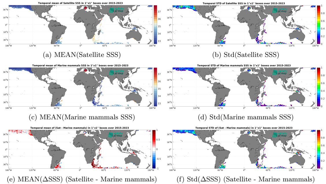
Figure 7: Temporal mean (left) and Std (right) of SSS from SMAP SSS L3 v5.0 - 8-Day running (JPL) (top), Marine mammals (middle), and of \Delta SSS (Satellite - Marine mammals). Only match-up pairs are used to generate these maps.
