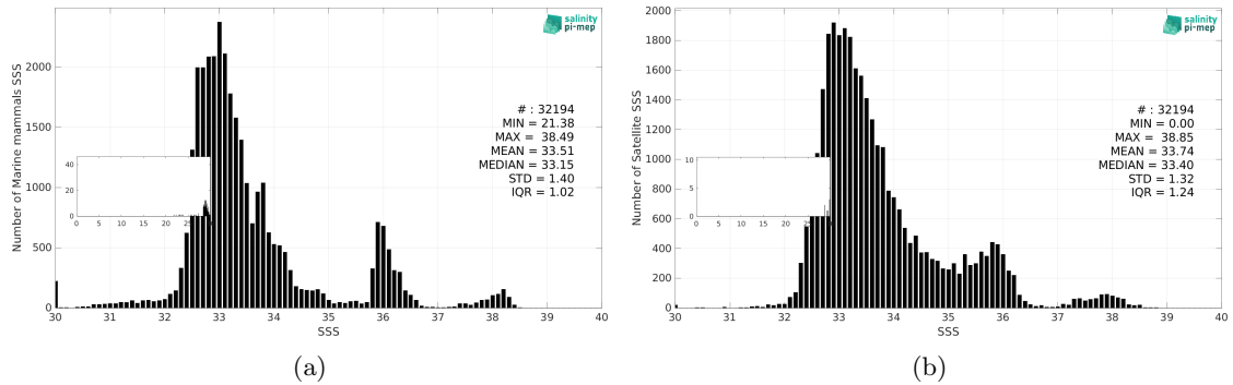
Figure 3: Histograms of SSS from Marine mammals (a) and SMAP SSS L3 v5.0 - 8-Day running (JPL) (b) considering all match-up pairs per bins of 0.1 over the Mid-Low Latitudes 45N-45S Pi-MEP region and for the full satellite product period.
