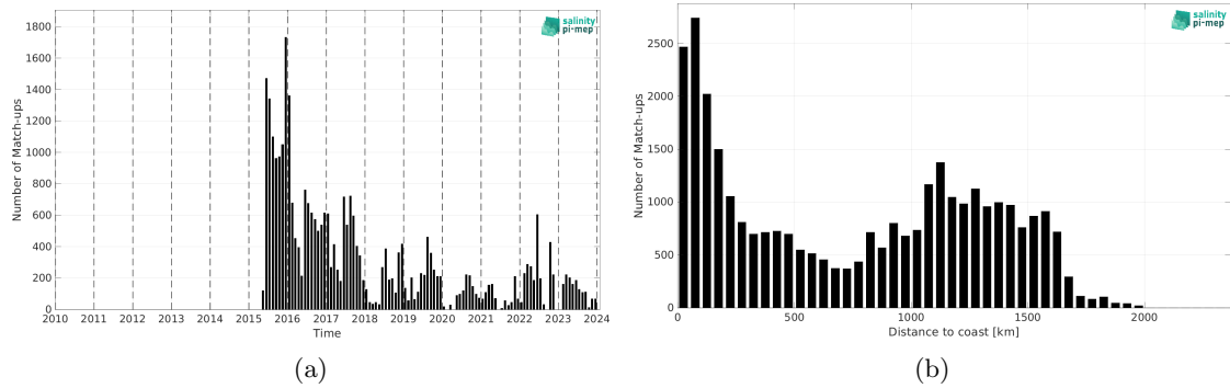
Figure 2: Number of match-ups between Marine mammals and SMAP SSS L3 v5.0 - 8-Day running (JPL) SSS as a function of time (a) and as function of the distance to coast (b) over the Mid-Low Latitudes 45N-45S Pi-MEP region and for the full satellite product period.
