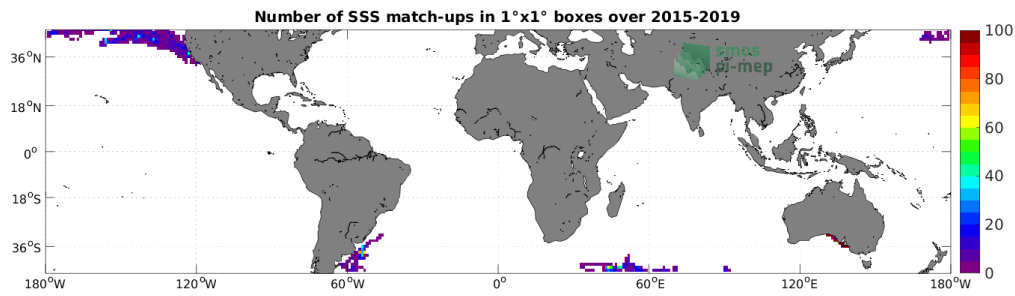
Figure 4: Number of SSS match-ups between Marine mammals SSS and the SMAP SSS L3 v5.0 - 8-Day running (JPL) SSS product for the Mid-Low Latitudes 45N-45S Pi-MEP region over 1°×1° boxes and for the full satellite product period.
