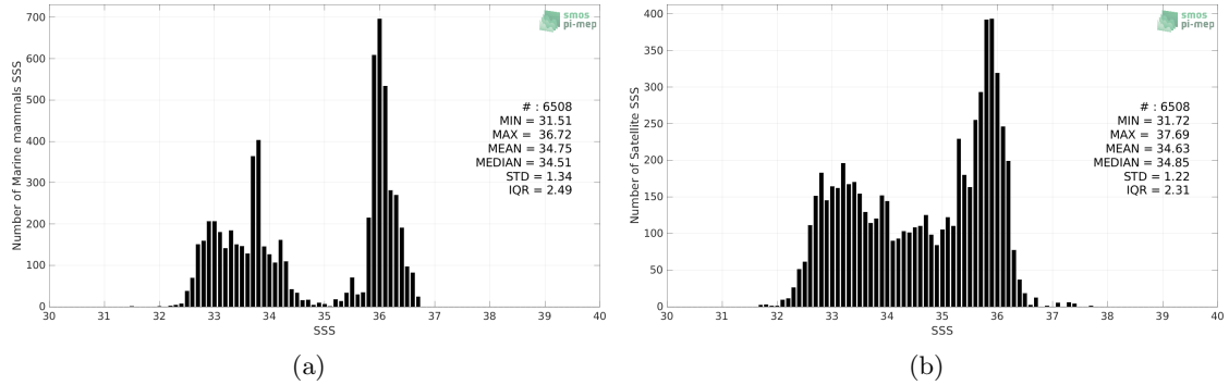
Figure 2: Histograms of SSS from Marine mammals (a) and SMAP SSS L3 v5.0 - 8-Day running (JPL) (b) considering all match-up pairs per bins of 0.1 over the Mid-Low Latitudes 45N-45S Pi-MEP region and for the full satellite product period.
