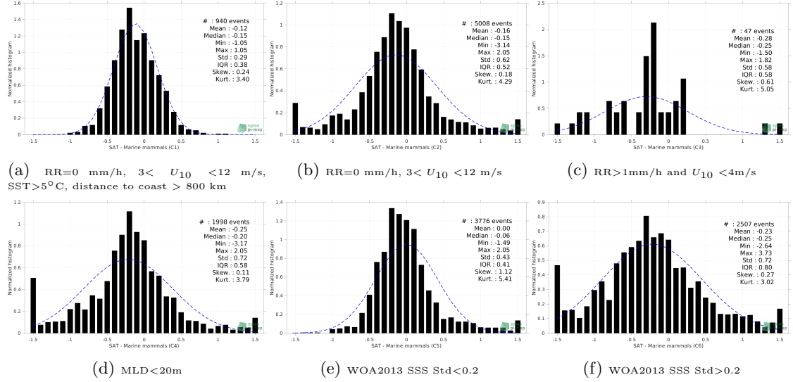
Figure 13: Normalized histogram of \Delta SSS (SMAP SSS L3 v5.0 - 8-Day running (JPL) - Marine mammals) for 6 different subdatasets corresponding to: RR=0 mm/h, 3 < U_{10} < 12 m/s, SST>5°C, distance to coast > 800 km (a), RR=0 mm/h, 3 < U_{10} < 12 m/s (b), RR>1mm/h and U_{10} < 4 m/s (c), MLD<20m (d), WOA2013 SSS Std<0.2 (e), WOA2013 SSS Std>0.2 (f).
