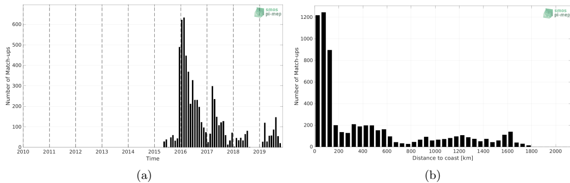
Figure 1: Number of match-ups between Marine mammals and SMAP SSS L3 v5.0 - 8-Day running (JPL) SSS as a function of time (a) and as function of the distance to coast (b) over the Mid-Low Latitudes 45N-45S Pi-MEP region and for the full satellite product period.
