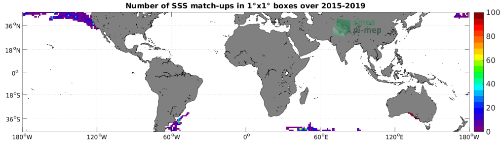
Figure 4: Number of SSS match-ups between Marine mammals SSS and the SMAP SSS L3 v5.0 - 8-Day running (JPL) SSS product for the Mid-Low Latitudes 45N-45S Pi-MEP region over 1^\circ \times 1^\circ boxes and for the full satellite product period.
