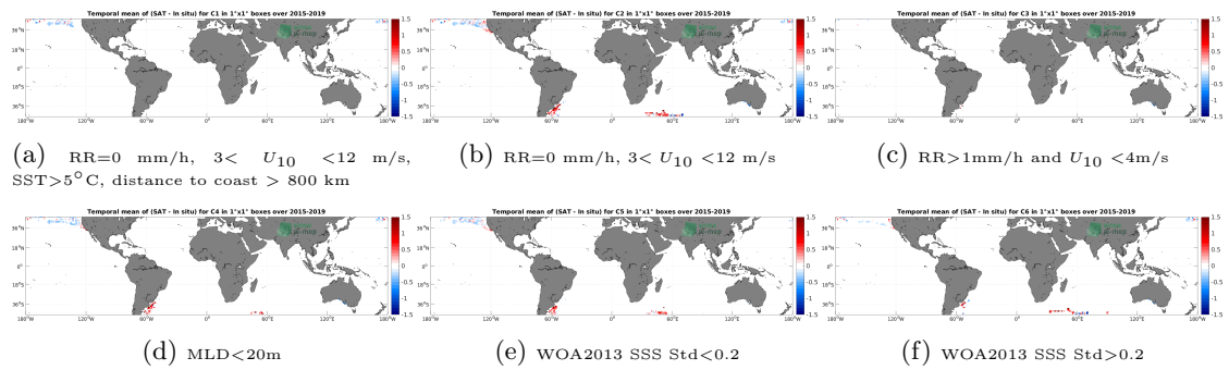
Figure 12: Temporal mean gridded over spatial boxes of size 1^\circ \times 1^\circ of \Delta SSS (SMAP SSS L3 v5.0 - 8-Day running (JPL) - Marine mammals) for 6 different subdatasets corresponding to:RR=0 mm/h, 3 < U_{10} < 12 m/s, SST > 5°C, distance to coast > 800 km (a), RR=0 mm/h, 3 < U_{10} < 12 m/s (b), RR > 1mm/h and U_{10} < 4 m/s (c),MLD < 20m (d),WOA2013 SSS Std < 0.2 (e),WOA2013 SSS Std > 0.2 (f).
