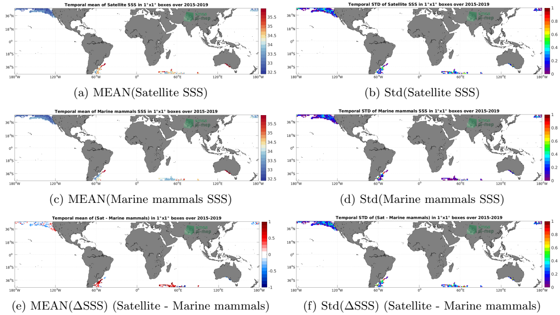
Figure 6: Temporal mean (left) and Std (right) of SSS from SMAP SSS L3 v5.0 - 8-Day running (JPL) (top), Marine mammals (middle), and of \Delta SSS (Satellite - Marine mammals). Only match-up pairs are used to generate these maps.
