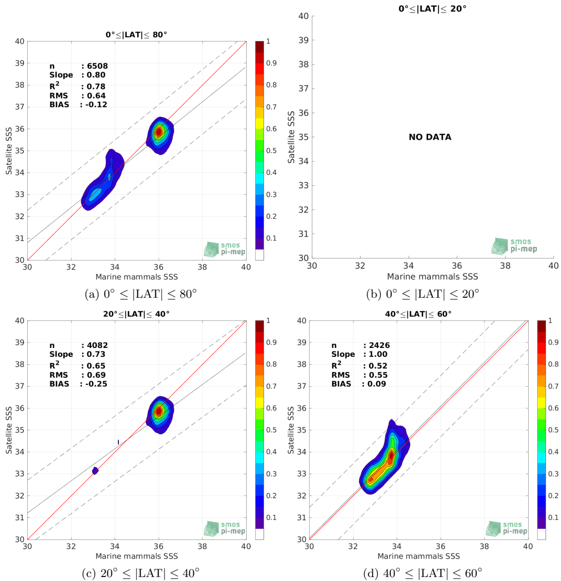
Figure 9: Contour maps of the concentration of SMAP SSS L3 v5.0 - 8-Day running (JPL) SSS (y-axis) versus Marine mammals SSS (x-axis) at match-up pairs for different latitude bands. For each plot, the red line shows x=y . The black thin and dashed lines indicate a linear fit through the data cloud and the \pm 95\% confidence levels, respectively. The number match-up pairs n , the slope and R^2 coefficient of the linear fit, the root mean square (RMS) and the mean bias between satellite and in situ data are indicated for each latitude band in each plots.
