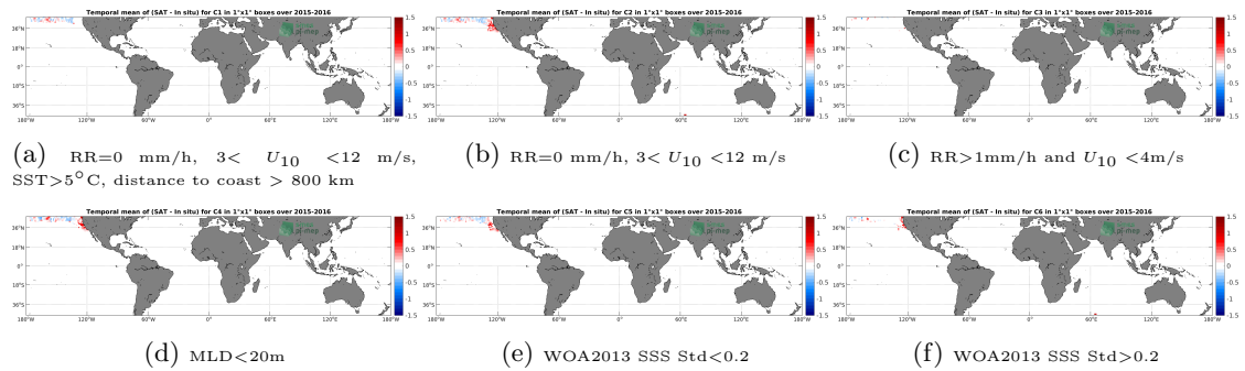
Figure 12: Temporal mean gridded over spatial boxes of size 1^\circ \times 1^\circ of \Delta SSS (SMAP SSS L3 v5.0 - 8-Day running (JPL) - Sea mammals) for 6 different subdatasets corresponding to:RR=0 mm/h, 3 < U_{10} < 12 m/s, SST > 5^\circ C , distance to coast > 800 km (a), RR=0 mm/h, 3 < U_{10} < 12 m/s (b), RR>1mm/h and U_{10} < 4 m/s (c),MLD<20m (d),WOA2013 SSS Std<0.2 (e),WOA2013 SSS Std>0.2 (f).
