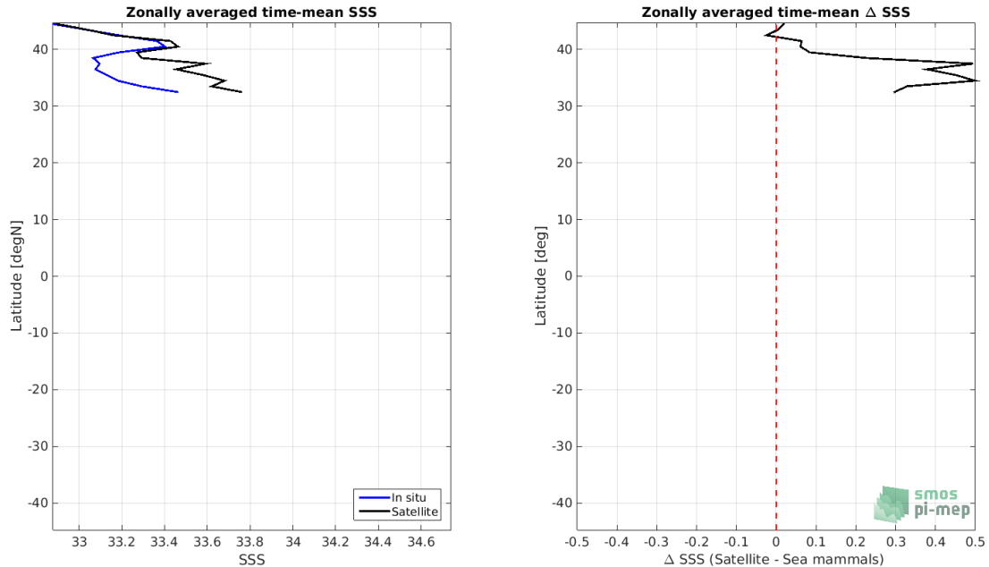
Figure 8: Left panel: Zonal mean SSS from SMAP SSS L3 v5.0 - 8-Day running (JPL) satellite product (black) and from Sea mammals (blue). Right panel: Zonal mean of \Delta SSS (Satellite - Sea mammals) for all the collected Pi-MEP match-up pairs estimated over the full satellite product period.
