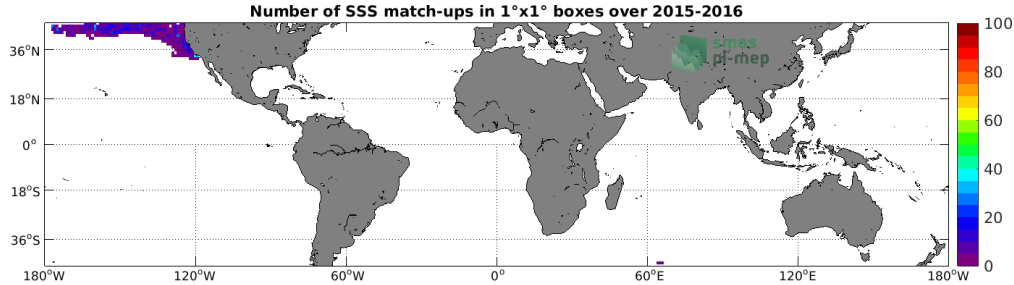
Figure 4: Number of SSS match-ups between Sea mammals SSS and the SMAP SSS L3 v5.0 - 8-Day running (JPL) SSS product for the Mid-Low Latitudes 45N-45S Pi-MEP region over 1^\circ \times 1^\circ boxes and for the full satellite product period.
