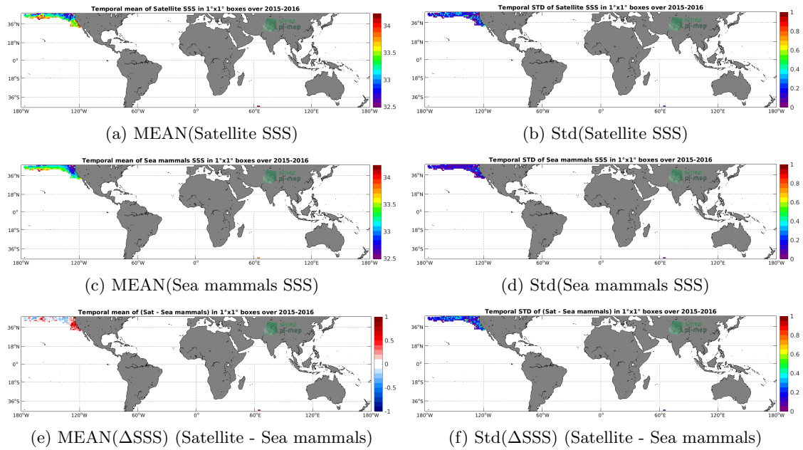
Figure 6: Temporal mean (left) and Std (right) of SSS from SMAP SSS L3 v5.0 - 8-Day running (JPL) (top), Sea mammals (middle), and of \Delta SSS (Satellite - Sea mammals). Only match-up pairs are used to generate these maps.
