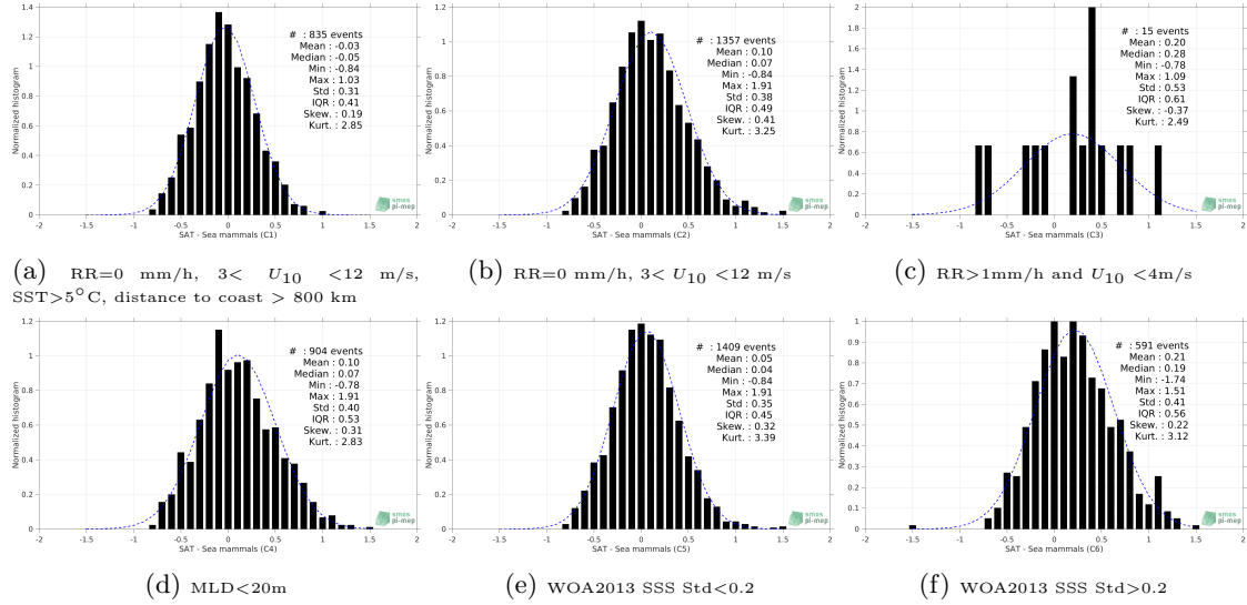
Figure 13: Normalized histogram of \Delta SSS (SMAP SSS L3 v5.0 - 8-Day running (JPL) - Sea mammals) for 6 different subdatasets corresponding to: RR=0 mm/h, 3 < U_{10} < 12 m/s, SST>5°C, distance to coast > 800 km (a), RR=0 mm/h, 3 < U_{10} < 12 m/s (b), RR>1mm/h and U_{10} < 4 m/s (c), MLD<20m (d), WOA2013 SSS Std<0.2 (e), WOA2013 SSS Std>0.2 (f).
