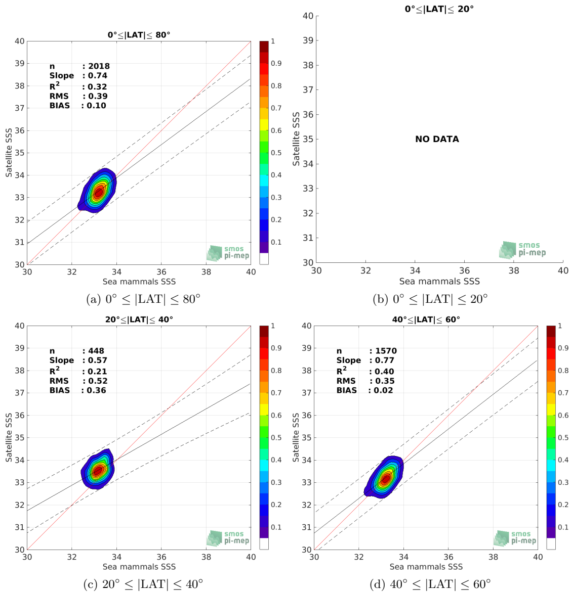
Figure 9: Contour maps of the concentration of SMAP SSS L3 v5.0 - 8-Day running (JPL) SSS (y-axis) versus Sea mammals SSS (x-axis) at match-up pairs for different latitude bands. For each plot, the red line shows x=y . The black thin and dashed lines indicate a linear fit through the data cloud and the \pm 95\% confidence levels, respectively. The number match-up pairs n , the slope and R^2 coefficient of the linear fit, the root mean square (RMS) and the mean bias between satellite and in situ data are indicated for each latitude band in each plots.
