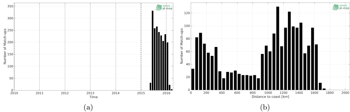
Figure 1: Number of match-ups between Sea mammals and SMAP SSS L3 v5.0 - 8-Day running (JPL) SSS as a function of time (a) and as function of the distance to coast (b) over the Mid-Low Latitudes 45N-45S Pi-MEP region and for the full satellite product period.
