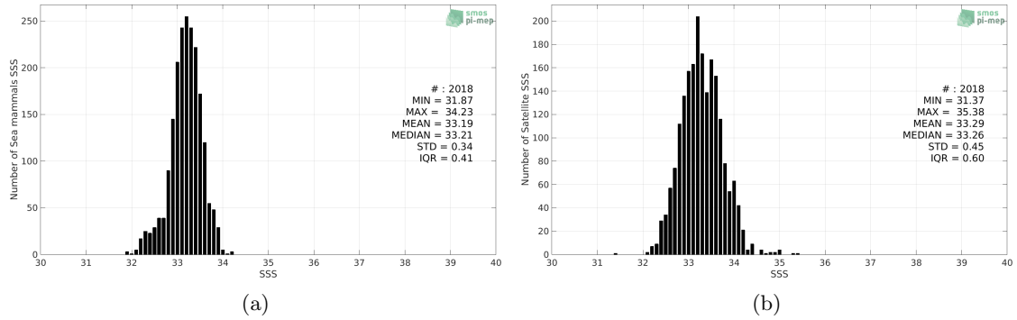
Figure 2: Histograms of SSS from Sea mammals (a) and SMAP SSS L3 v5.0 - 8-Day running (JPL) (b) considering all match-up pairs per bins of 0.1 over the Mid-Low Latitudes 45N-45S Pi-MEP region and for the full satellite product period.
