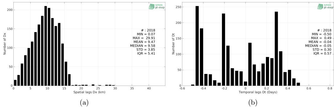
Figure 5: Histograms of the spatial (a) and temporal (b) lags between the time of the Sea mammals measurements and the date of the corresponding SMAP SSS L3 v5.0 - 8-Day running (JPL) SSS product.
