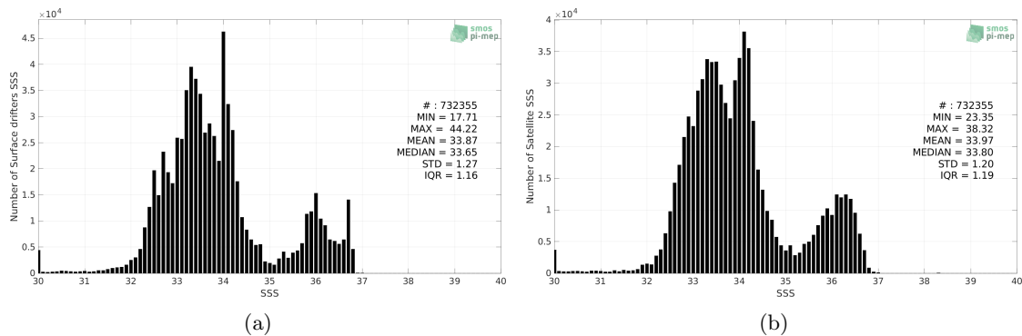
Figure 2: Histograms of SSS from Surface drifters (a) and SMAP SSS L3 v5.0 - 8-Day running (JPL) (b) considering all match-up pairs per bins of 0.1 over the Mid-Low Latitudes 45N-45S Pi-MEP region and for the full satellite product period.
