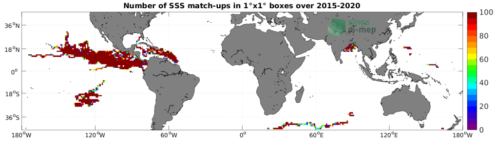
Figure 3: Number of SSS match-ups between Surface drifters SSS and the SMAP SSS L3 v5.0 - 8-Day running (JPL) SSS product for the Mid-Low Latitudes 45N-45S Pi-MEP region over 1^\circ \times 1^\circ boxes and for the full satellite product period.
