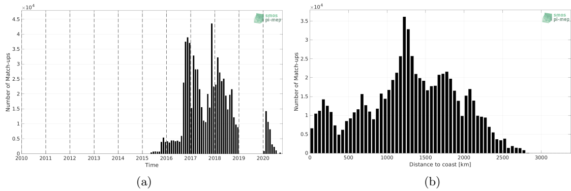
Figure 1: Number of match-ups between Surface drifters and SMAP SSS L3 v5.0 - 8-Day running (JPL) SSS as a function of time (a) and as function of the distance to coast (b) over the Mid-Low Latitudes 45N-45S Pi-MEP region and for the full satellite product period.
