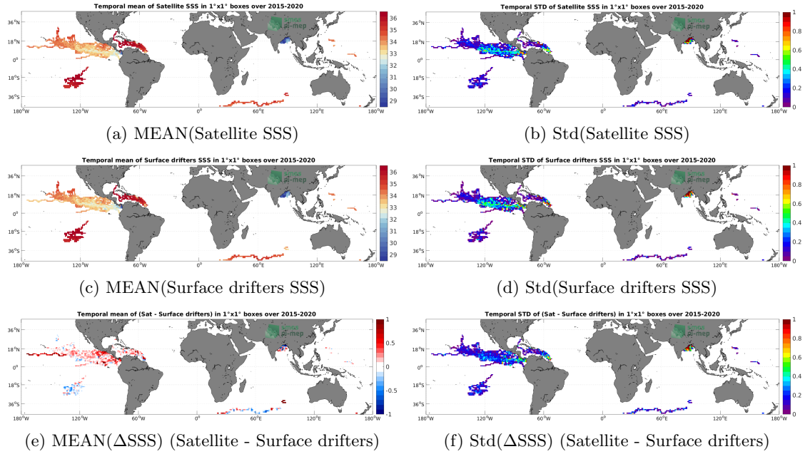
Figure 5: Temporal mean (left) and Std (right) of SSS from SMAP SSS L3 v5.0 - 8-Day running (JPL) (top), Surface drifters (middle), and of \Delta SSS (Satellite - Surface drifters). Only match-up pairs are used to generate these maps.
