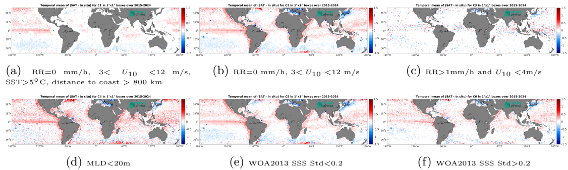
Figure 14: Temporal mean gridded over spatial boxes of size 1^\circ \times 1^\circ of \Delta SSS (SMAP SSS L3 v5.0 - 8-Day running (JPL) - Argo) for 6 different subdatasets corresponding to:RR=0 mm/h, 3 < U_{10} < 12 m/s, SST>5°C, distance to coast > 800 km (a), RR=0 mm/h, 3 < U_{10} < 12 m/s (b), RR>1mm/h and U_{10} < 4 m/s (c),MLD<20m (d),WOA2013 SSS Std<0.2 (e),WOA2013 SSS Std>0.2 (f).
