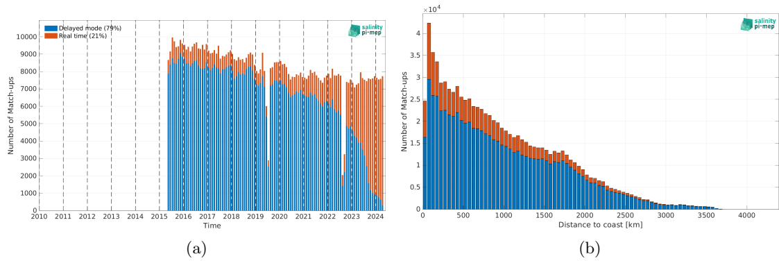
Figure 2: Number of match-ups between Argo and SMAP SSS L3 v5.0 - 8-Day running (JPL) SSS as a function of time (a) and as function of the distance to coast (b) over the Mid-Low Latitudes 45N-45S Pi-MEP region and for the full satellite product period.
