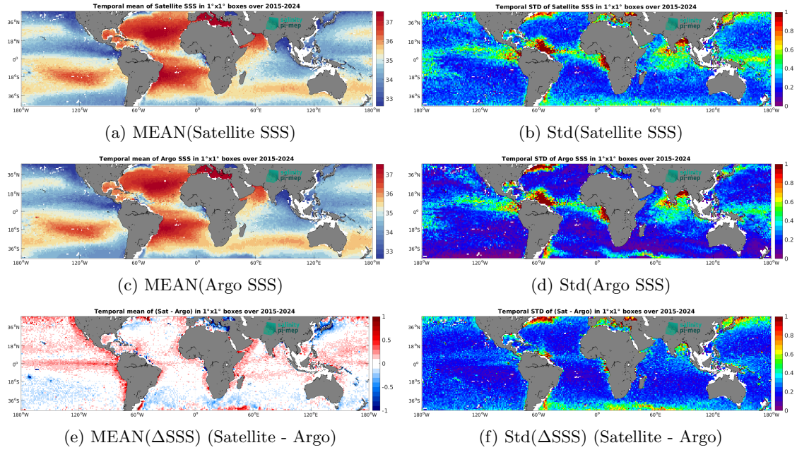
Figure 7: Temporal mean (left) and Std (right) of SSS from SMAP SSS L3 v5.0 - 8-Day running (JPL) (top), Argo (middle), and of \Delta SSS (Satellite - Argo). Only match-up pairs are used to generate these maps.
