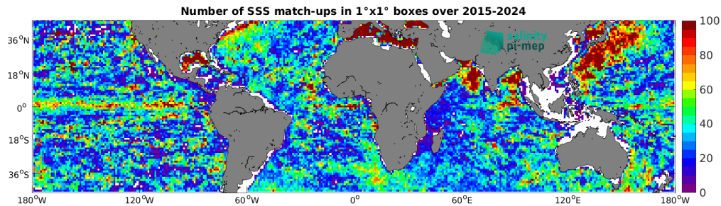
Figure 5: Number of SSS match-ups between Argo SSS and the SMAP SSS L3 v5.0 - 8-Day running (JPL) SSS product for the Mid-Low Latitudes 45N-45S Pi-MEP region over 1^\circ \times 1^\circ boxes and for the full satellite product period.
