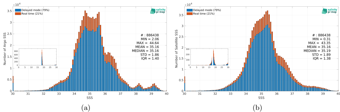
Figure 3: Histograms of SSS from Argo (a) and SMAP SSS L3 v5.0 - 8-Day running (JPL) (b) considering all match-up pairs per bins of 0.1 over the Mid-Low Latitudes 45N-45S Pi-MEP region and for the full satellite product period.
