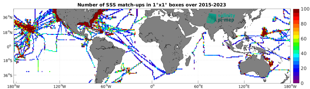
Figure 5: Number of SSS match-ups between TSG (SAMOS) SSS and the SMAP SSS L3 v5.0 - Monthly (JPL) SSS product for the Mid-Low Latitudes 45N-45S Pi-MEP region over 1^\circ \times 1^\circ boxes and for the full satellite product period.
