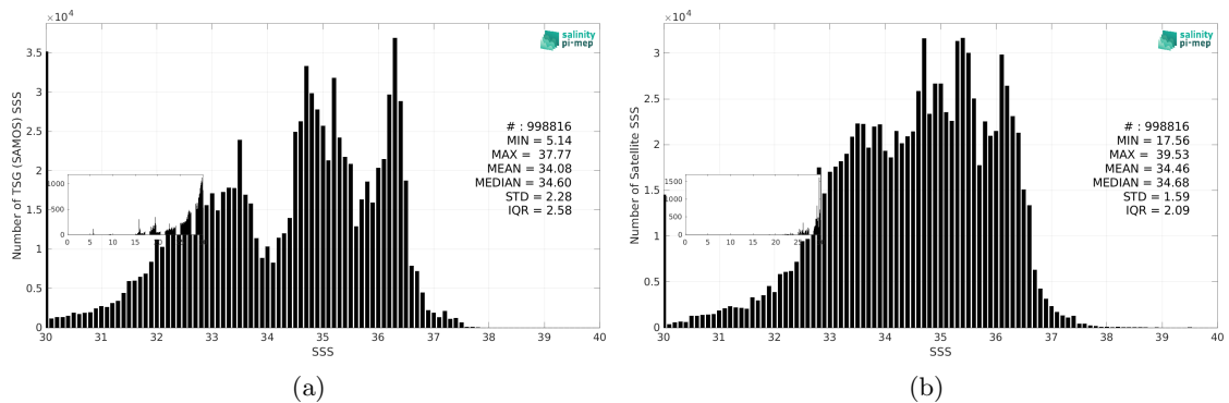
Figure 3: Histograms of SSS from TSG (SAMOS) (a) and SMAP SSS L3 v5.0 - Monthly (JPL) (b) considering all match-up pairs per bins of 0.1 over the Mid-Low Latitudes 45N-45S Pi-MEP region and for the full satellite product period.
