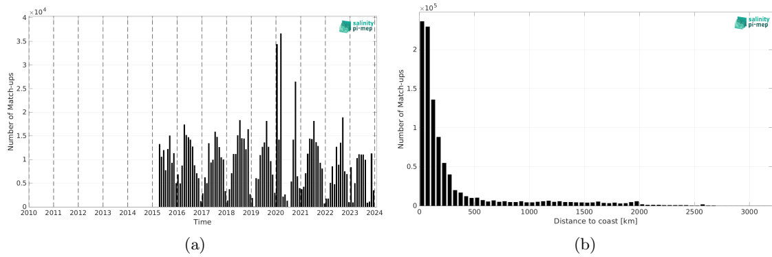
Figure 2: Number of match-ups between TSG (SAMOS) and SMAP SSS L3 v5.0 - Monthly (JPL) SSS as a function of time (a) and as function of the distance to coast (b) over the Mid-Low Latitudes 45N-45S Pi-MEP region and for the full satellite product period.
