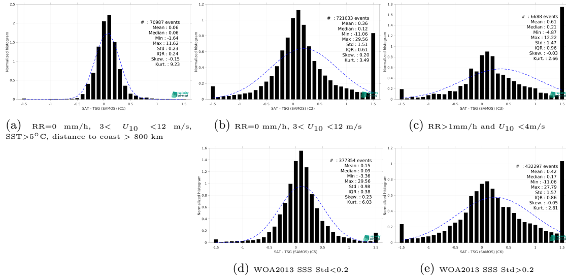
Figure 15: Normalized histogram of \Delta SSS (SMAP SSS L3 v5.0 - Monthly (JPL) - TSG (SAMOS)) for 5 different subdatasets corresponding to: RR=0 mm/h, 3 < U_{10} < 12 m/s, SST>5°C, distance to coast > 800 km (a), RR=0 mm/h, 3 < U_{10} < 12 m/s (b), RR>1mm/h and U_{10} < 4 m/s (c), WOA2013 SSS Std<0.2 (d), WOA2013 SSS Std>0.2 (e).
