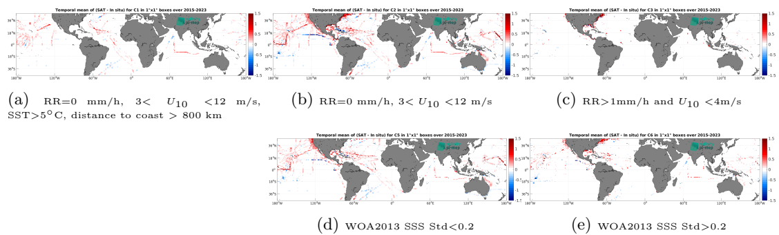
Figure 14: Temporal mean gridded over spatial boxes of size 1^\circ \times 1^\circ of \Delta\text{SSS} (SMAP SSS L3 v5.0 - Monthly (JPL) - TSG (SAMOS)) for 5 different subdatasets corresponding to: RR=0 mm/h, 3 < U_{10} < 12 m/s, SST > 5°C, distance to coast > 800 km (a), RR=0 mm/h, 3 < U_{10} < 12 m/s (b), RR > 1mm/h and U_{10} < 4 m/s (c), WOA2013 SSS Std < 0.2 (d), WOA2013 SSS Std > 0.2 (e).
