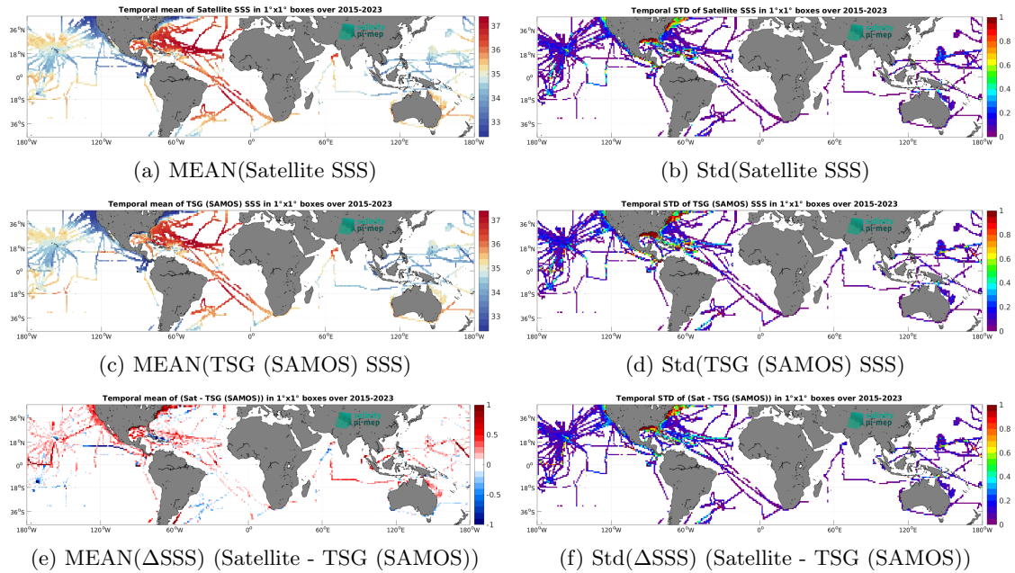
Figure 7: Temporal mean (left) and Std (right) of SSS from SMAP SSS L3 v5.0 - Monthly (JPL) (top), TSG (SAMOS) (middle), and of \Delta SSS (Satellite - TSG (SAMOS)). Only match-up pairs are used to generate these maps.
