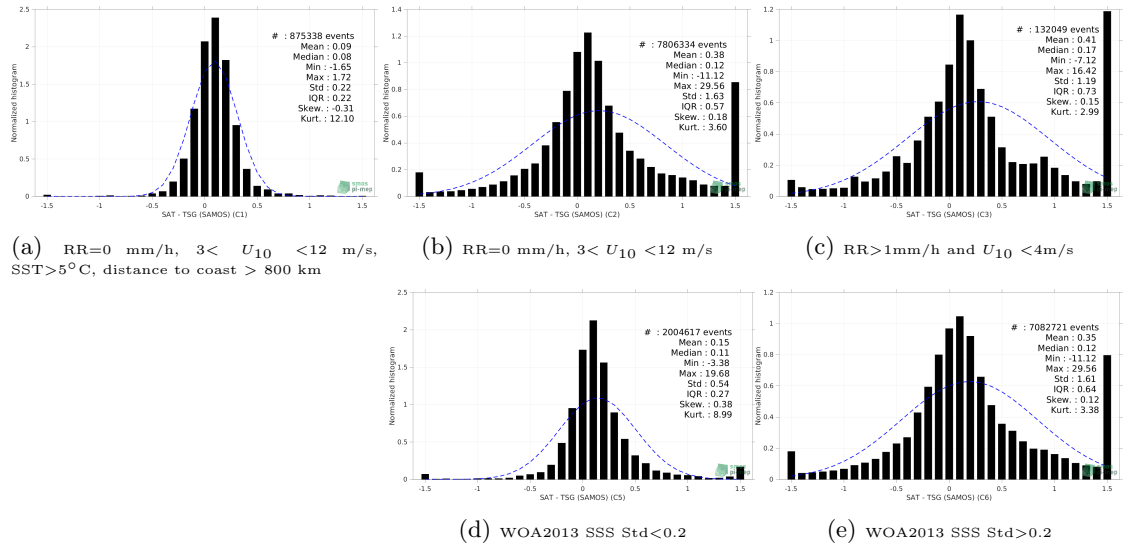
Figure 13: Normalized histogram of \Delta SSS (SMAP SSS L3 v5.0 - Monthly (JPL) - TSG (SAMOS)) for 5 different subdatasets corresponding to: RR=0 mm/h, 3 < U_{10} < 12 m/s, SST >5^\circ\text{C} , distance to coast > 800 km (a), RR=0 mm/h, 3 < U_{10} < 12 m/s (b), RR >1 mm/h and U_{10} < 4 m/s (c), WOA2013 SSS Std <0.2 (d), WOA2013 SSS Std >0.2 (e).
