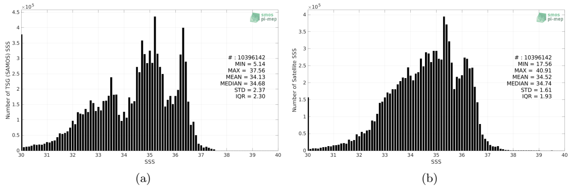
Figure 2: Histograms of SSS from TSG (SAMOS) (a) and SMAP SSS L3 v5.0 - Monthly (JPL) (b) considering all match-up pairs per bins of 0.1 over the Mid-Low Latitudes 45N-45S Pi-MEP region and for the full satellite product period.
