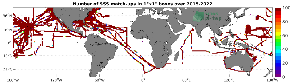
Figure 4: Number of SSS match-ups between TSG (SAMOS) SSS and the SMAP SSS L3 v5.0 - Monthly (JPL) SSS product for the Mid-Low Latitudes 45N-45S Pi-MEP region over 1^\circ \times 1^\circ boxes and for the full satellite product period.
