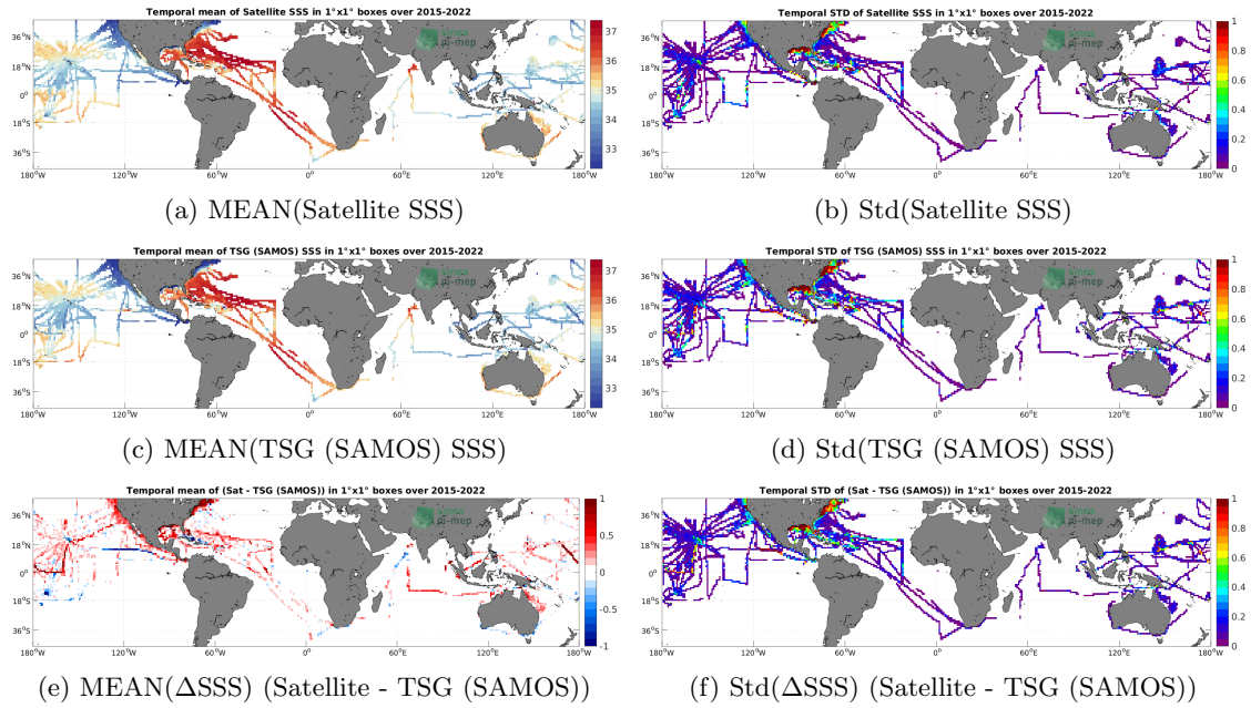
Figure 6: Temporal mean (left) and Std (right) of SSS from SMAP SSS L3 v5.0 - Monthly (JPL) (top), TSG (SAMOS) (middle), and of \Delta SSS (Satellite - TSG (SAMOS)). Only match-up pairs are used to generate these maps.
