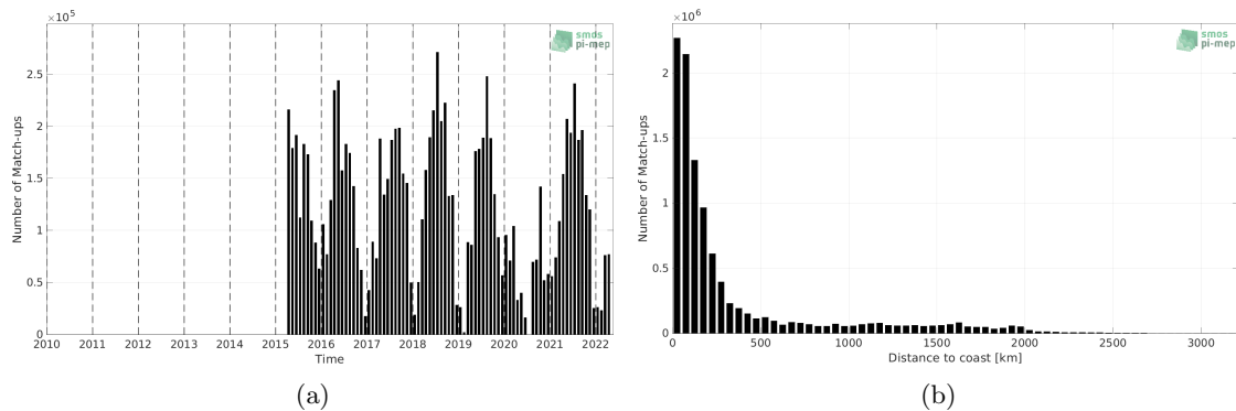
Figure 1: Number of match-ups between TSG (SAMOS) and SMAP SSS L3 v5.0 - Monthly (JPL) SSS as a function of time (a) and as function of the distance to coast (b) over the Mid-Low Latitudes 45N-45S Pi-MEP region and for the full satellite product period.
