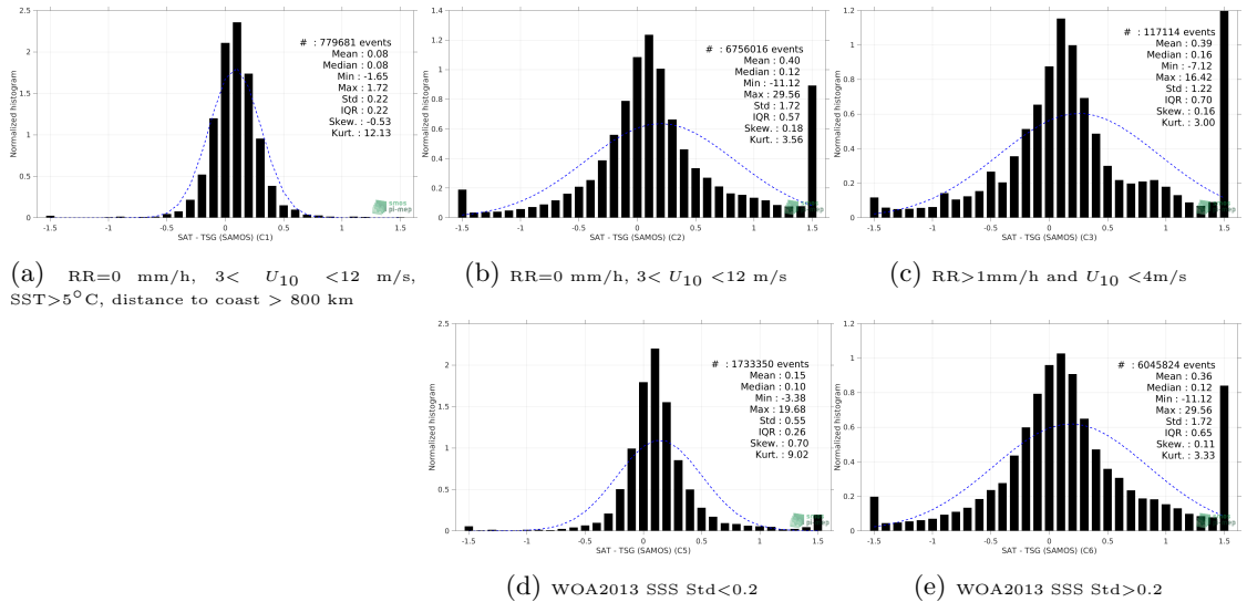
Figure 13: Normalized histogram of \Delta SSS (SMAP SSS L3 v5.0 - Monthly (JPL) - TSG (SAMOS)) for 5 different subdatasets corresponding to: RR=0 mm/h, 3 < U_{10} < 12 m/s, SST > 5^\circ C , distance to coast > 800 km (a), RR=0 mm/h, 3 < U_{10} < 12 m/s (b), RR>1mm/h and U_{10} < 4 m/s (c), WOA2013 SSS Std<0.2 (d), WOA2013 SSS Std>0.2 (e).
