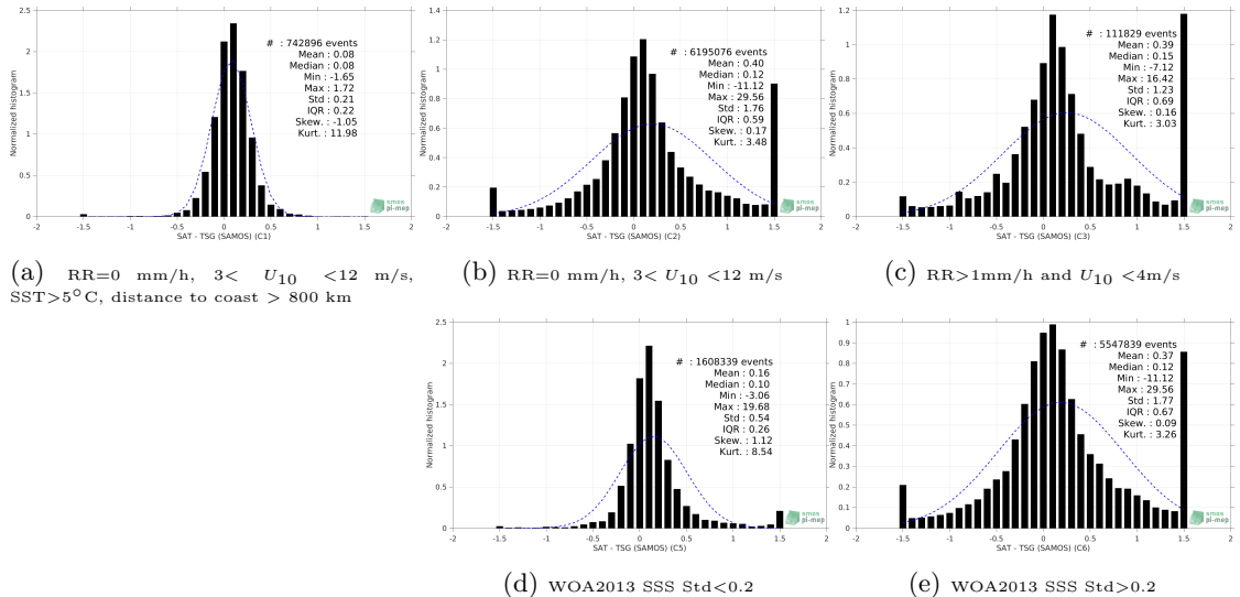
Figure 13: Normalized histogram of ΔSSS (SMAP SSS L3 v5.0 - Monthly (JPL) - TSG (SAMOS)) for 5 different subdatasets corresponding to: RR=0 mm/h, 3 < U 10 < 12 m/s, SST>5°C, distance to coast > 800 km (a), RR=0 mm/h, 3 < U 10 < 12 m/s (b), RR>1mm/h and U 10 <4m/s (c), WOA2013 SSS Std<0.2 (d), WOA2013 SSS Std>0.2 (e).
