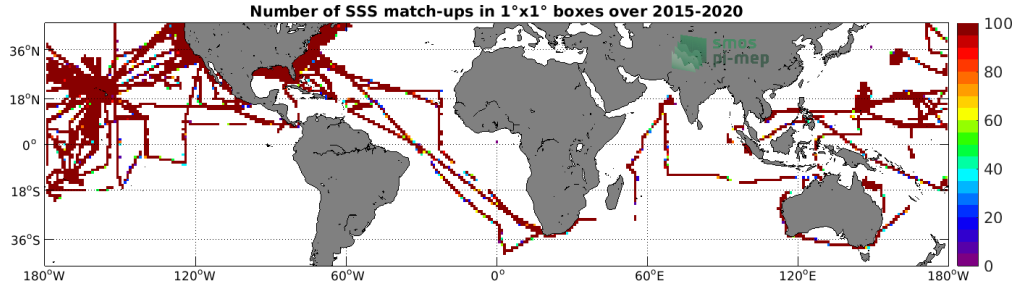
Figure 4: Number of SSS match-ups between TSG (SAMOS) SSS and the SMAP SSS L3 v5.0 - Monthly (JPL) SSS product for the Mid-Latitudes 45N-45S Pi-MEP region over 1^\circ \times 1^\circ boxes and for the full satellite product period.
