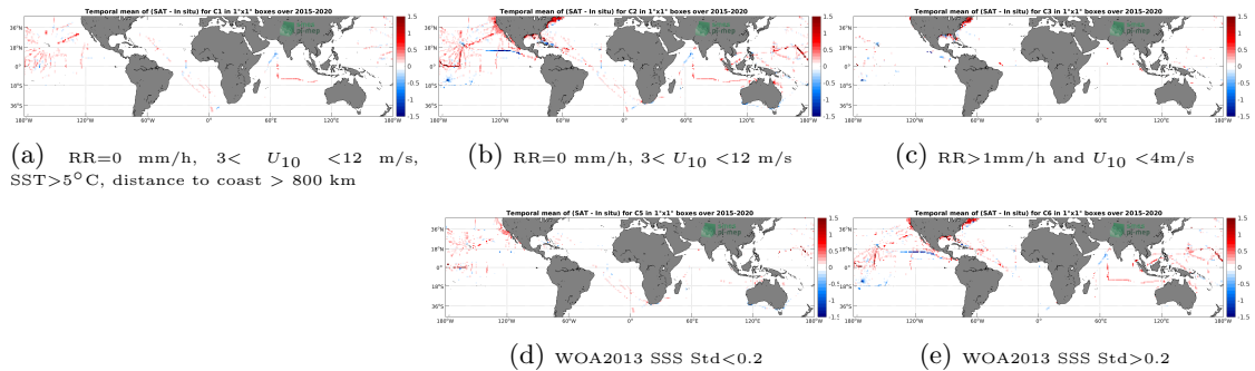
Figure 12: Temporal mean gridded over spatial boxes of size 1°x1° of ΔSSS (SMAP SSS L3 v5.0 - Monthly (JPL) - TSG (SAMOS)) for 5 different subdatasets corresponding to:RR=0 mm/h, 3 < U 10 < 12 m/s, SST>5°C, distance to coast > 800 km (a), RR=0 mm/h, 3 < U 10 < 12 m/s (b), RR>1mm/h and U 10 <4m/s (c), WOA2013 SSS Std<0.2 (d), WOA2013 SSS Std>0.2 (e).
