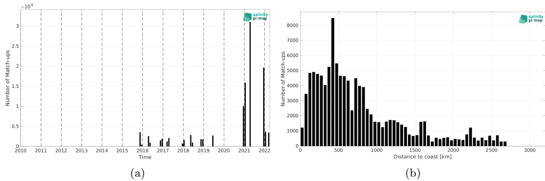
Figure 1: Number of match-ups between TSG (Polarstern) and SMAP SSS L3 v5.0 - Monthly (JPL) SSS as a function of time (a) and as function of the distance to coast (b) over the Mid-Low Latitudes 45N-45S Pi-MEP region and for the full satellite product period.
