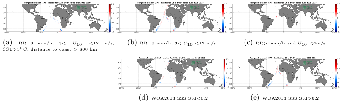
Figure 12: Temporal mean gridded over spatial boxes of size 1^\circ \times 1^\circ of \Delta SSS (SMAP SSS L3 v5.0 - Monthly (JPL) - TSG (Polarstern)) for 5 different subdatasets corresponding to: RR=0 mm/h, 3 < U_{10} < 12 m/s, SST>5°C, distance to coast > 800 km (a), RR=0 mm/h, 3 < U_{10} < 12 m/s (b), RR>1mm/h and U_{10} < 4 m/s (c), WOA2013 SSS Std<0.2 (d), WOA2013 SSS Std>0.2 (e).
