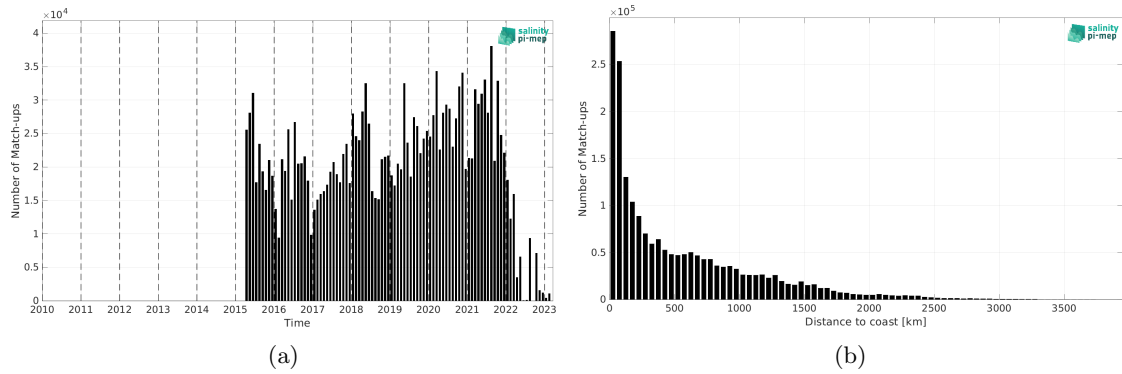
Figure 2: Number of match-ups between TSG (LEGOS-DM) and SMAP SSS L3 v5.0 - Monthly (JPL) SSS as a function of time (a) and as function of the distance to coast (b) over the Mid-Low Latitudes 45N-45S Pi-MEP region and for the full satellite product period.
