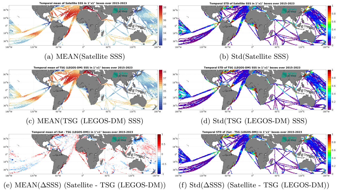
Figure 7: Temporal mean (left) and Std (right) of SSS from SMAP SSS L3 v5.0 - Monthly (JPL) (top), TSG (LEGOS-DM) (middle), and of \Delta SSS (Satellite - TSG (LEGOS-DM)). Only match-up pairs are used to generate these maps.
