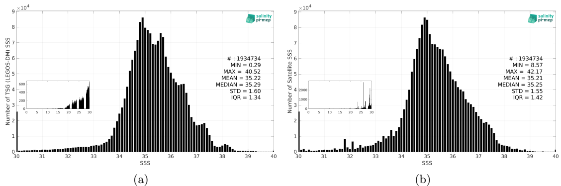
Figure 3: Histograms of SSS from TSG (LEGOS-DM) (a) and SMAP SSS L3 v5.0 - Monthly (JPL) (b) considering all match-up pairs per bins of 0.1 over the Mid-Low Latitudes 45N-45S Pi-MEP region and for the full satellite product period.
