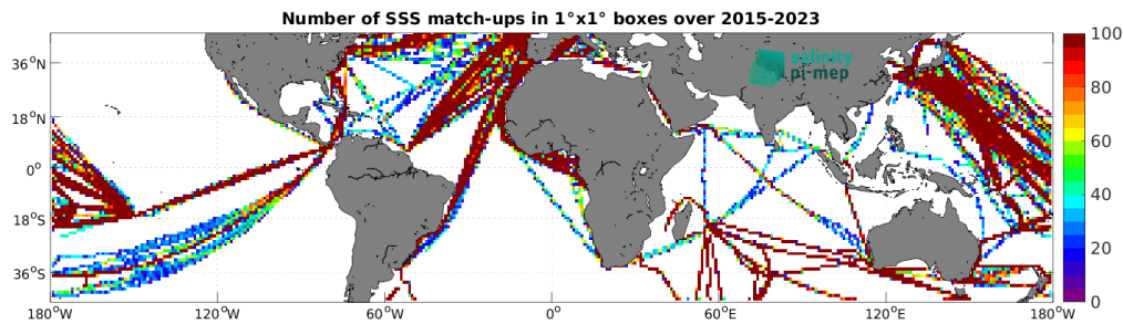
Figure 5: Number of SSS match-ups between TSG (LEGOS-DM) SSS and the SMAP SSS L3 v5.0 - Monthly (JPL) SSS product for the Mid-Low Latitudes 45N-45S Pi-MEP region over 1^\circ \times 1^\circ boxes and for the full satellite product period.
