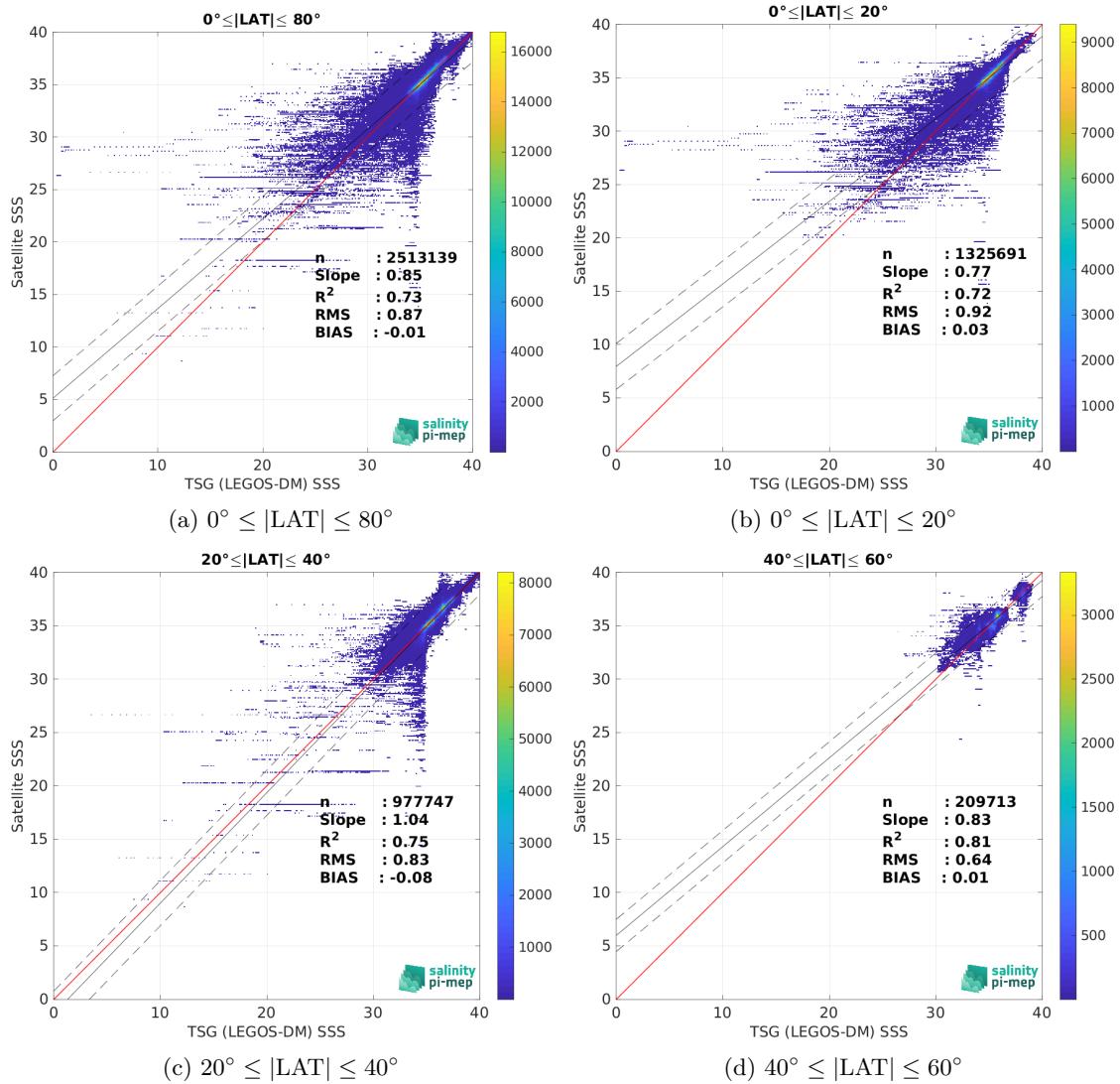
Figure 9: Contour maps of the concentration of SMAP SSS L3 v5.0 - Monthly (JPL) SSS (y-axis) versus TSG (LEGOS-DM) SSS (x-axis) at match-up pairs for different latitude bands. For each plot, the red line shows x=y . The black thin and dashed lines indicate a linear fit through the data cloud and the \pm 95\% confidence levels, respectively. The number match-up pairs n , the slope and R^2 coefficient of the linear fit, the root mean square (RMS) and the mean bias between satellite and in situ data are indicated for each latitude band in each plots.
