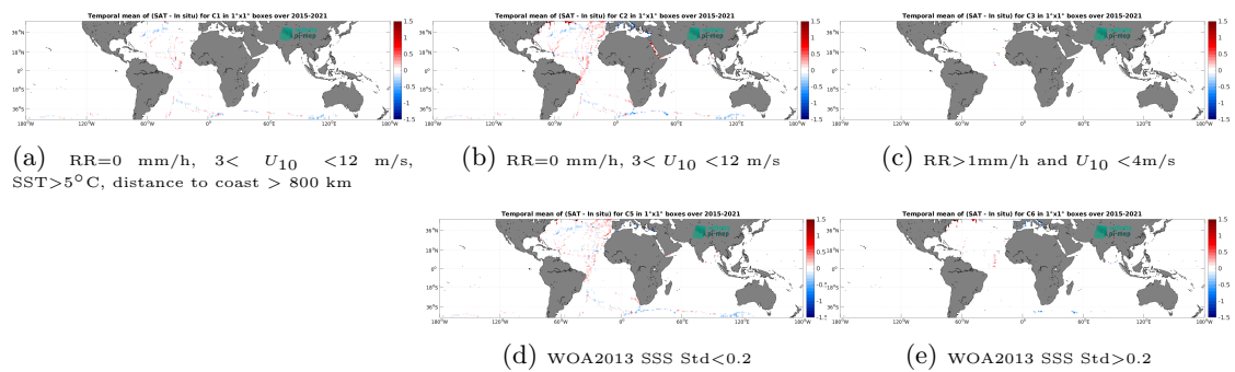
Figure 14: Temporal mean gridded over spatial boxes of size 1^\circ \times 1^\circ of \Delta SSS (SMAP SSS L3 v5.0 - Monthly (JPL) - TSG (GOSUD-Sailing-ship)) for 5 different subdatasets corresponding to: RR=0 mm/h, 3 < U_{10} < 12 m/s, SST > 5°C, distance to coast > 800 km (a), RR=0 mm/h, 3 < U_{10} < 12 m/s (b), RR > 1mm/h and U_{10} < 4 m/s (c), WOA2013 SSS Std < 0.2 (d), WOA2013 SSS Std > 0.2 (e).
