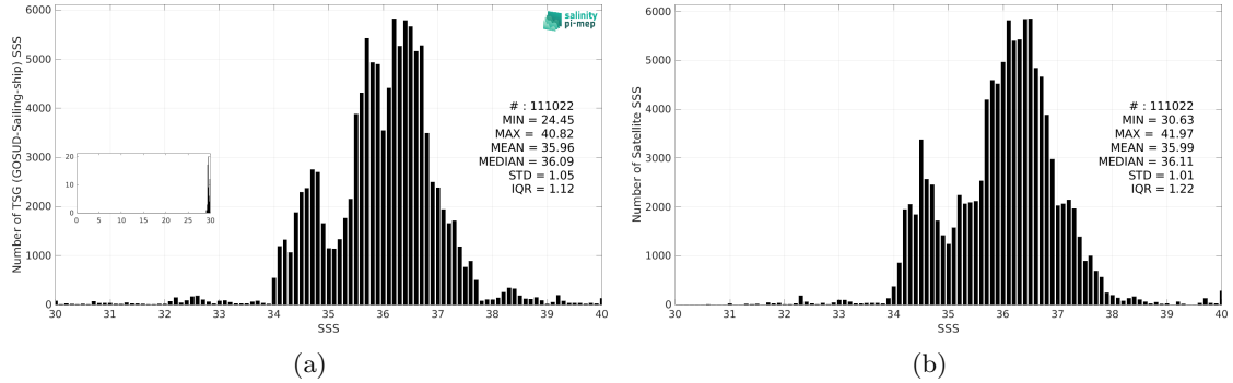
Figure 3: Histograms of SSS from TSG (GOSUD-Sailing-ship) (a) and SMAP SSS L3 v5.0 - Monthly (JPL) (b) considering all match-up pairs per bins of 0.1 over the Mid-Low Latitudes 45N-45S Pi-MEP region and for the full satellite product period.
