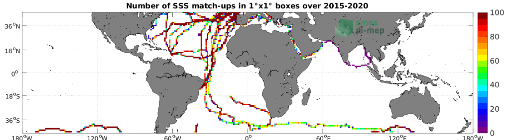
Figure 4: Number of SSS match-ups between TSG (GOSUD-Sailing-ship) SSS and the SMAP SSS L3 v5.0 - Monthly (JPL) SSS product for the Mid-Low Latitudes 45N-45S Pi-MEP region over 1^\circ \times 1^\circ boxes and for the full satellite product period.
