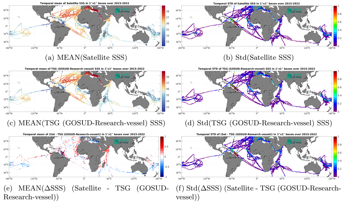
Figure 7: Temporal mean (left) and Std (right) of SSS from SMAP SSS L3 v5.0 - Monthly (JPL) (top), TSG (GOSUD-Research-vessel) (middle), and of \Delta SSS (Satellite - TSG (GOSUD-Research-vessel)). Only match-up pairs are used to generate these maps.
