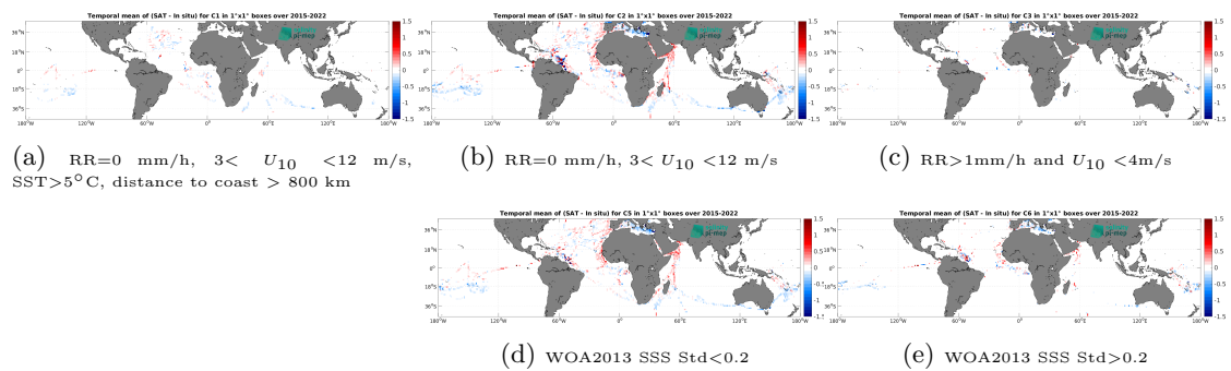
Figure 14: Temporal mean gridded over spatial boxes of size 1^\circ \times 1^\circ of \Delta SSS (SMAP SSS L3 v5.0 - Monthly (JPL) - TSG (GOSUD-Research-vessel)) for 5 different subdatasets corresponding to: RR=0 mm/h, 3 < U_{10} < 12 m/s, SST > 5°C, distance to coast > 800 km (a), RR=0 mm/h, 3 < U_{10} < 12 m/s (b), RR > 1mm/h and U_{10} < 4 m/s (c), WOA2013 SSS Std < 0.2 (d), WOA2013 SSS Std > 0.2 (e).
