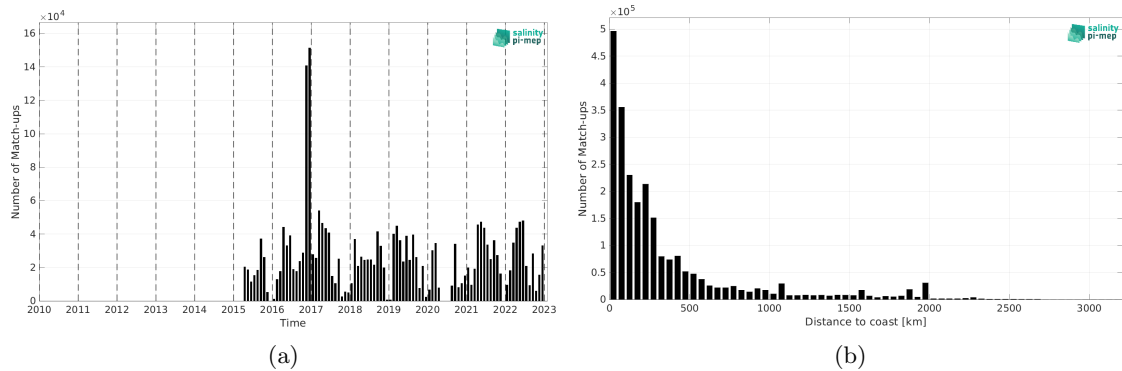
Figure 2: Number of match-ups between TSG (GOSUD-Research-vessel) and SMAP SSS L3 v5.0 - Monthly (JPL) SSS as a function of time (a) and as function of the distance to coast (b) over the Mid-Low Latitudes 45N-45S Pi-MEP region and for the full satellite product period.
