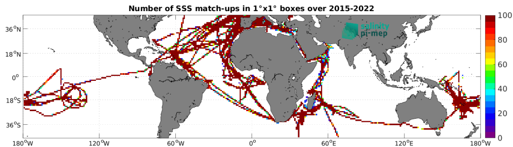
Figure 5: Number of SSS match-ups between TSG (GOSUD-Research-vessel) SSS and the SMAP SSS L3 v5.0 - Monthly (JPL) SSS product for the Mid-Low Latitudes 45N-45S Pi-MEP region over 1^\circ \times 1^\circ boxes and for the full satellite product period.
