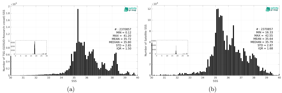
Figure 3: Histograms of SSS from TSG (GOSUD-Research-vessel) (a) and SMAP SSS L3 v5.0 - Monthly (JPL) (b) considering all match-up pairs per bins of 0.1 over the Mid-Low Latitudes 45N-45S Pi-MEP region and for the full satellite product period.
