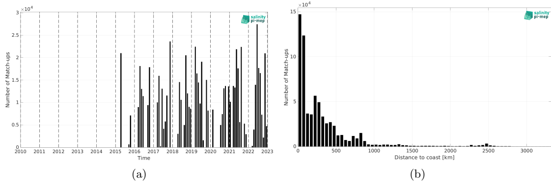
Figure 2: Number of match-ups between TSG (CSIC-UTM) and SMAP SSS L3 v5.0 - Monthly (JPL) SSS as a function of time (a) and as function of the distance to coast (b) over the Mid-Low Latitudes 45N-45S Pi-MEP region and for the full satellite product period.
