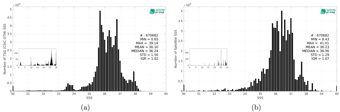
Figure 3: Histograms of SSS from TSG (CSIC-UTM) (a) and SMAP SSS L3 v5.0 - Monthly (JPL) (b) considering all match-up pairs per bins of 0.1 over the Mid-Low Latitudes 45N-45S Pi-MEP region and for the full satellite product period.
