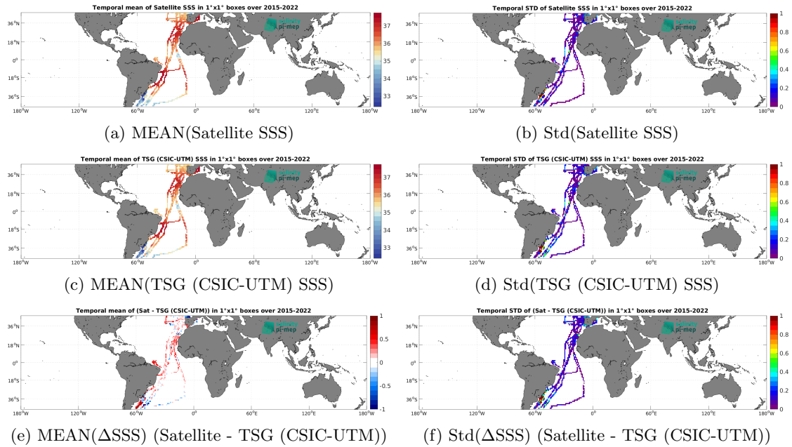
Figure 7: Temporal mean (left) and Std (right) of SSS from SMAP SSS L3 v5.0 - Monthly (JPL) (top), TSG (CSIC-UTM) (middle), and of \Delta SSS (Satellite - TSG (CSIC-UTM)). Only match-up pairs are used to generate these maps.
