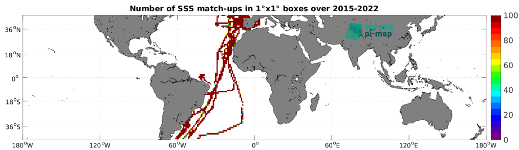
Figure 5: Number of SSS match-ups between TSG (CSIC-UTM) SSS and the SMAP SSS L3 v5.0 - Monthly (JPL) SSS product for the Mid-Low Latitudes 45N-45S Pi-MEP region over 1^\circ \times 1^\circ boxes and for the full satellite product period.
