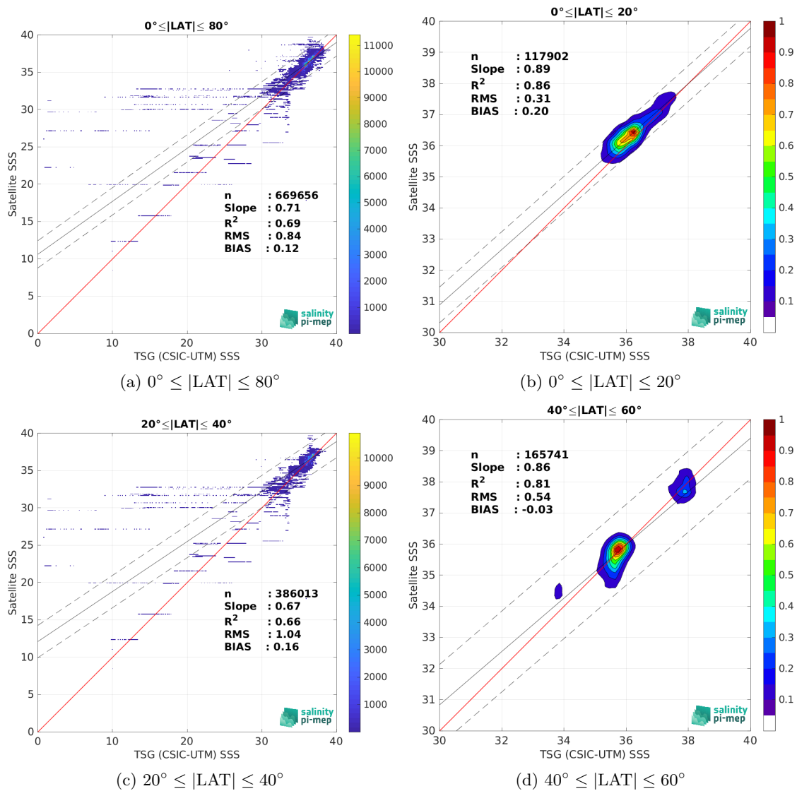
Figure 10: Contour maps of the concentration of SMAP SSS L3 v5.0 - Monthly (JPL) SSS ( y -axis) versus TSG (CSIC-UTM) SSS ( x -axis) at match-up pairs for different latitude bands. For each plot, the red line shows x=y . The black thin and dashed lines indicate a linear fit through the data cloud and the \pm 95\% confidence levels, respectively. The number match-up pairs n , the slope and R^2 coefficient of the linear fit, the root mean square (RMS) and the mean bias between satellite and in situ data are indicated for each latitude band in each plots.
