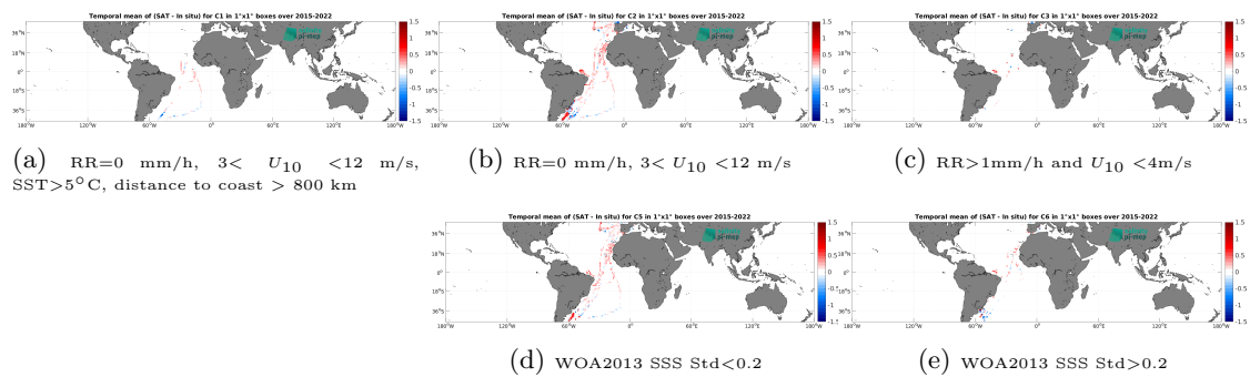
Figure 14: Temporal mean gridded over spatial boxes of size 1^\circ \times 1^\circ of \Delta SSS (SMAP SSS L3 v5.0 - Monthly (JPL) - TSG (CSIC-UTM)) for 5 different subdatasets corresponding to: RR=0 mm/h, 3 < U_{10} < 12 m/s, SST > 5°C, distance to coast > 800 km (a), RR=0 mm/h, 3 < U_{10} < 12 m/s (b), RR > 1mm/h and U_{10} < 4 m/s (c), WOA2013 SSS Std < 0.2 (d), WOA2013 SSS Std > 0.2 (e).
