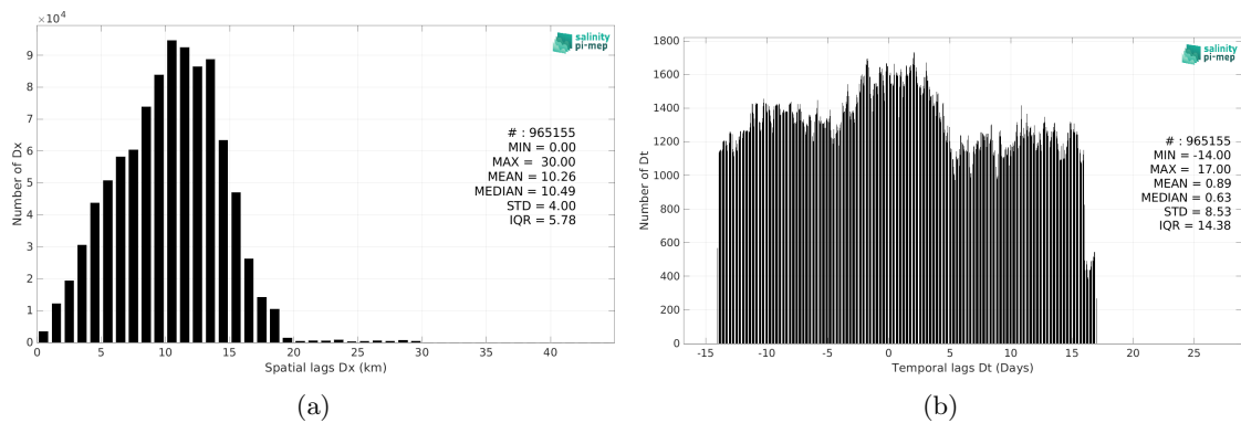
Figure 5: Histograms of the spatial (a) and temporal (b) lags between the location/time of the TSG (CSIC-UTM) measurement and the date of the corresponding SMAP SSS L3 v5.0 - Monthly (JPL) SSS pixel.
