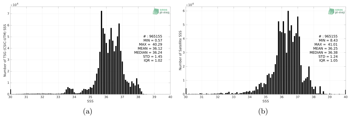
Figure 2: Histograms of SSS from TSG (CSIC-UTM) (a) and SMAP SSS L3 v5.0 - Monthly (JPL) (b) considering all match-up pairs per bins of 0.1 over the Mid-Low Latitudes 45N-45S Pi-MEP region and for the full satellite product period.
