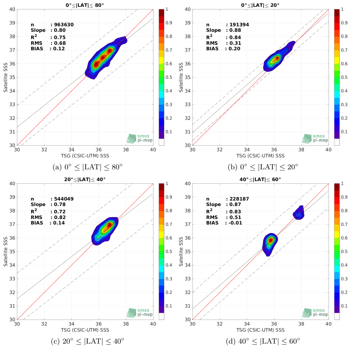
Figure 9: Contour maps of the concentration of SMAP SSS L3 v5.0 - Monthly (JPL) SSS ( y -axis) versus TSG (CSIC-UTM) SSS ( x -axis) at match-up pairs for different latitude bands. For each plot, the red line shows x=y . The black thin and dashed lines indicate a linear fit through the data cloud and the \pm 95\% confidence levels, respectively. The number match-up pairs n , the slope and R^2 coefficient of the linear fit, the root mean square (RMS) and the mean bias between satellite and in situ data are indicated for each latitude band in each plots.
