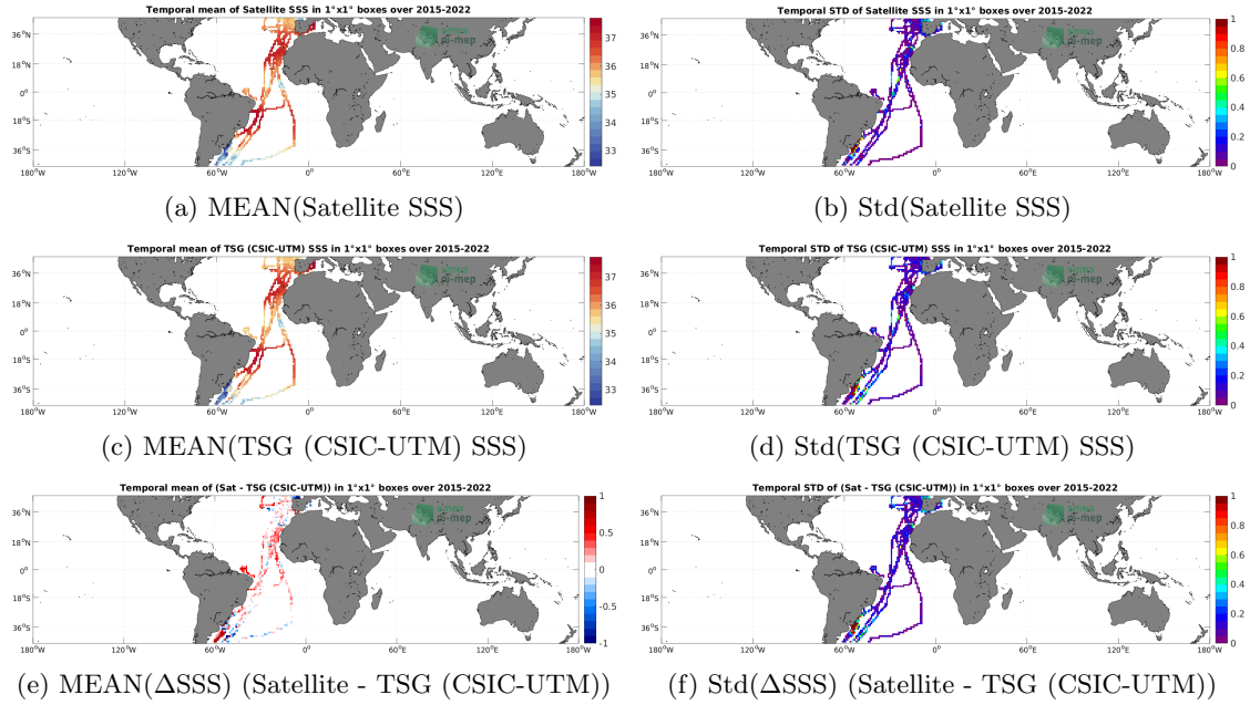
Figure 6: Temporal mean (left) and Std (right) of SSS from SMAP SSS L3 v5.0 - Monthly (JPL) (top), TSG (CSIC-UTM) (middle), and of \Delta SSS (Satellite - TSG (CSIC-UTM)). Only match-up pairs are used to generate these maps.
