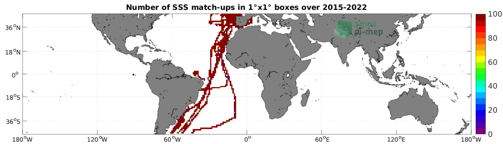
Figure 4: Number of SSS match-ups between TSG (CSIC-UTM) SSS and the SMAP SSS L3 v5.0 - Monthly (JPL) SSS product for the Mid-Low Latitudes 45N-45S Pi-MEP region over 1^\circ \times 1^\circ boxes and for the full satellite product period.
