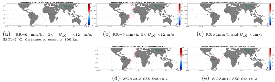
Figure 12: Temporal mean gridded over spatial boxes of size 1^\circ \times 1^\circ of \Delta SSS (SMAP SSS L3 v5.0 - Monthly (JPL) - TSG (CSIC-UTM)) for 5 different subdatasets corresponding to:RR=0 mm/h, 3 < U_{10} < 12 m/s, SST > 5^\circ C , distance to coast > 800 km (a), RR=0 mm/h, 3 < U_{10} < 12 m/s (b), RR > 1 mm/h and U_{10} < 4 m/s (c), WOA2013 SSS Std < 0.2 (d), WOA2013 SSS Std > 0.2 (e).
