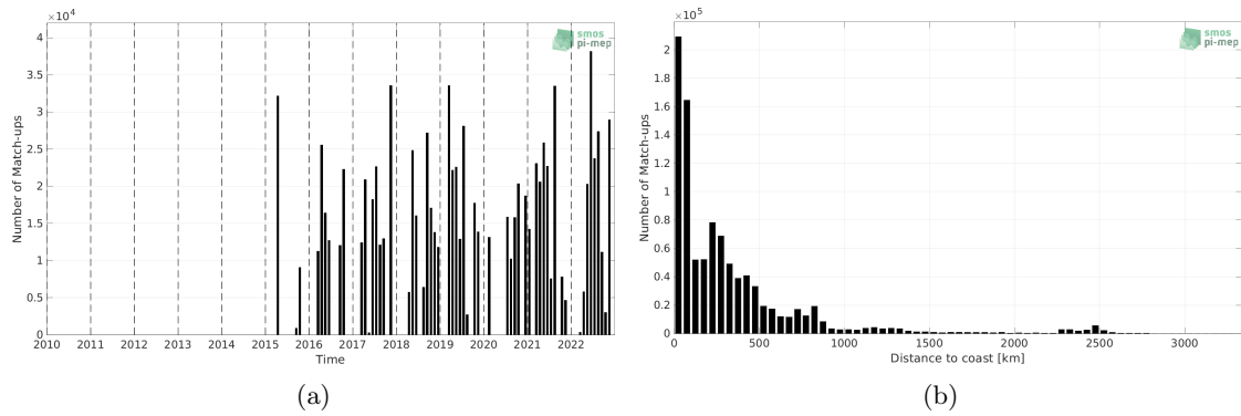
Figure 1: Number of match-ups between TSG (CSIC-UTM) and SMAP SSS L3 v5.0 - Monthly (JPL) SSS as a function of time (a) and as function of the distance to coast (b) over the Mid-Low Latitudes 45N-45S Pi-MEP region and for the full satellite product period.
