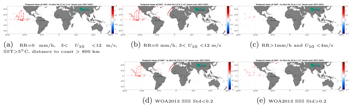
Figure 14: Temporal mean gridded over spatial boxes of size 1^\circ \times 1^\circ of \Delta SSS (SMAP SSS L3 v5.0 - Monthly (JPL) - Sairdrone) for 5 different subdatasets corresponding to: RR=0 mm/h, 3 < U_{10} < 12 m/s, SST > 5°C, distance to coast > 800 km (a), RR=0 mm/h, 3 < U_{10} < 12 m/s (b), RR > 1mm/h and U_{10} < 4 m/s (c), WOA2013 SSS Std < 0.2 (d), WOA2013 SSS Std > 0.2 (e).
