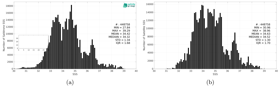
Figure 3: Histograms of SSS from Saildrone (a) and SMAP SSS L3 v5.0 - Monthly (JPL) (b) considering all match-up pairs per bins of 0.1 over the Mid-Low Latitudes 45N-45S Pi-MEP region and for the full satellite product period.
