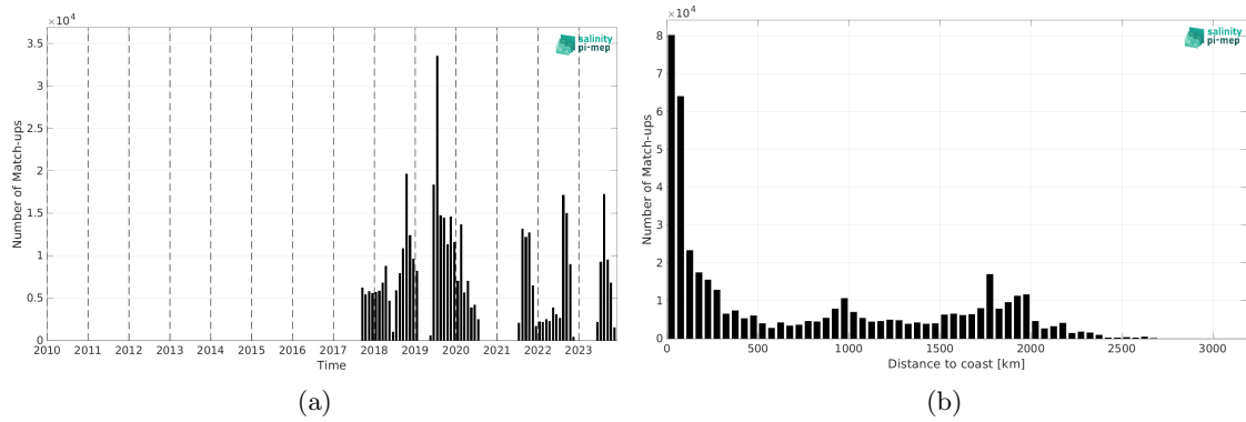
Figure 2: Number of match-ups between Saildrone and SMAP SSS L3 v5.0 - Monthly (JPL) SSS as a function of time (a) and as function of the distance to coast (b) over the Mid-Low Latitudes 45N-45S Pi-MEP region and for the full satellite product period.
