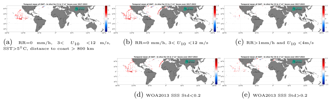
Figure 14: Temporal mean gridded over spatial boxes of size 1^\circ \times 1^\circ of \Delta\text{SSS} (SMAP SSS L3 v5.0 - Monthly (JPL) - Sairdrone) for 5 different subdatasets corresponding to:RR=0 mm/h, 3 < U_{10} < 12 m/s, SST>5°C, distance to coast > 800 km (a), RR=0 mm/h, 3 < U_{10} < 12 m/s (b), RR>1mm/h and U_{10} < 4 m/s (c), WOA2013 SSS Std<0.2 (d), WOA2013 SSS Std>0.2 (e).
