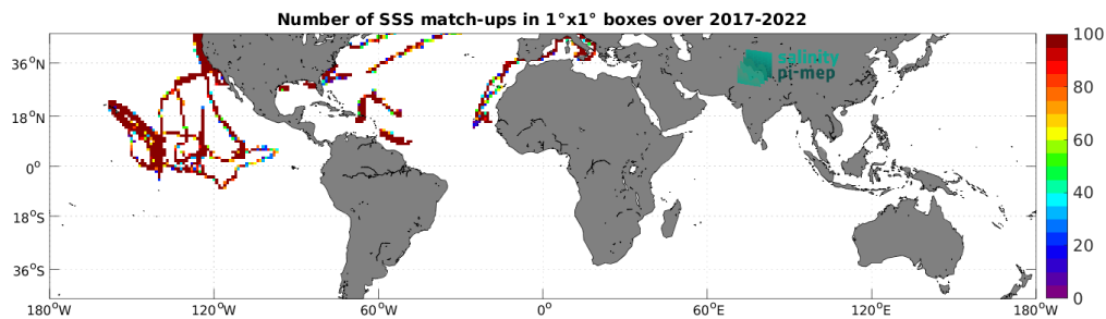
Figure 5: Number of SSS match-ups between Saildrone SSS and the SMAP SSS L3 v5.0 - Monthly (JPL) SSS product for the Mid-Low Latitudes 45N-45S Pi-MEP region over 1^\circ \times 1^\circ boxes and for the full satellite product period.
