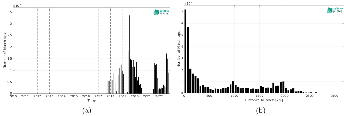
Figure 2: Number of match-ups between Sairdrone and SMAP SSS L3 v5.0 - Monthly (JPL) SSS as a function of time (a) and as function of the distance to coast (b) over the Mid-Low Latitudes 45N-45S Pi-MEP region and for the full satellite product period.
