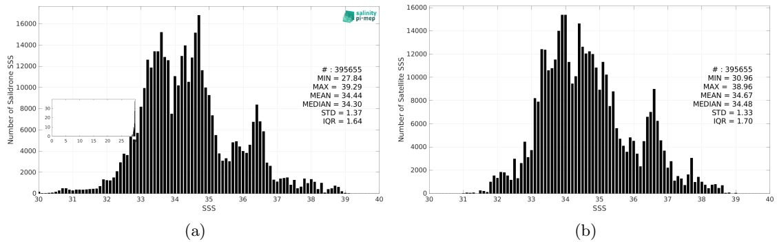
Figure 3: Histograms of SSS from Sairdrone (a) and SMAP SSS L3 v5.0 - Monthly (JPL) (b) considering all match-up pairs per bins of 0.1 over the Mid-Low Latitudes 45N-45S Pi-MEP region and for the full satellite product period.
