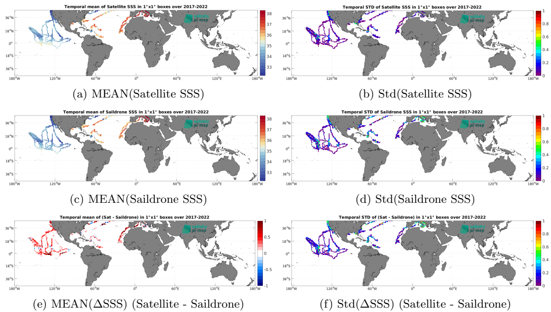
Figure 7: Temporal mean (left) and Std (right) of SSS from SMAP SSS L3 v5.0 - Monthly (JPL) (top), Saildrone (middle), and of \Delta SSS (Satellite - Saildrone). Only match-up pairs are used to generate these maps.
