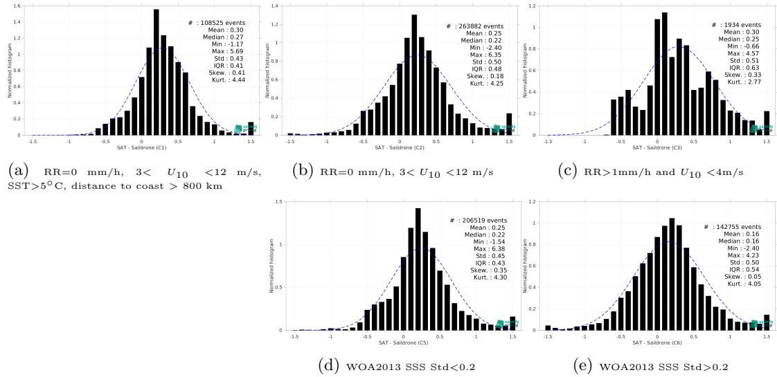
Figure 15: Normalized histogram of \Delta\text{SSS} (SMAP SSS L3 v5.0 - Monthly (JPL) - Saildrone) for 5 different subdatasets corresponding to: RR=0 mm/h, 3 < U_{10} < 12 m/s, SST>5°C, distance to coast > 800 km (a), RR=0 mm/h, 3 < U_{10} < 12 m/s (b), RR>1mm/h and U_{10} < 4 m/s (c), WOA2013 SSS Std<0.2 (d), WOA2013 SSS Std>0.2 (e).
