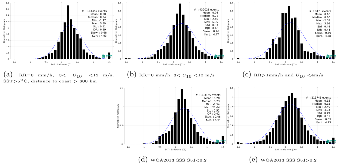
Figure 13: Normalized histogram of \Delta SSS (SMAP SSS L3 v5.0 - Monthly (JPL) - Saildrone) for 5 different subdatasets corresponding to: RR=0 mm/h, 3 < U_{10} < 12 m/s, SST >5^\circ\text{C} , distance to coast > 800 km (a), RR=0 mm/h, 3 < U_{10} < 12 m/s (b), RR >1 mm/h and U_{10} < 4 m/s (c), WOA2013 SSS Std <0.2 (d), WOA2013 SSS Std >0.2 (e).
