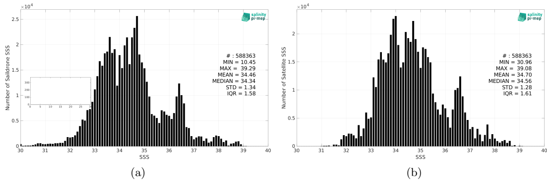
Figure 2: Histograms of SSS from Sairdrone (a) and SMAP SSS L3 v5.0 - Monthly (JPL) (b) considering all match-up pairs per bins of 0.1 over the Mid-Low Latitudes 45N-45S Pi-MEP region and for the full satellite product period.
