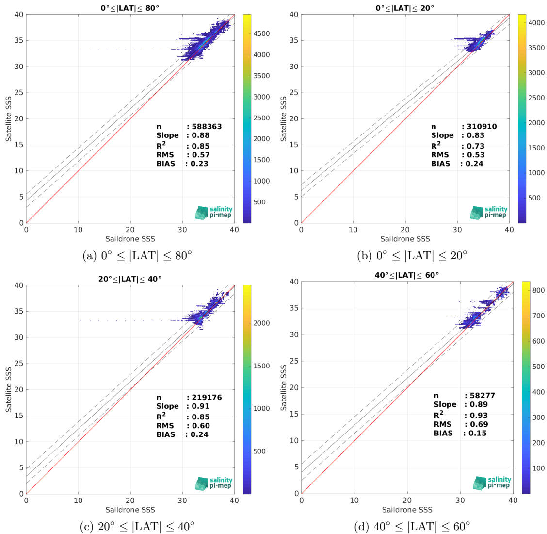
Figure 9: Contour maps of the concentration of SMAP SSS L3 v5.0 - Monthly (JPL) SSS (y-axis) versus Saildrone SSS (x-axis) at match-up pairs for different latitude bands. For each plot, the red line shows x=y . The black thin and dashed lines indicate a linear fit through the data cloud and the \pm 95\% confidence levels, respectively. The number match-up pairs n , the slope and R^2 coefficient of the linear fit, the root mean square (RMS) and the mean bias between satellite and in situ data are indicated for each latitude band in each plots.
