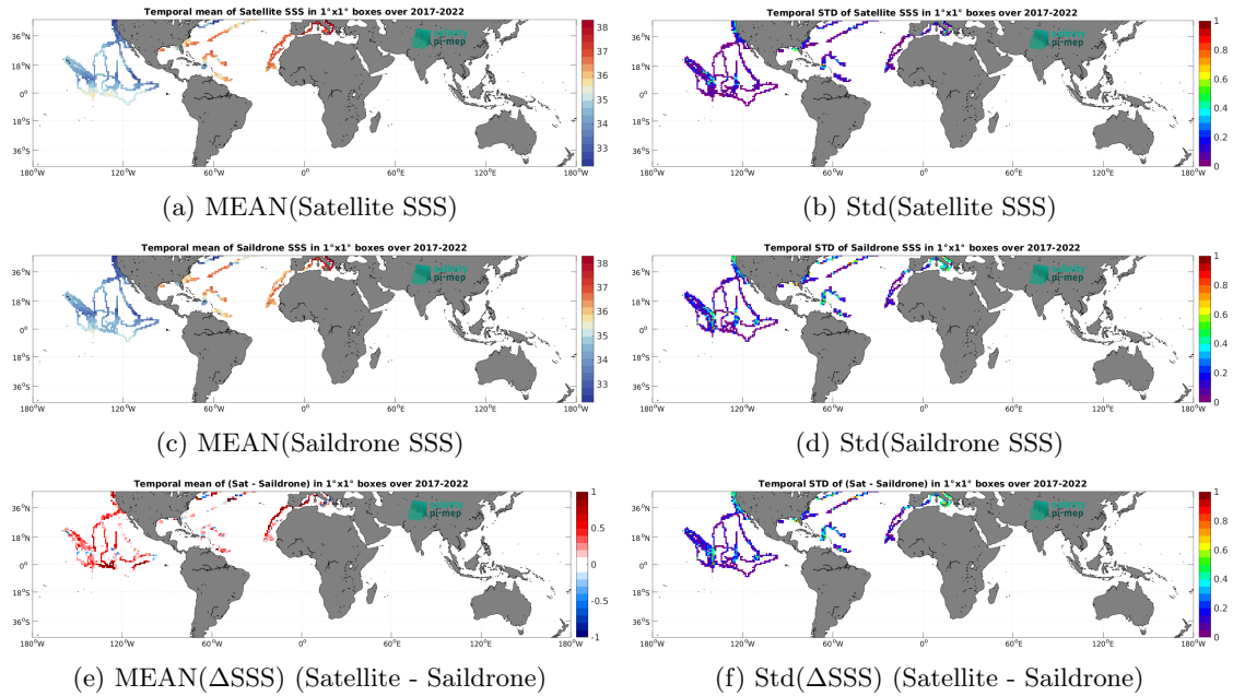
Figure 6: Temporal mean (left) and Std (right) of SSS from SMAP SSS L3 v5.0 - Monthly (JPL) (top), Saildrone (middle), and of \Delta SSS (Satellite - Saildrone). Only match-up pairs are used to generate these maps.
