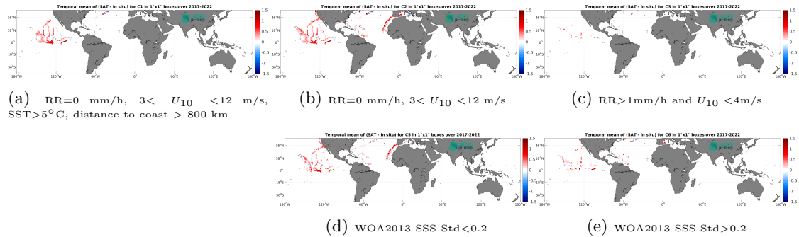
Figure 12: Temporal mean gridded over spatial boxes of size 1^\circ \times 1^\circ of \Delta SSS (SMAP SSS L3 v5.0 - Monthly (JPL) - Saildrone) for 5 different subdatasets corresponding to:RR=0 mm/h, 3 < U_{10} < 12 m/s, SST >5^\circ\text{C} , distance to coast > 800 km (a), RR=0 mm/h, 3 < U_{10} < 12 m/s (b), RR >1 mm/h and U_{10} < 4 m/s (c), WOA2013 SSS Std <0.2 (d), WOA2013 SSS Std >0.2 (e).
