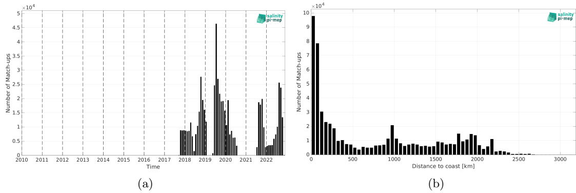
Figure 1: Number of match-ups between Sairdrone and SMAP SSS L3 v5.0 - Monthly (JPL) SSS as a function of time (a) and as function of the distance to coast (b) over the Mid-Low Latitudes 45N-45S Pi-MEP region and for the full satellite product period.
