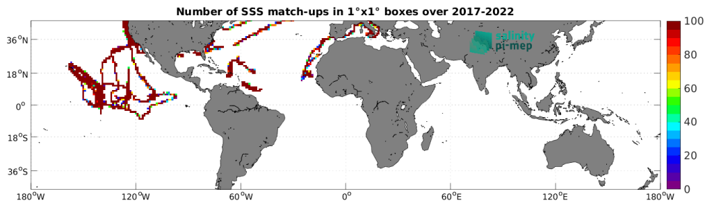
Figure 4: Number of SSS match-ups between Saildrone SSS and the SMAP SSS L3 v5.0 - Monthly (JPL) SSS product for the Mid-Low Latitudes 45N-45S Pi-MEP region over 1^\circ \times 1^\circ boxes and for the full satellite product period.
