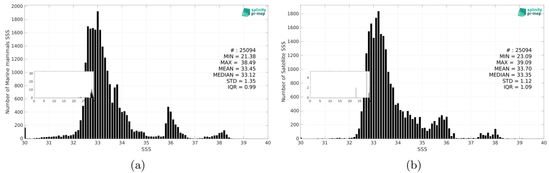
Figure 3: Histograms of SSS from Marine mammals (a) and SMAP SSS L3 v5.0 - Monthly (JPL) (b) considering all match-up pairs per bins of 0.1 over the Mid-Low Latitudes 45N-45S Pi-MEP region and for the full satellite product period.
