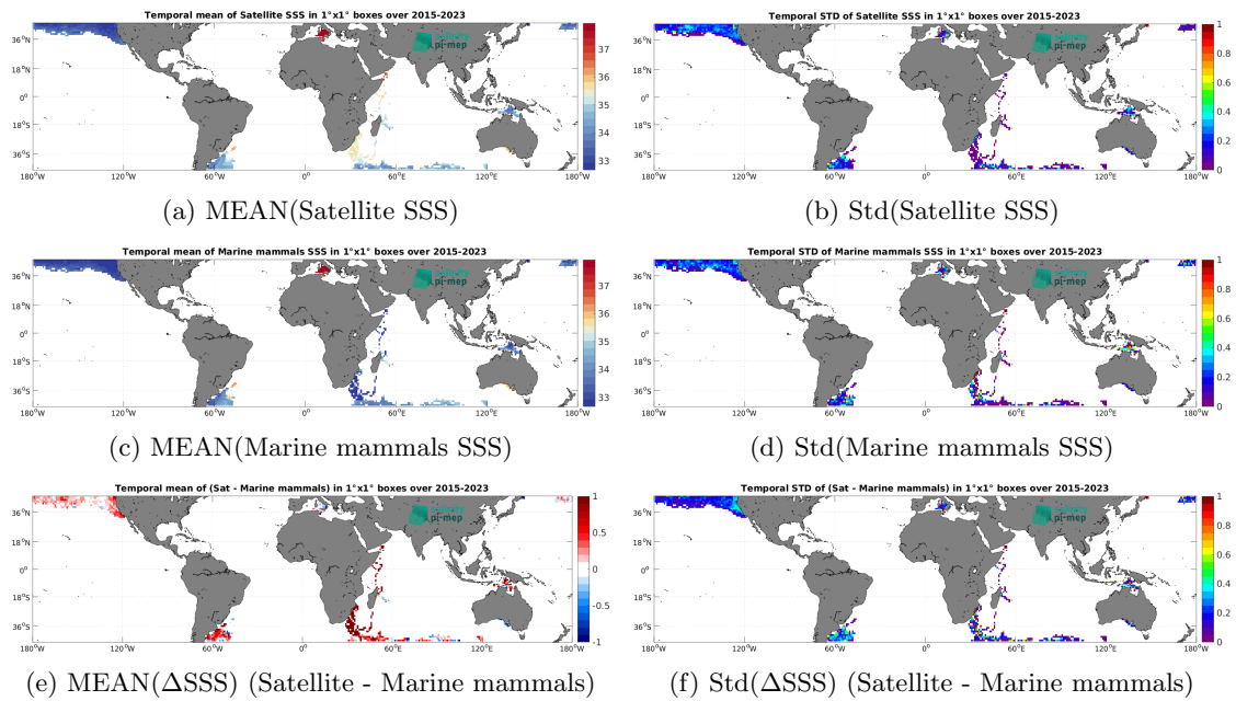
Figure 7: Temporal mean (left) and Std (right) of SSS from SMAP SSS L3 v5.0 - Monthly (JPL) (top), Marine mammals (middle), and of \Delta SSS (Satellite - Marine mammals). Only match-up pairs are used to generate these maps.
