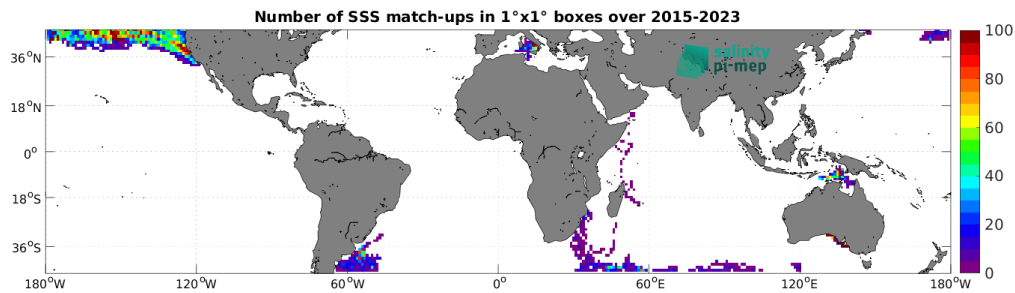
Figure 5: Number of SSS match-ups between Marine mammals SSS and the SMAP SSS L3 v5.0 - Monthly (JPL) SSS product for the Mid-Low Latitudes 45N-45S Pi-MEP region over 1^\circ \times 1^\circ boxes and for the full satellite product period.
