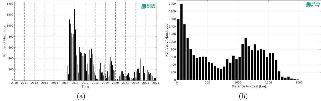
Figure 2: Number of match-ups between Marine mammals and SMAP SSS L3 v5.0 - Monthly (JPL) SSS as a function of time (a) and as function of the distance to coast (b) over the Mid-Low Latitudes 45N-45S Pi-MEP region and for the full satellite product period.
