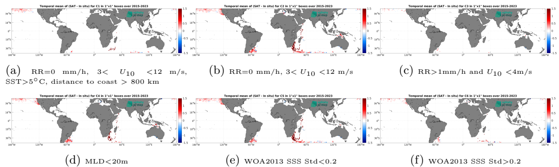
Figure 14: Temporal mean gridded over spatial boxes of size 1^\circ \times 1^\circ of \Delta SSS (SMAP SSS L3 v5.0 - Monthly (JPL) - Marine mammals) for 6 different subdatasets corresponding to:RR=0 mm/h, 3 < U_{10} < 12 m/s, SST>5°C, distance to coast > 800 km (a), RR=0 mm/h, 3 < U_{10} < 12 m/s (b), RR>1mm/h and U_{10} < 4 m/s (c),MLD<20m (d),WOA2013 SSS Std<0.2 (e),WOA2013 SSS Std>0.2 (f).
