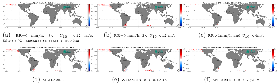
Figure 12: Temporal mean gridded over spatial boxes of size 1^\circ \times 1^\circ of \Delta SSS (SMAP SSS L3 v5.0 - Monthly (JPL) - Marine mammals) for 6 different subdatasets corresponding to:RR=0 mm/h, 3 < U_{10} < 12 m/s, SST >5^\circ C, distance to coast > 800 km (a), RR=0 mm/h, 3 < U_{10} < 12 m/s (b), RR >1 mm/h and U_{10} < 4 m/s (c),MLD <20 m (d),WOA2013 SSS Std <0.2 (e),WOA2013 SSS Std >0.2 (f).
