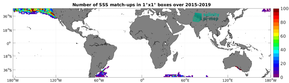
Figure 4: Number of SSS match-ups between Marine mammals SSS and the SMAP SSS L3 v5.0 - Monthly (JPL) SSS product for the Mid-Low Latitudes 45N-45S Pi-MEP region over 1^\circ \times 1^\circ boxes and for the full satellite product period.
