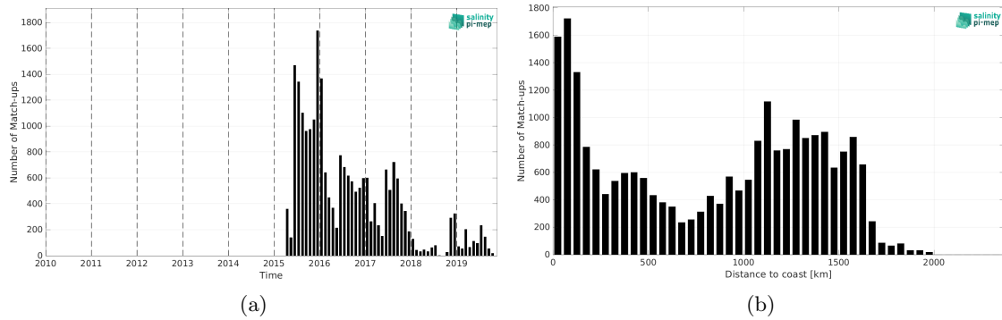
Figure 1: Number of match-ups between Marine mammals and SMAP SSS L3 v5.0 - Monthly (JPL) SSS as a function of time (a) and as function of the distance to coast (b) over the Mid-Low Latitudes 45N-45S Pi-MEP region and for the full satellite product period.
