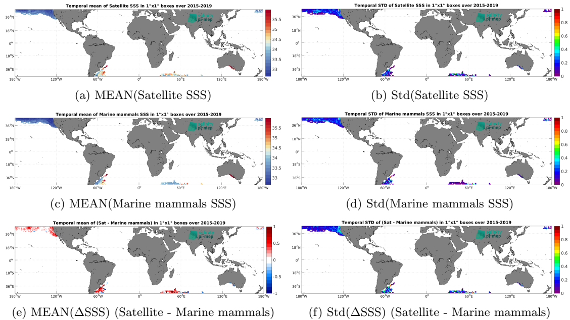
Figure 6: Temporal mean (left) and Std (right) of SSS from SMAP SSS L3 v5.0 - Monthly (JPL) (top), Marine mammals (middle), and of \Delta SSS (Satellite - Marine mammals). Only match-up pairs are used to generate these maps.
