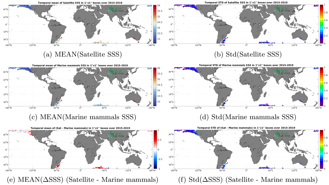
Figure 6: Temporal mean (left) and Std (right) of SSS from SMAP SSS L3 v5.0 - Monthly (JPL) (top), Marine mammals (middle), and of \Delta SSS (Satellite - Marine mammals). Only match-up pairs are used to generate these maps.
