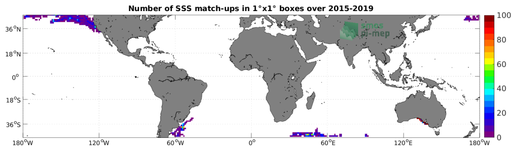
Figure 4: Number of SSS match-ups between Marine mammals SSS and the SMAP SSS L3 v5.0 - Monthly (JPL) SSS product for the Mid-Low Latitudes 45N-45S Pi-MEP region over 1°x1° boxes and for the full satellite product period.
