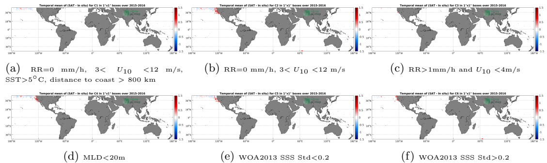
Figure 12: Temporal mean gridded over spatial boxes of size 1°x1° of \Delta SSS (SMAP SSS L3 v5.0 - Monthly (JPL) - Sea mammals) for 6 different subdatasets corresponding to:RR=0 mm/h, 3 < U_{10} < 12 m/s, SST > 5°C, distance to coast > 800 km (a), RR=0 mm/h, 3 < U_{10} < 12 m/s (b), RR > 1mm/h and U_{10} < 4m/s (c),MLD < 20m (d),WOA2013 SSS Std < 0.2 (e),WOA2013 SSS Std > 0.2 (f).
